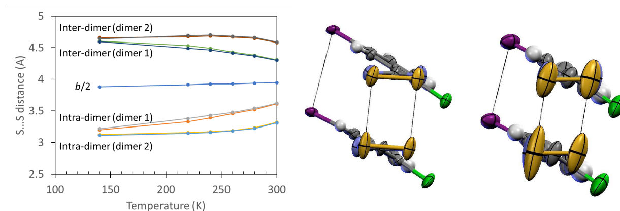
Figure 11. (left) Temperature dependence of the intra-dimer and inter-dimer S...S contacts in 4 in relation to half the crystallographic b -axis ( \pi -stacking direction); thermal ellipsoids are shown (80% probability) for the same crystallographically unique dimer at 140 K (center) and 300 K (right).
