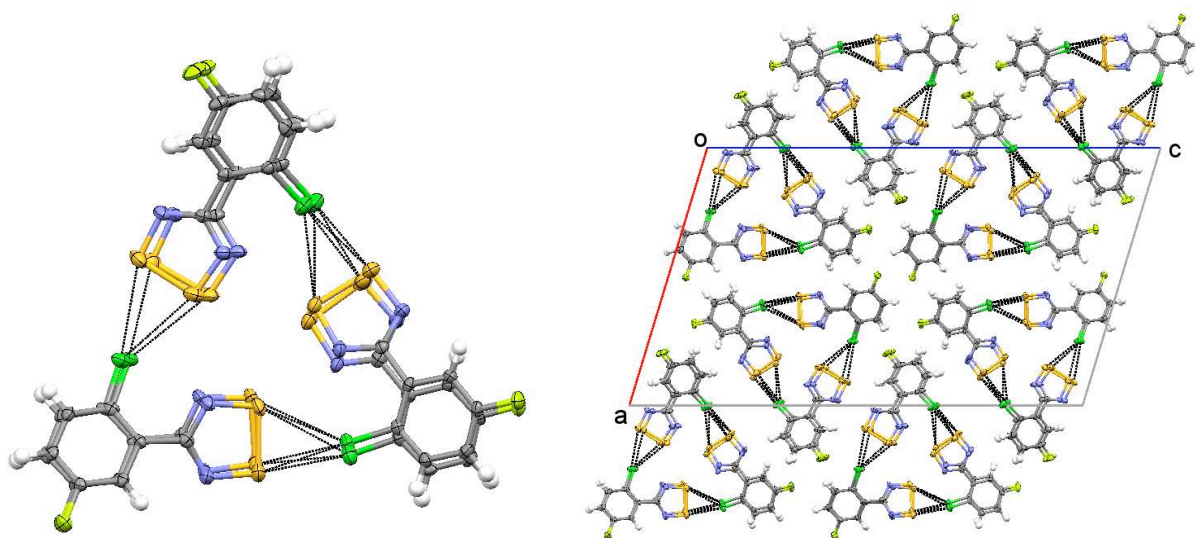
Figure 3. (left) Asymmetric unit of 1 illustrating the structure-directing S...Cl contacts which form supramolecular triangles; (right) packing of triangles in the ac plane.
