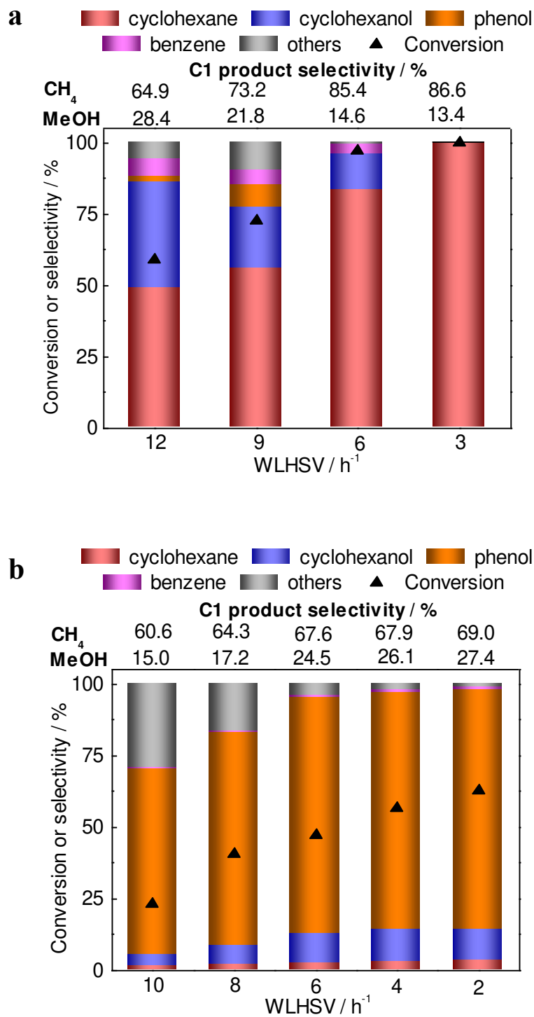
Figure 7 Catalytic performances of catalysts with different WLHSV, P(H 2 )=3.0 MPa, H 2 /GUA molar ratio = 50, T= 573 K, (a) Ni 5 Fe 1 /CNT, (b) Ni 1 Fe 5 /CNT.
