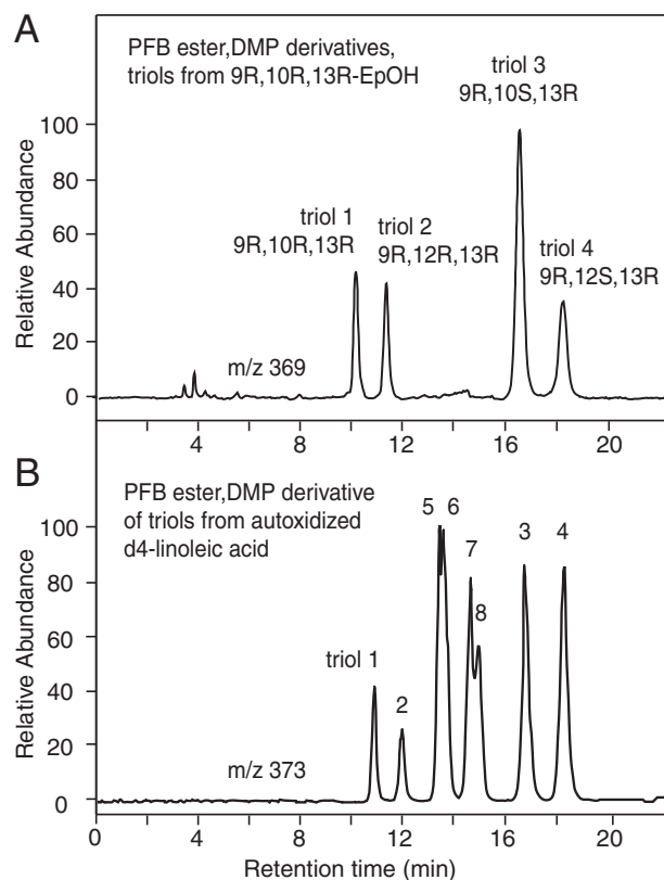
FIGURE 4. LC-MS resolution of linoleate triol standards as the PFB ester DMP derivative. A , four triol hydrolysis products (triol-1 to -4) of 9R,10R-epoxy-13R-hydroxyoctadec-11E-enoic acid are analyzed as the PFB ester DMP derivative using a Thomson Advantage Silica 150Å 5- \mu , column (25 \times 0.46 cm) with a solvent of hexane/IPA 100/1 (by volume) at a flow rate 1 ml/min, with UV detection at 205 nm. B , in autoxidized d4 epoxy alcohol, the same four products were chromatographed with the triols (PFB ester DMP derivative) from the second major epoxy alcohol of the hematin reaction, the 13S diastereomer, 9R,10R-epoxy-13S-hydroxyoctadec-11E-enoate (triol-5 to -8).
