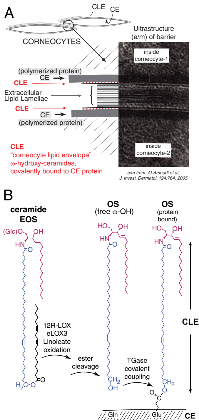
FIGURE 1. Structures of the epidermal water barrier and formation of the CLE. A , electron micrograph of the epidermal barrier with the parts illustrated in schematic style. In the barrier layer of the epidermis the corneocytes are melded together by fusion of three substructures: polymerized protein forming the corneocyte envelope (CE) on the periphery of each cell, extracellular lamellar lipids between cells, and the monolayer of covalently bound ceramides and fatty acids, the CLE, covering the corneocyte envelope and forming a scaffold for the lamellar lipids. B , our working hypothesis (8) entails LOX-catalyzed oxidation of the linoleate in EOS ceramide, facilitating hydrolysis of the ester bond, freeing OS ceramide for coupling to the corneocyte envelope protein by transglutaminase (TGase), thus forming the CLE. The electron micrograph is from Ref. 66 with permission.
