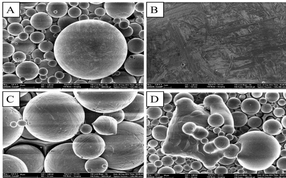
Figure 8 - SEM Images of A. Powder from Fourth Build Showing Large Particle. B. Magnified Image of A Showing Fine Acicular Martensitic alpha structure. C. Powder taken from the chamber after the fifth build D. Powder from Third Build Showing Partial Sintering.
