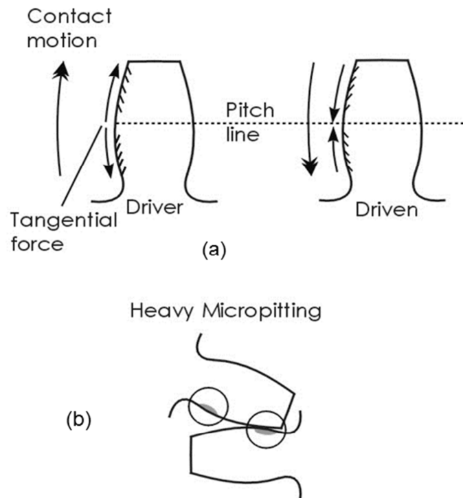
Fig. 3 Illustration of observed direction of growth of micro-cracks on gear teeth
