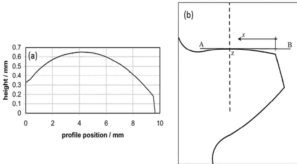
Fig. 4 (a) typical raw profilometer trace of a gear tooth showing the tooth tip location on the right (origin of the x -coordinate) (b) illustration showing the setup for measurement of the tooth profile. Here, AB is the datum line of the profilometer, which is tangential to the tooth at the working pitch point z and x is the distance along the profile measured from the tooth tip.
