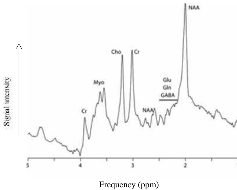
Figure 2.4: A typical MRS spectrum showing the brain metabolites that can be detected and their chemical shift frequencies. Image adapted from (Puts and Edden, 2012).
