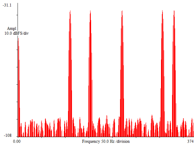
Fig. 12. 10-bit INL and one Q noise DCF.
