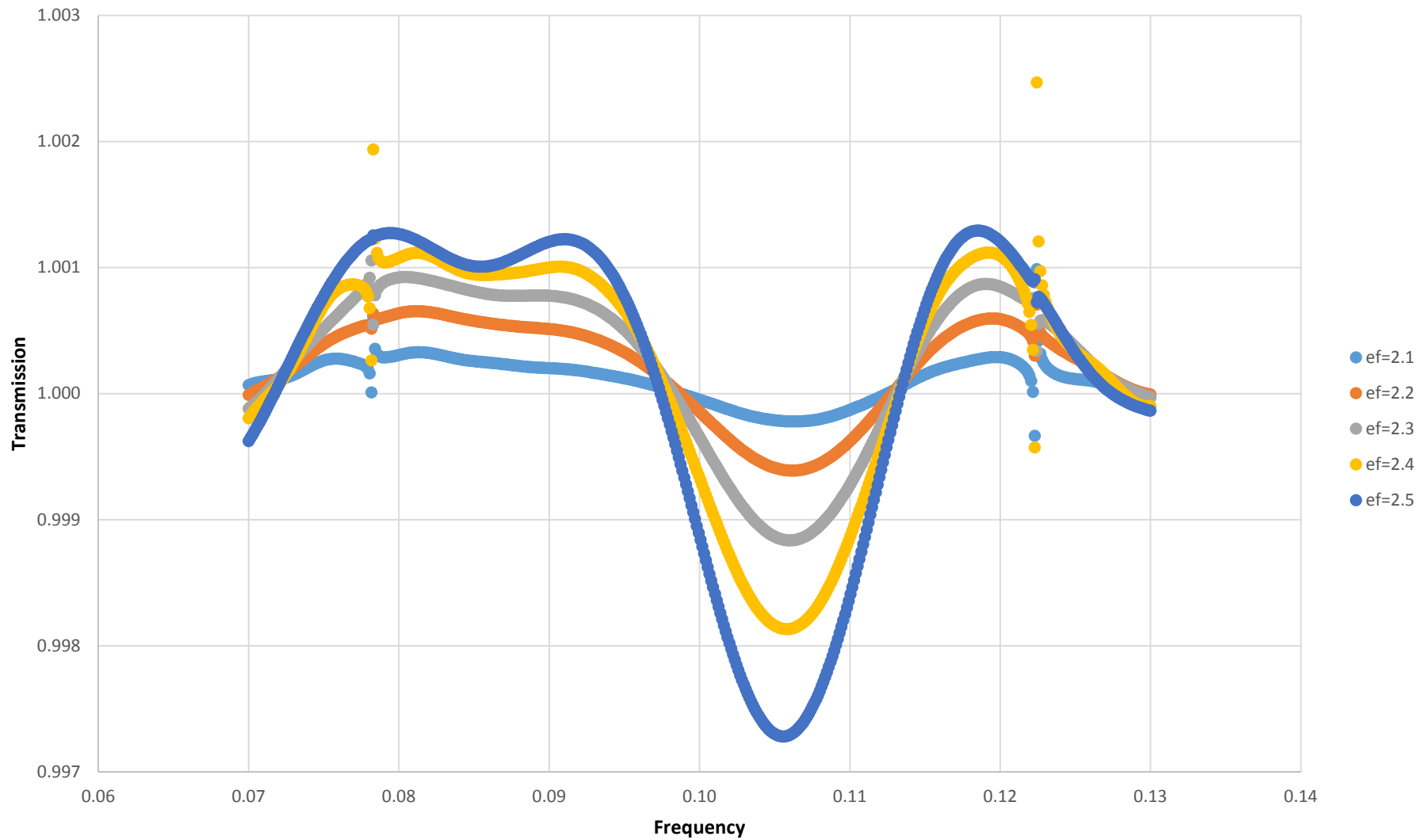
Figure 3.17: Plot showing relative transmission vs frequency for a 40x60 lattice of fibril with epsilon value between 2.1-2.5
