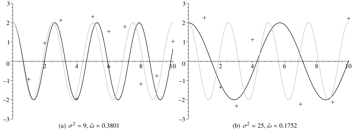
Figure A.6: Plots of Y and the estimated reconstructed signal a^{(0)} \exp(d^{(0)}n) \sin(2\pi\hat{\omega}n + \phi^{(0)}) in black, with true signal a^{(0)} \exp(d^{(0)}n) \sin(2\pi\omega n + \phi^{(0)}) in grey, corresponding to the estimated global minimizer shown in Fig. A.5.
