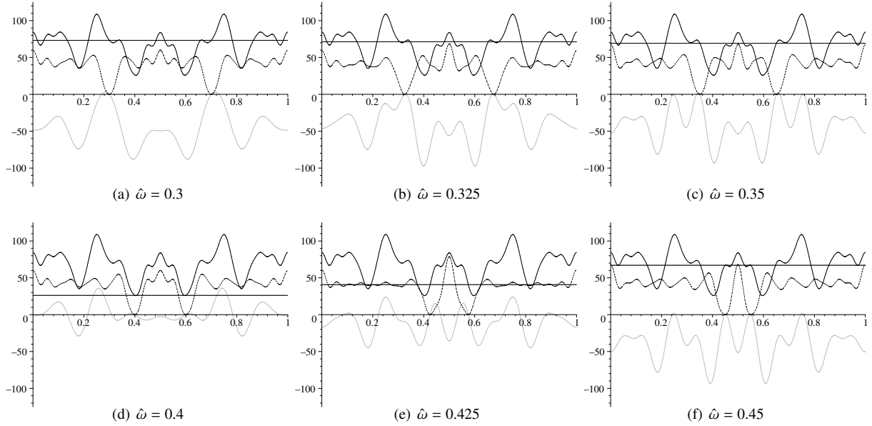
Figure A.6: Plots of Y and the estimated reconstructed signal a^{(0)} \exp(d^{(0)}n) \sin(2\pi\hat{\omega}n + \phi^{(0)}) in black, with true signal a^{(0)} \exp(d^{(0)}n) \sin(2\pi\omega n + \phi^{(0)}) in grey, corresponding to the estimated global minimizer shown in Fig. A.5.
