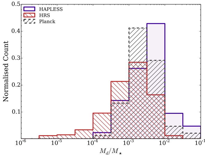
FIGURE 6.3 The distributions of M_d/M_* (ie, specific dust mass) for the HAPLESS, HRS, and Planck C13N13 galaxies. HAPLESS contains a much higher proportion of very dust-rich galaxies than either of the other two samples.
