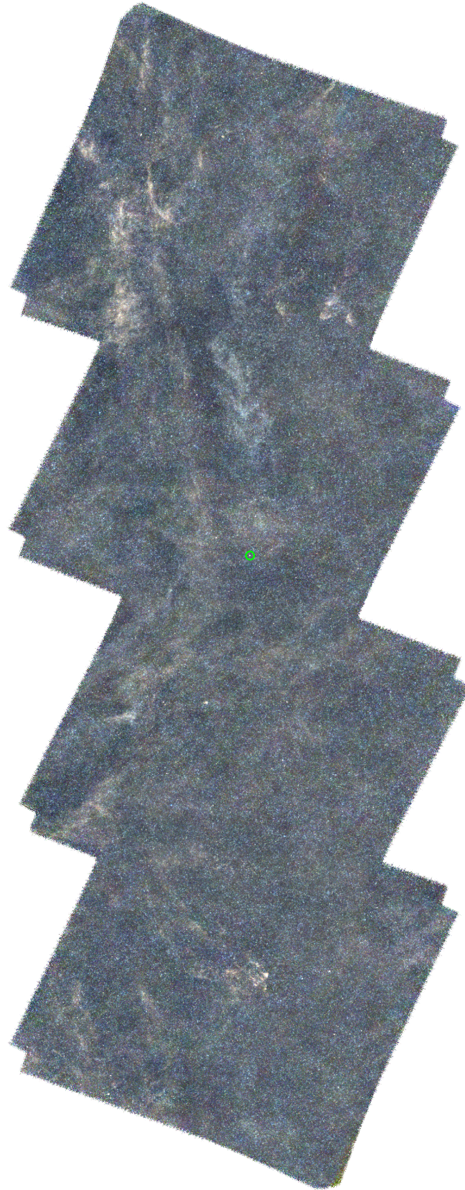
FIGURE 3.5 Three-colour SPIRE (250, 250, and 500 \mu\text{m} ) images of the H-ATLAS GAMMA fields, with the locations of the HAPLESS galaxies indicated by the green circles. This Page: The H-ATLAS GAMMA09 field.
