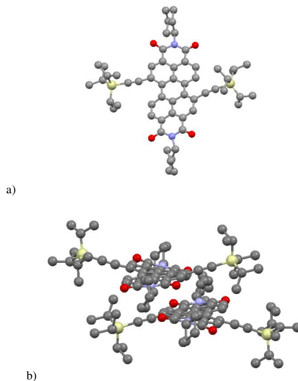
Figure 1 Views of a) the single crystal structure of N,N' -di-(cyclohexyl)-1,7-di-(tri-isopropyl-silylethynyl)-PDI, note the 1,7-isomeric arrangement; b) pairs of \pi - \pi stacked M and P isomers of N,N' -di-(cyclohexyl)-1,7-di-(tri-isopropyl-silylethynyl)-PDI. Carbon - grey, nitrogen - blue, oxygen - red, silicon - yellow. Hydrogen atoms are omitted for clarity.
