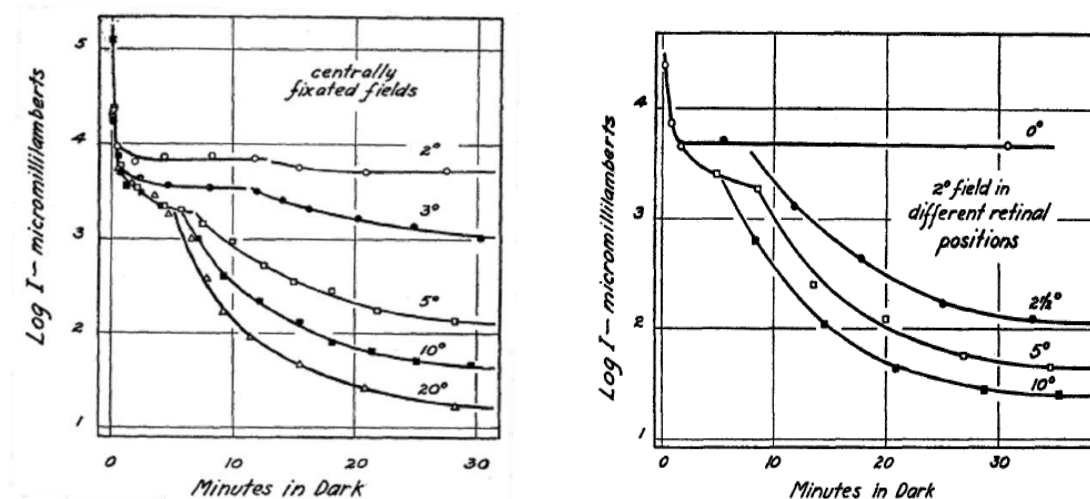
Figure 20. Dark adaptation thresholds measured with centrally fixated stimuli of different size (left panel) and with a 2° stimulus placed at different distances from fixation (right panel) (Hecht et al. 1937).
