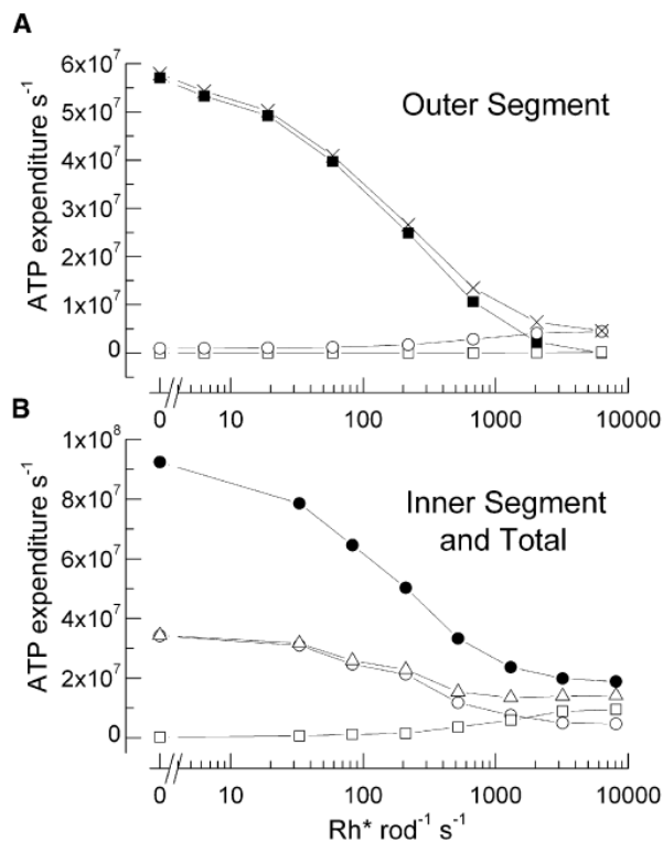
Figure 14. Main contributors to ATP consumption in mammalian rods over the physiological range of steady light intensities. (A) Outer segment. ATP required for extrusion of \text{Na}^+ entering cGMP-gated channels (filled square), transducin GTP hydrolysis and rhodopsin phosphorylation (open square), cGMP synthesis (open circle), and sum of these processes (X). (B) Inner segment and total rod ATP consumption. ATP required for extrusion of \text{Na}^+ entering through i_h channels (open square), extrusion of \text{Ca}^{2+} entering voltage-gated channels at synaptic terminal (open circle), sum of ATP for \text{Na}^+ and \text{Ca}^{2+} extrusion (open triangle), and sum of ATP turnover in whole rod (closed circle) (Okawa et al. 2008).
