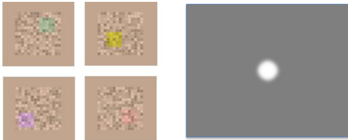
Figure 41. Images showing the appearance of the moving coloured stimulus (Barbur et al. 2006) (left panel) and flickering stimulus (right panel) used during the test.
