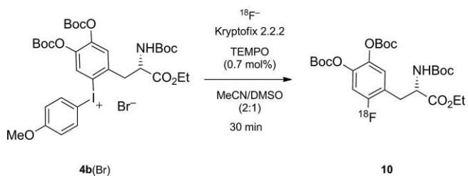
Scheme 2. Synthesis of hot [ 18 F]F-DOPA.
