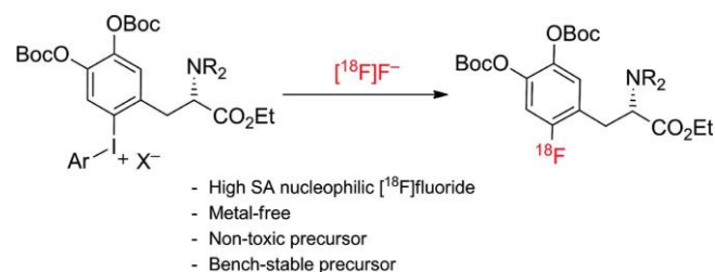
Scheme 1. Synthesis of [ 18 F]F-DOPA.
