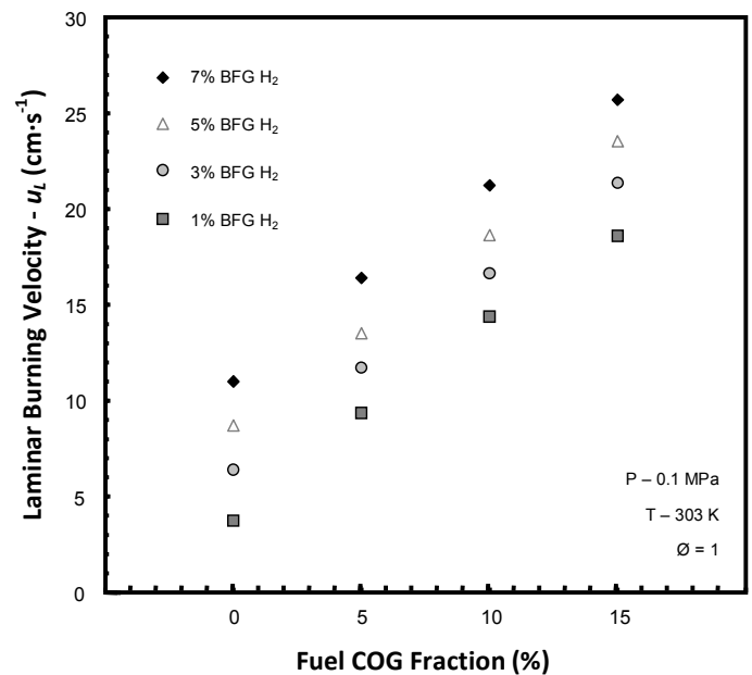
Figure 4.8 u_L plotted against COG fraction for combustion of stoichiometric COG/BFG blends
