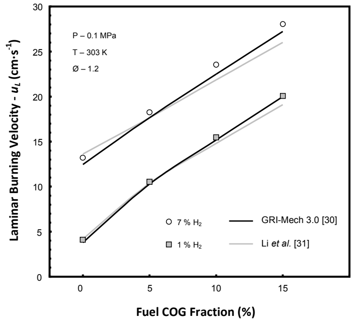
Figure 4.10 Performance of models for COG/BFG blends
