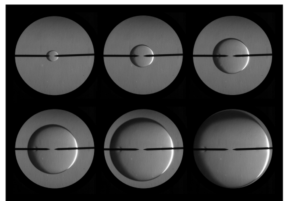
Figure 2.2 Examples of images obtained from the Schlieren optical system
