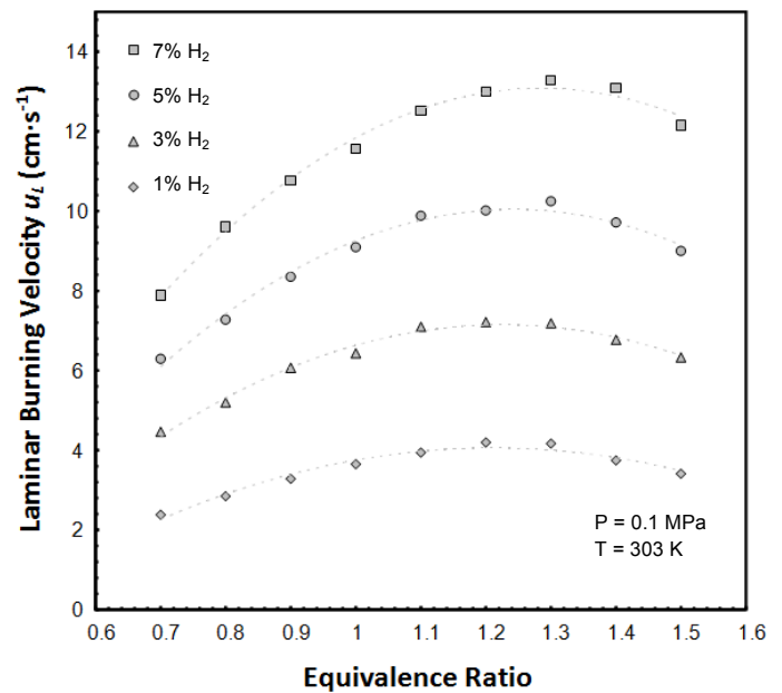
Figure 1.1 laminar burning velocities of different BFG compositions [9]
