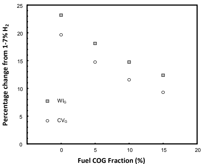
Figure 4.12 Percentage change in CV_G and WI_G for 1-7 % H_2
