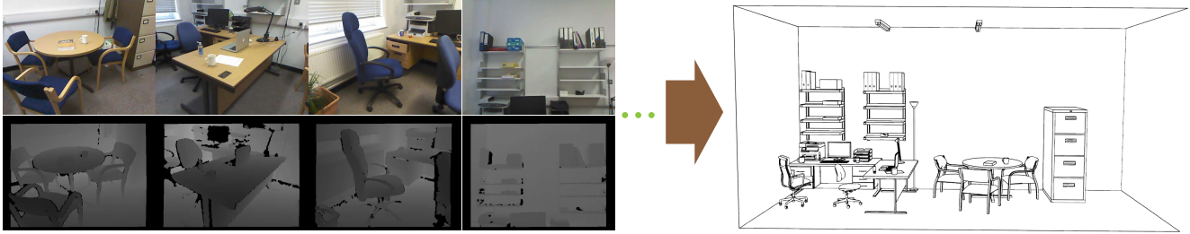
Figure 1: Automatic semantic modeling of an office scene. Left: input RGB-D images, right: reconstructed 3D scene.
