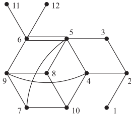
Figure 43: Graph \mathcal{E}_{12}^{\rho_1}(Sp(2))
