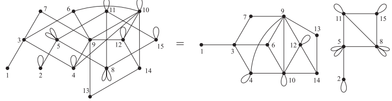
Figure 41: Graph \mathcal{E}_8^{\rho_2}(Sp(2))
