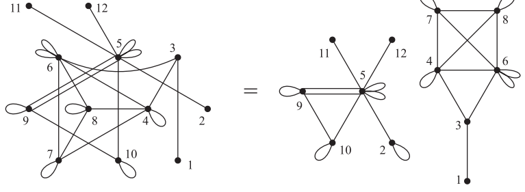
Figure 44: Graph \mathcal{E}_{12}^{\rho_2}(Sp(2))
