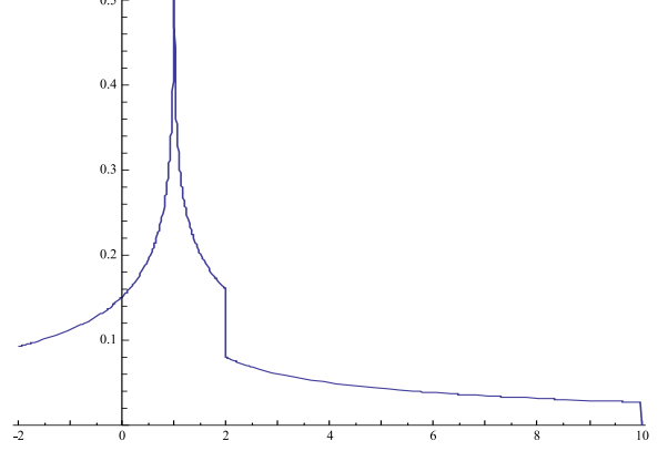
Figure 10: J_z^{\mathbb{T}^2}(z)
