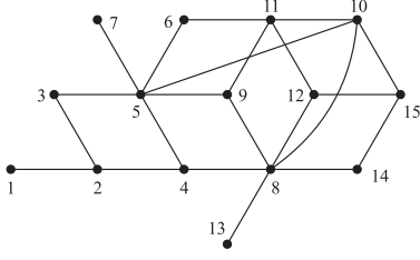
Figure 40: Graph \mathcal{E}_8^{\rho_1}(Sp(2))
