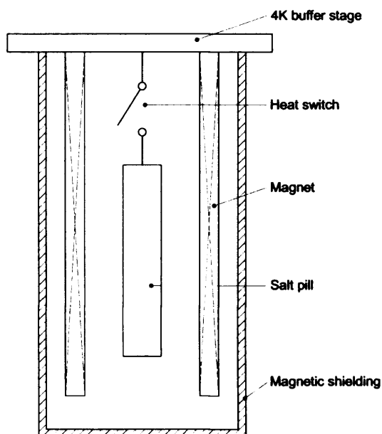
Figure 1.12: Principle schematic of a single-shot ADR using only one salt pill.
