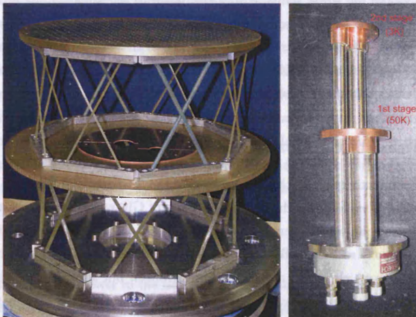
Figure 2.2: Left picture shows the 3 K base plate (top), the 50 K base plate (middle) and the vacuum shield (bottom) together with the G10 support structures. The right picture shows the PTC with its first and second stage cold heads.
