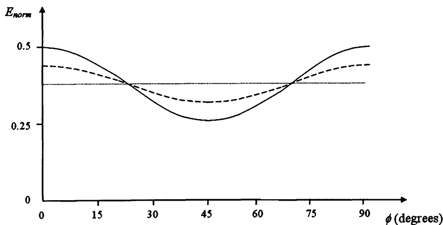
Fig. 3. Variation of normalised elastic modulus, E_{norm} , with angle, \phi , for three theoretical collagenous lamellar structures: (1) A laminate in which the lamellae are arranged isotropically about \phi (dotted line); (2) A laminate in which half the lamellae lie perfectly oriented at \phi = 0^\circ and the remaining half lie orthogonally at \phi = 90^\circ (continuous line); (3) An idealised human corneal stroma in which two identical Gaussian distributions of lamellae are spread about orthogonal preferred meridians at \phi = 0^\circ/90^\circ (dashed line).
