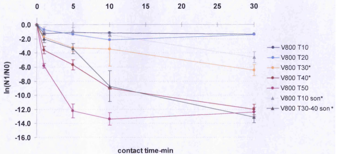
Figure 5-9. The efficacy of VANTOCIL™ TG at 800 ppm against MS2 established by suspension test.
