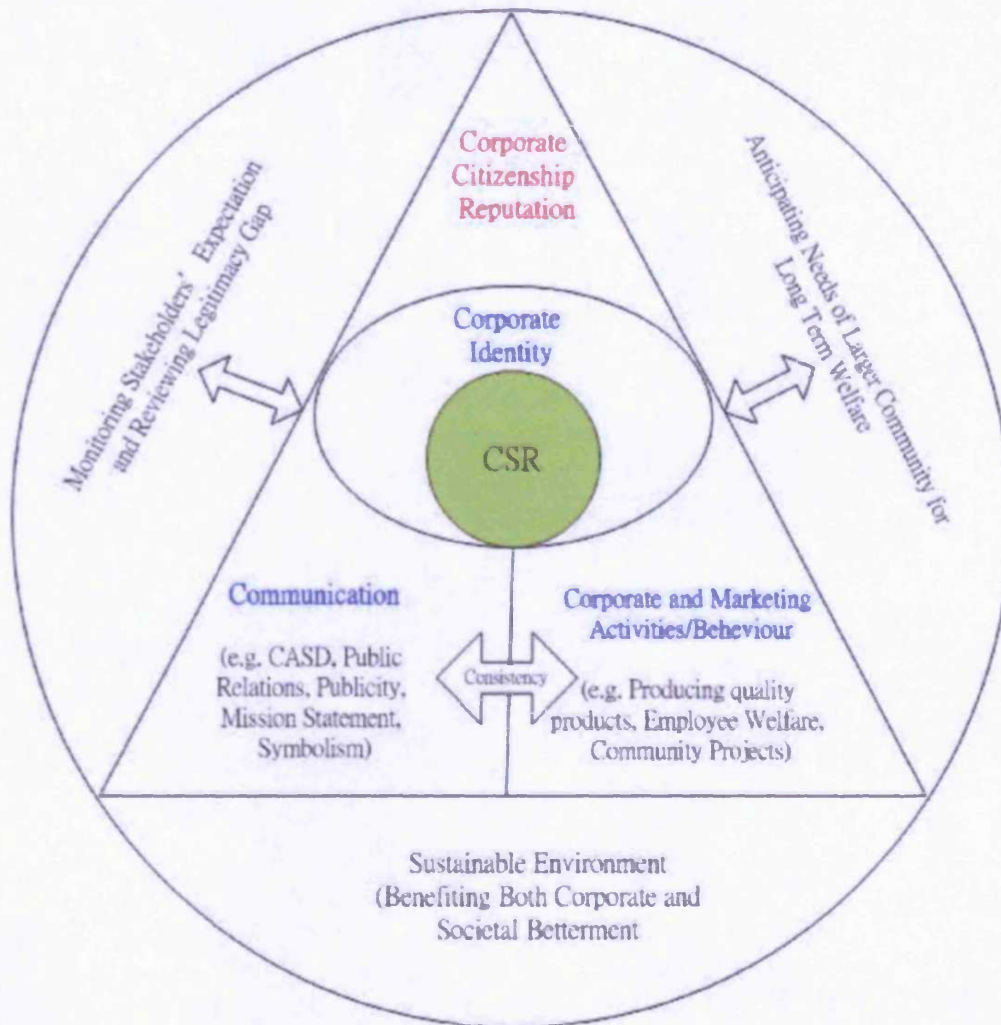
Figure 2.4: Conceptual Model
