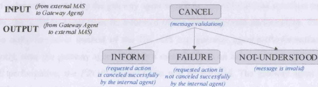
Figure 5.6. FIPA Cancel interaction protocol
