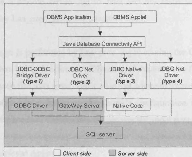
Figure 7.4. JDBC methodologies[20]
