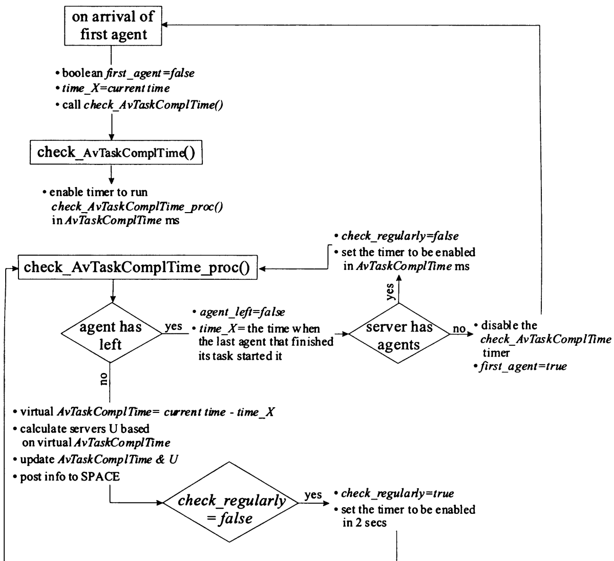
Figure 6.9. Adaptability algorithm of SARA LB model
