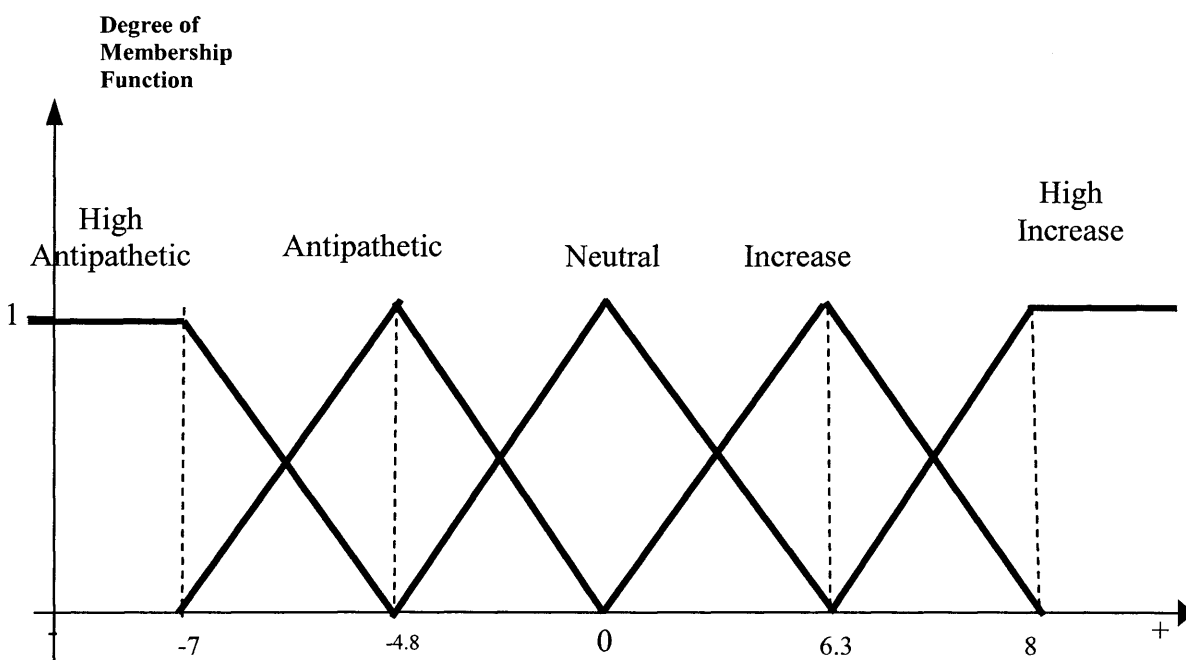
Figure 4.10 Membership functions for \Delta A_7
