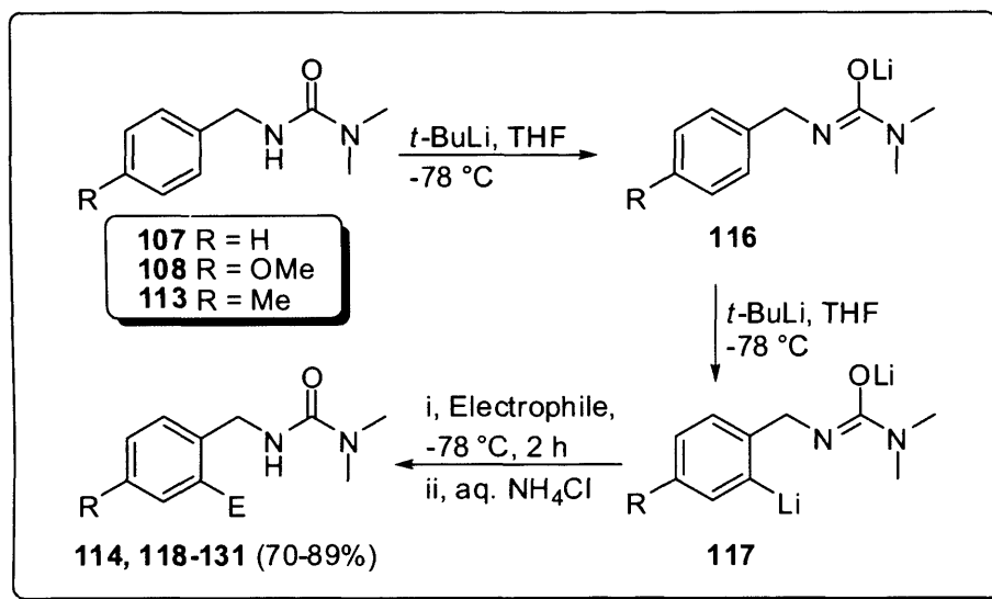
Scheme 3.5
