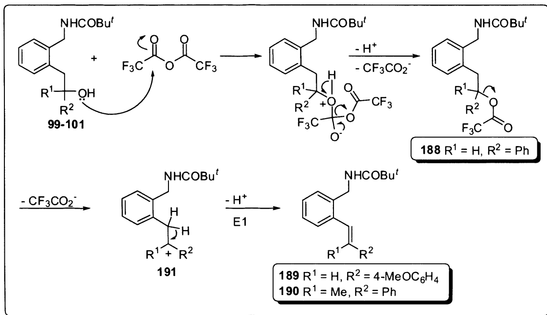
Scheme 5.6
