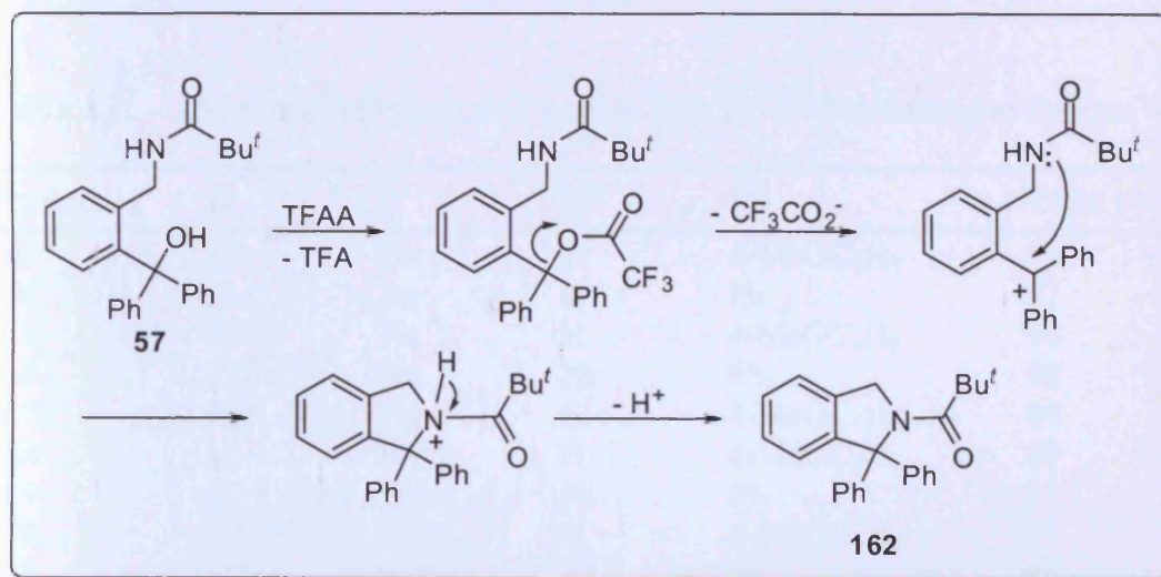
Scheme 4.2
