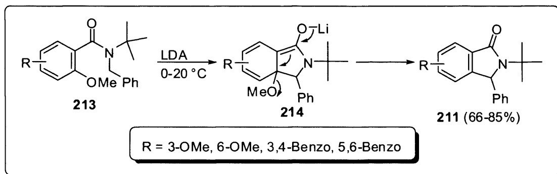
Scheme 6.3
