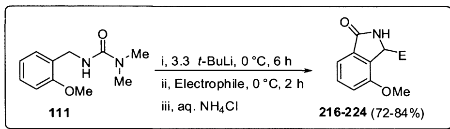
Scheme 6.6
