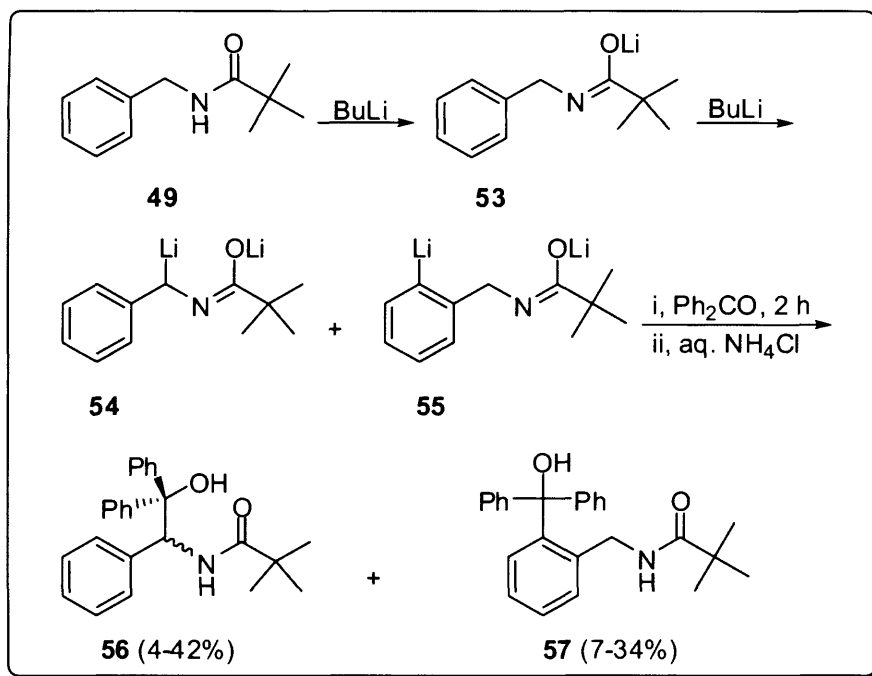
Scheme 2.5
