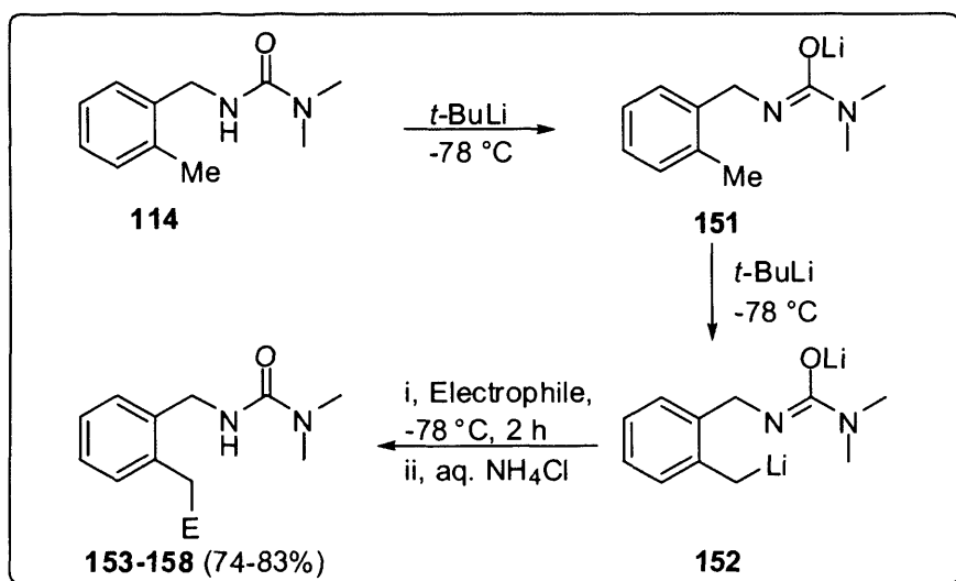
Scheme 3.8
