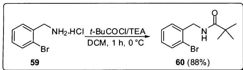
Scheme 2.6
