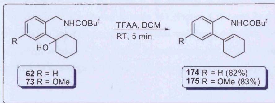
Scheme 4.4
