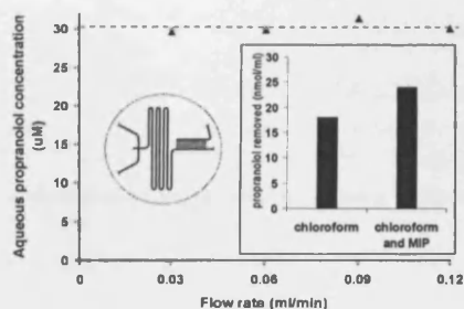
Figure 4: Propranolol remaining in the aqueous phase following on-chip extraction of a 50 \mu M sample with chloroform. Inset: Schematic of extraction chip and enhanced efficiency of extraction by incorporation of MIP affinity phase.
