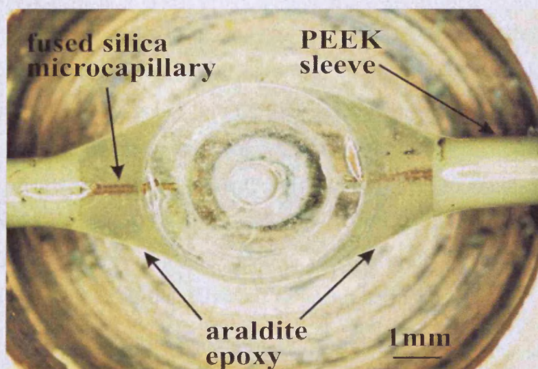
Figure 6.15. Photograph of the applied Araldite ® Precision epoxy adhesive to seal inlet/outlet microcapillary segments of the miniaturised SDR based microfluidic device (taken with a Nikon SMZ800 electron microscope).
