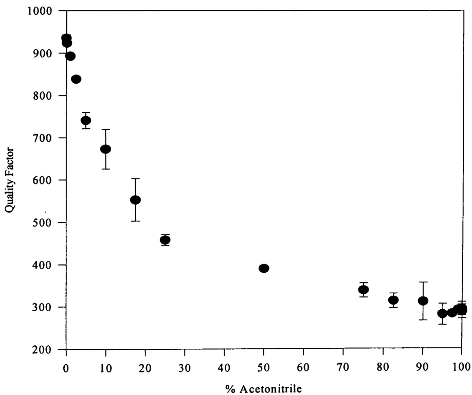
Figure 6.19. The average loaded quality factor as a function of solution composition for the acetonitrile:toluene system in miniaturised SDR.
