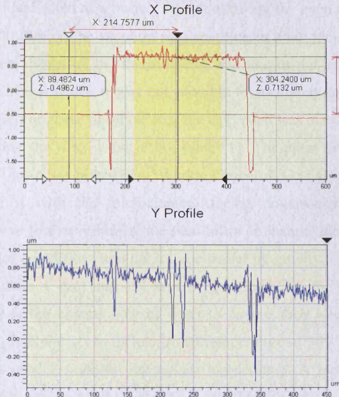
Figure 6.11. Veeco NT 3300 Optical Interferometer image showing the \approx 1.2 \mu\text{m} thick Teflon ® AF 1600 film on a sapphire sample, as can be viewed in the X profile.
