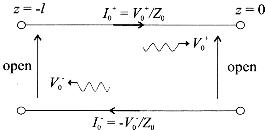
Figure 3.2. Open-circuited TL.
