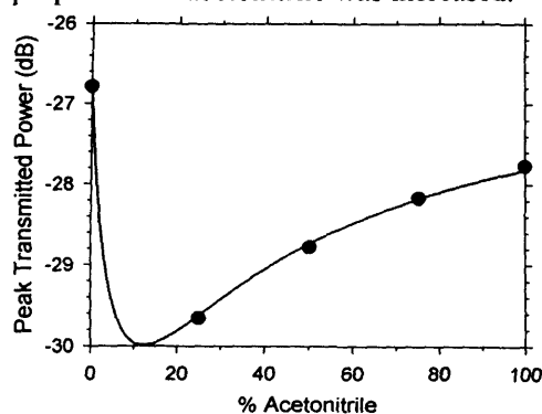
Figure 5. The peak transmitted power (in dB) as a function of composition. The theoretical dependence is shown by the solid line.
