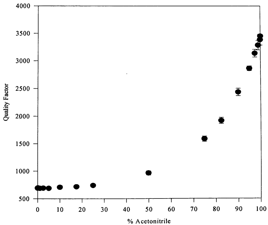
Figure 5.26. The loaded quality factor as a function of solution composition for the acetonitrile:water system in SDR.
