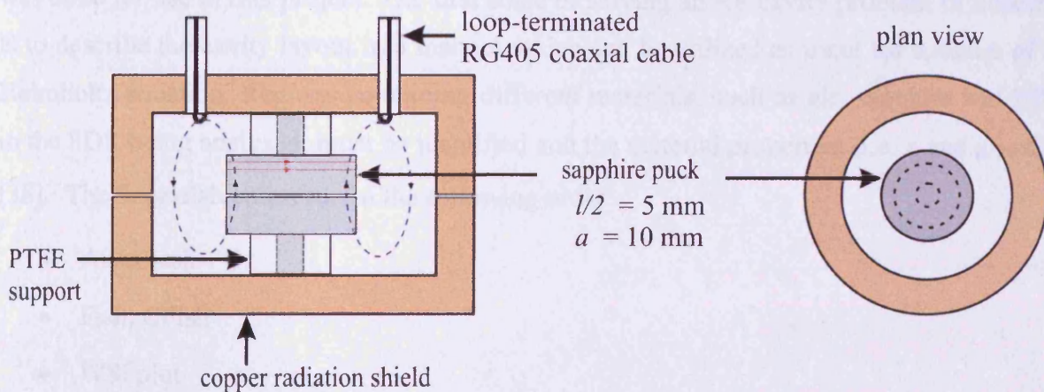
Figure 4.9. Schematic diagram of SDR and its microwave field profile. The TE_{018} mode E field is illustrated by solid red lines while H field is shown by dotted blue ellipses.
