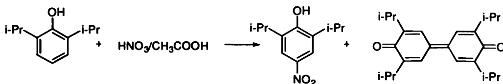
Scheme 3.17. Synthesis of 4-nitro-2,6-di-iso-propylphenol. Reagents and condition: \text{HNO}_3 , acetic acid, DCM, 0 °C.
