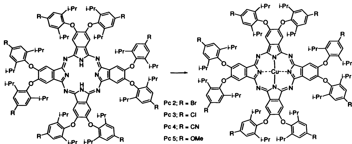
Scheme 3.22. Synthesis of PcCus . Reagents and conditions: Cu(OOCCH_3)_2 , DCM, 0 °C.
