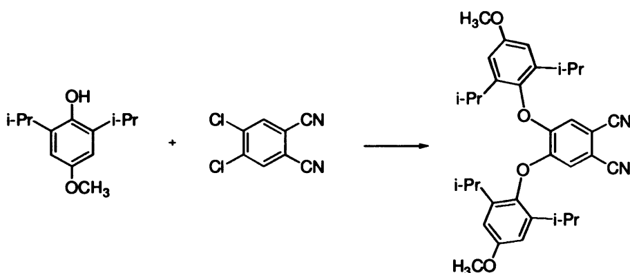
Scheme 3.11. Synthesis of PnOMe . Reagents and conditions: K_2CO_3 , DMF, 70 °C.
