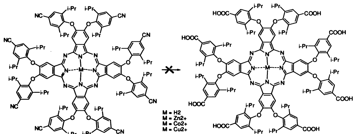
Scheme 3.24. Attempted synthesis of PcCOOHs. Reagents and conditions: KOH (85% aqueous solution), ethanol, reflux.
