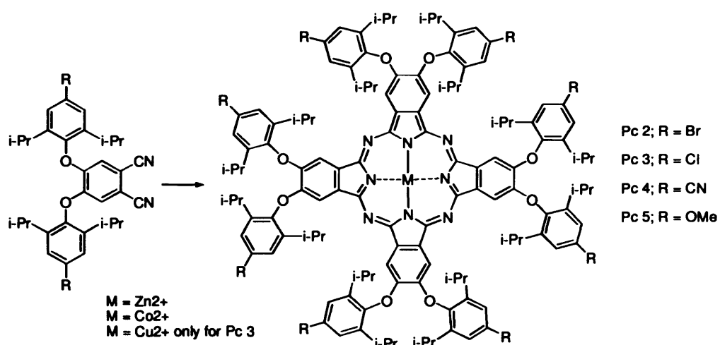
Scheme 3.20. Synthesis of PcsM . Reagents and conditions: Metal salt, NMP, 165 °C.
