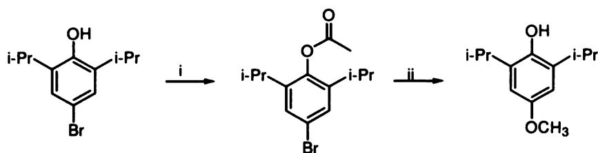
3.10. Protection of 4-bromo-2,6-di- iso -propylphenol and synthesis of 4-methoxy-2,6-di- iso -propylphenol. Reagents and Conditions: i) Acetic anhydride, H 2 SO 4 . ii) NaOCH 3 /CH 3 OH, DMF, CuBr, 110 °C
