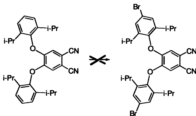
Scheme 3.2. Bromination of Pn1 .
