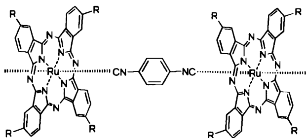
Figure 1.3 Phthalocyaninoruthenium 'shish-kebab' complex.
