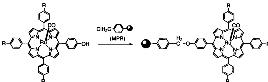
Scheme 1.4. Ruthenium porphyrins covalently immobilized onto Merrifield's peptide resin.
