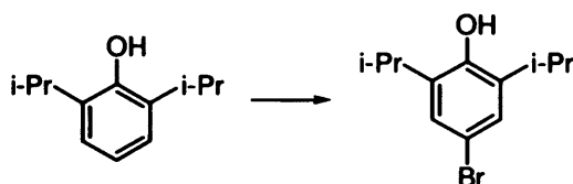
Scheme 3.3. Bromination of 2,6-di- iso -propylphenol. Reagents and conditions: Br 2 , DCM.
