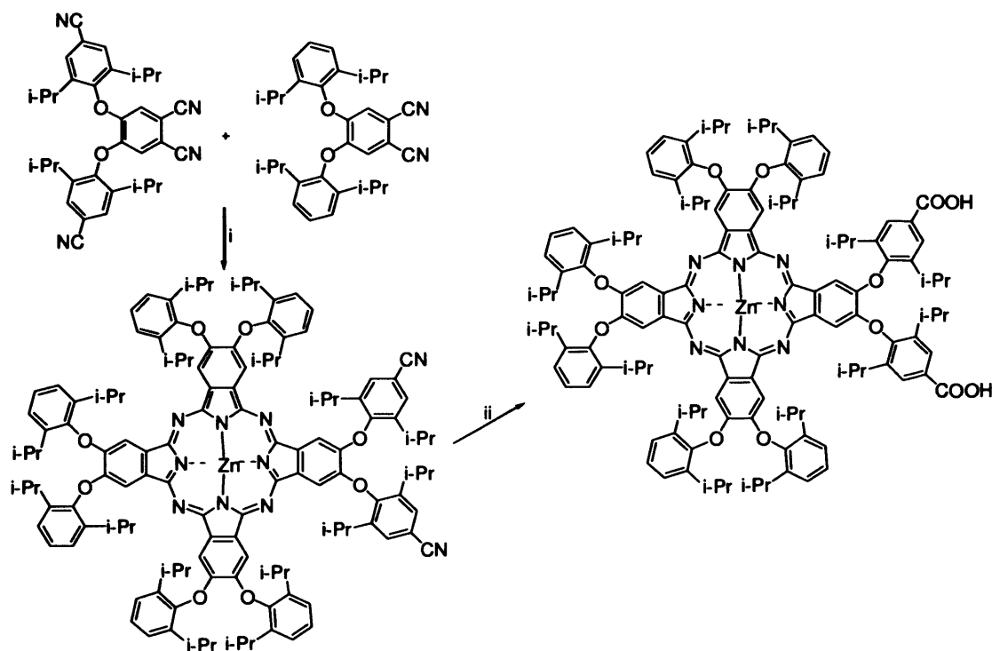
Scheme 3.26. Synthesis of Pc1 3 PcCNZn i) Zn(II)acetate, NMP, 165 °C. Synthesis Pc1 3 PcCOOHZn ii) KOH, ethylene glycol, 24h, 160 °C. H 2 PO 4 , 160°C, 24h.
