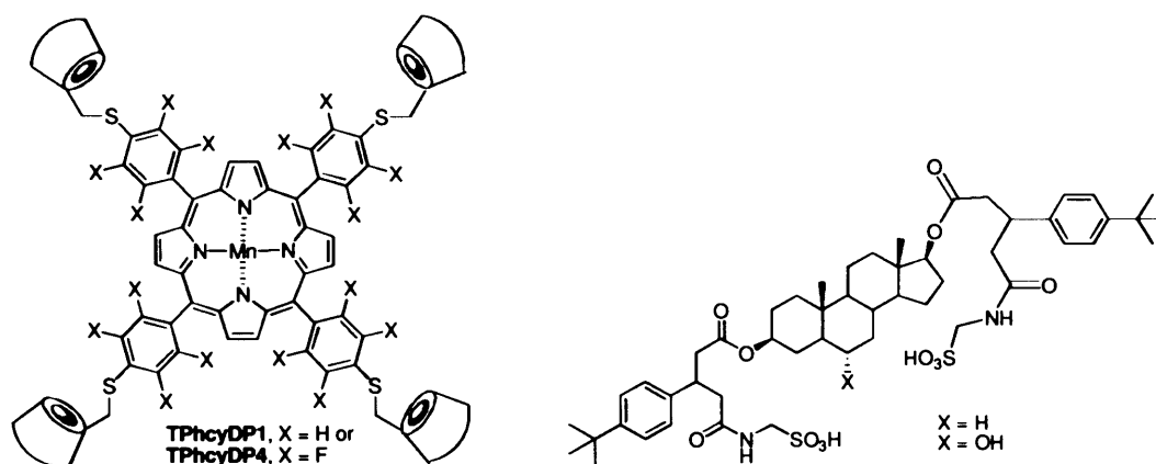
Figure 1.5 Cyclodextrin substituted porphyrin catalysts.
