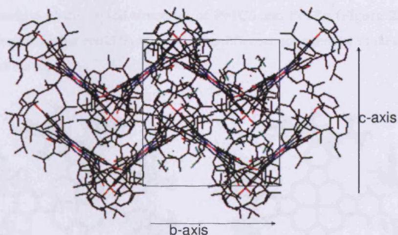
Figure 2.1 The monoclinic packing of Pc1Co , view along a axis.
