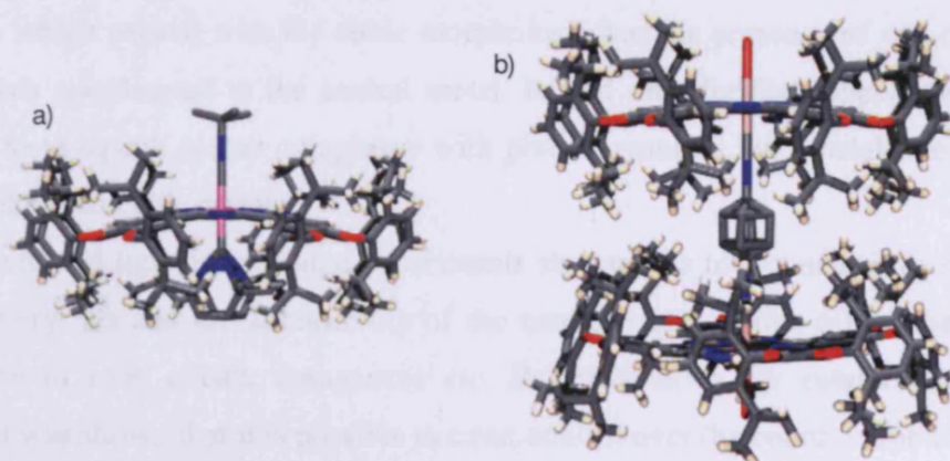
Figure 2.20. Edge-on molecular view of the molecular structures of a) Pc1Ru( t -BuNC) 2 and b) Pc1Ru(1,4-phenylenediisocyanide)(O 2 )
