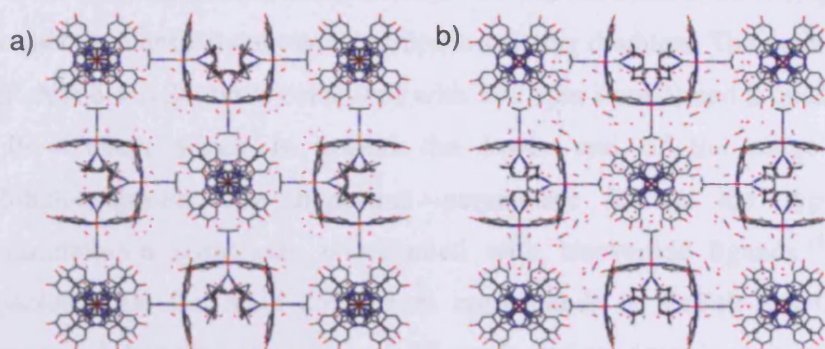
Figure 2.12. The cubic packing arrangement of a) \text{Pc1Fe}(t\text{-BuNC})_2 , and b) \text{Pc1Ru}(t\text{-BuNC})_2 .
