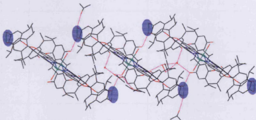
Figure 3.4 Hydrogen bonding interactions between PcOHZn molecules in the crystals
