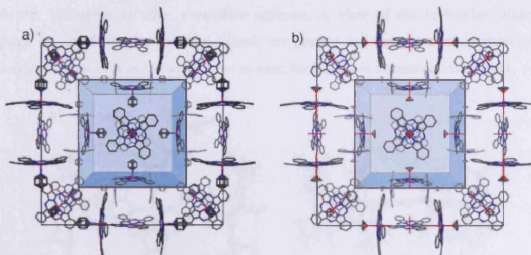
Figure 2.4 The cubic packing arrangement of Pc1Co (the 2,6-di-isopropylphenoxy substituents have been removed for clarity) a) recrystallised from pyridine/ \text{CHCl}_3 /MeOH – note the pyridine axial ligands; b) recrystallized from slow diffusion of MeOH into DCM – note the \text{H}_2\text{O} and MeOH axial ligands (MeOH pointing towards the centre of the cubic void).
