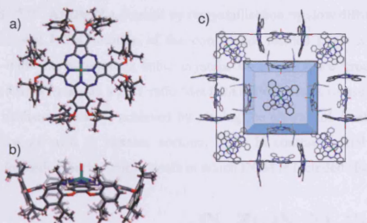
Figure 1.15. The molecular and crystal structure of Pc1Zn . a) Face-on and b) edge-on molecular views c) The cubic packing arrangement of Pc1Zn , the phenoxy substituents have been removed for clarity. The outer cube represents the unit cell, the inner cube represents one of the two voids of volume 8 \text{ nm}^3 found in each unit cell, and the second nanovoid is distributed at each corner of the unit cell in 8 \times 1 \text{ nm}^3 portions
