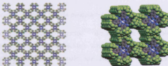
Figure 1.13. Packing arrangement of F_{64}PcH_2 along the c axis.
