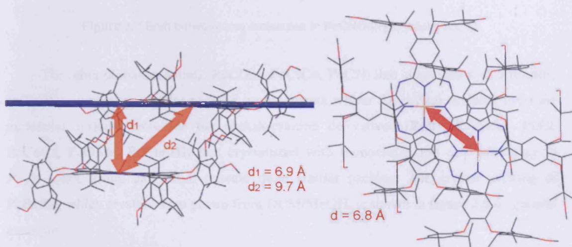
Figure 3.6 Shift between two phthalocyanine molecules in PcOMeCu crystal packing.
