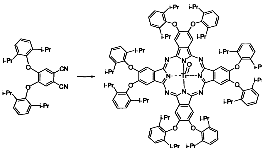
Scheme 2.13. Synthesis of Pc1TiO . Reagents and conditions: Titanium(IV) butoxide, NMP, 165 °C.
