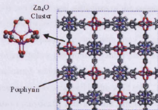
Figure 1.12. Crystal structure of interpenetrated PIZA-4 along the cubic axis.
