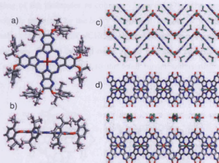
Figure 1.16 The molecular and crystal structure of AzaPc1 ( M = \text{Ni} ). a) Face-on and b) side views. c) A view of the herringbone arrangement of the macrocycles looking down the x axis of the crystal. d) A view along the z axis of the crystal showing the disordered solvent (DCM, acetone and \text{H}_2\text{O} ) the 2,6-di- iso -propylphenoxy groups are not shown in for clarity c) and d).
