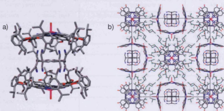
Figure 2.18 a) Edge-on molecular view of the molecular structure and b) cubic packing arrangement of Pc1Zn(H 2 O) with 1,6-diaminohexane molecules as included guest.
