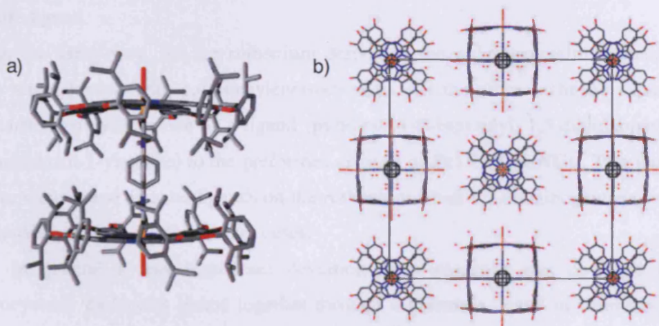
Figure 2.19 a) Edge-on molecular view of the molecular structure and b) cubic packing arrangement of Pc1Fe(1,4-phenylenediisocyanide)(O 2 ) .
