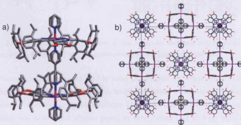
Figure 2.17 a) Edge-on molecular view of the molecular structure and b) cubic packing arrangement of Pc1Co(bipy)(Py) .
