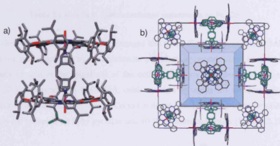
Figure 2.16 a) Edge-on molecular view of the molecular structure and b) cubic packing arrangement of Pc1Co(1,6-diaminohexane)(H 2 O) .
