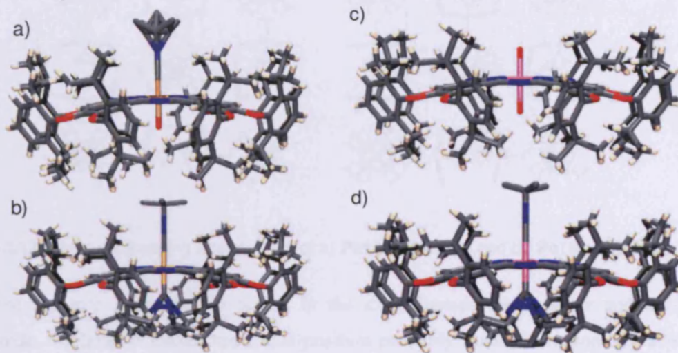
Figure 2.11 Edge-on molecular views of the molecular structure of a) Pc1Fe( t -BuNC)(H 2 O) , b) Pc1Fe( t -BuNC) 2 , c) Pc1Ru(H 2 O) 2 and d) Pc1Ru( t -BuNC) 2 .
