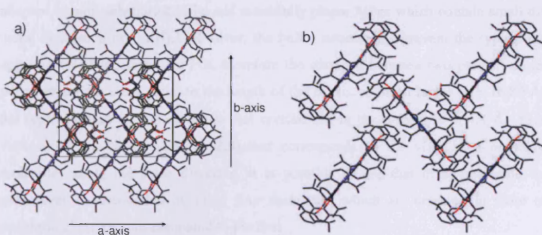
Figure 2.7 a) The orthorhombic packing of Pc1 , view along c axis. b) A monomolecular layer along c .
