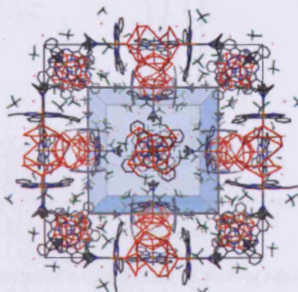
Figure 2.13. The cubic packing arrangement of \text{Pc1Fe}(t\text{-BuNC})(\text{H}_2\text{O}) .
