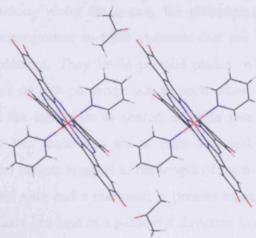
Figure 3.7 Shift between two molecules in PcNCoPy crystal packing.
