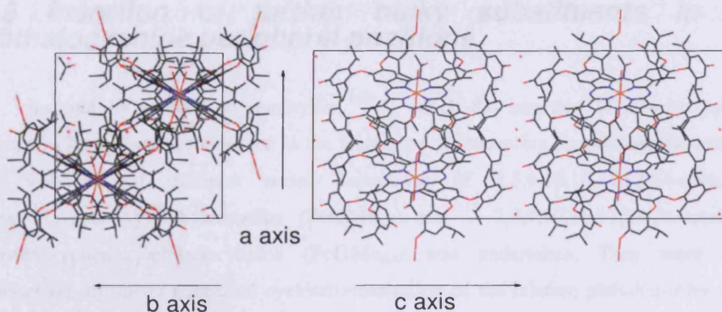
Figure 3.9. The monoclinic packing of PcOHCu crystals
