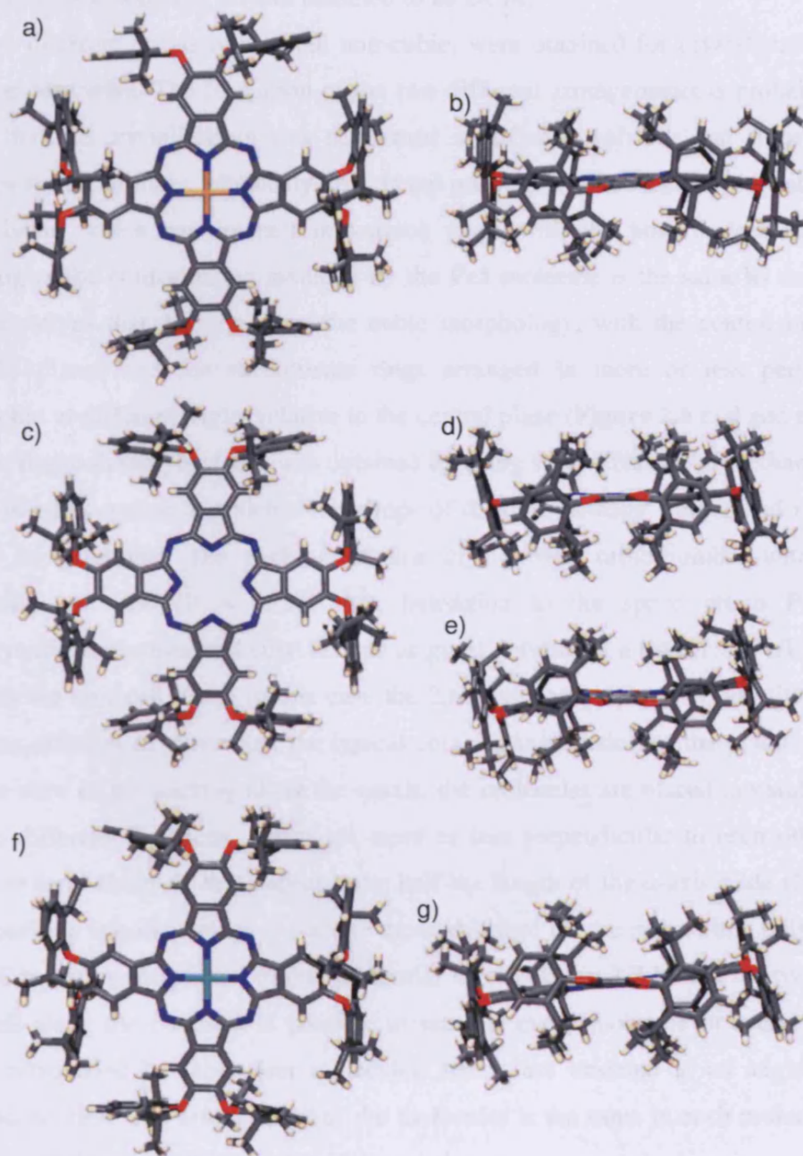
Figure 2.6. The molecular structures of Pc1Cu , Pc1 and Pc1Ni . Pc1Cu a) Face-on and b) edge-on views; Pc1 c) Face-on and edge-on molecular views d) in the orthorhombic packing e) in the monoclinic packing. Pc1Ni f) Face-on and g) edge-on molecular views.
