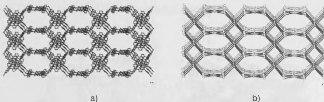
Figure 1.10. Extended structure of a) the ((\text{Cu(II)(tpp)Cu(I)})^{n+}) framework and b) the two interpenetrating frameworks of ((\text{Cu(II)(tcp)Cu(I)})_n)^n .
