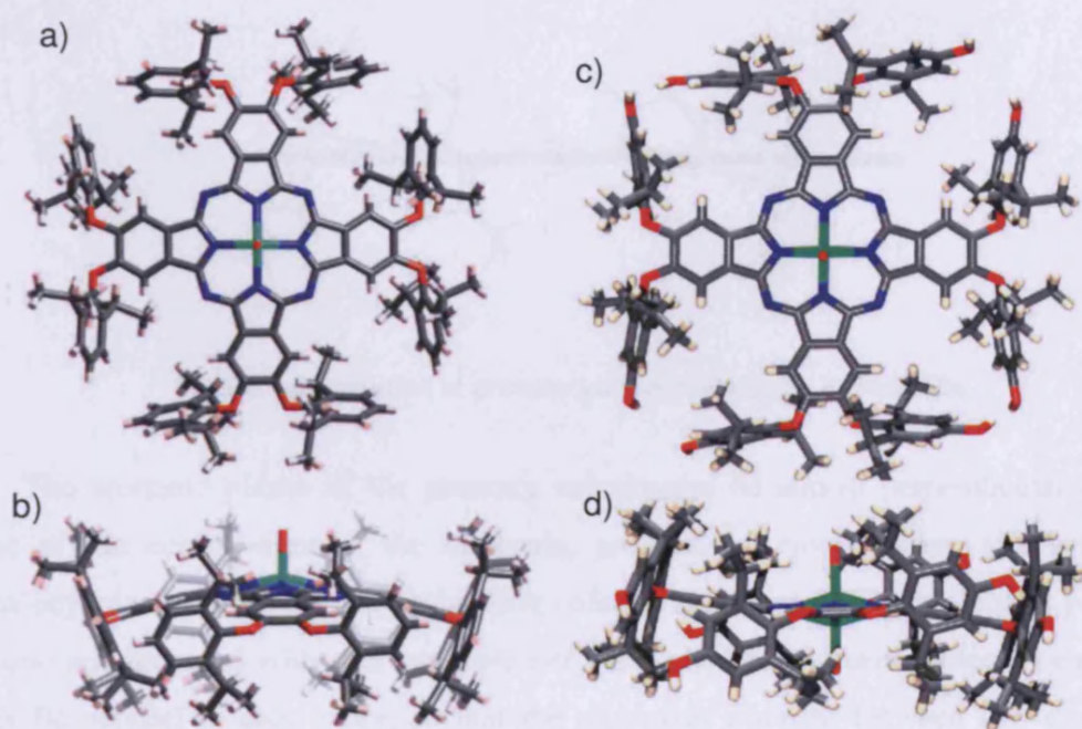
Figure 3.3 The molecular structure of Pc1Zn . a) Face-on and b) edge-on molecular views, and PcOHZn . c) Face-on and d) edge-on molecular views.
