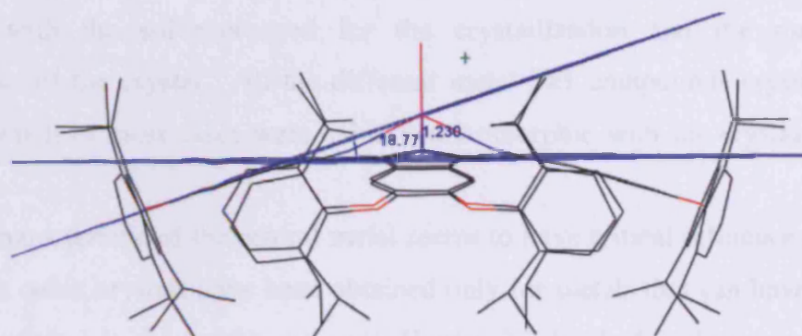
Figure 2.15 Edge-on molecular view of PcInCl . Measurement of the displacement from the plane of the metal and measurement of the angle of deviation from planarity of the Pc molecule.
