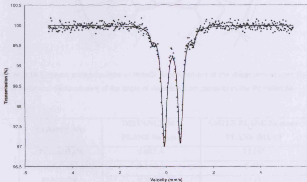
Figure 2.14. Mossbauer spectrum of a suspension of \text{Pc1Fe}(t\text{-BuNC})_2 crystals in FOMBLIN Y ® measured at 80 K.
