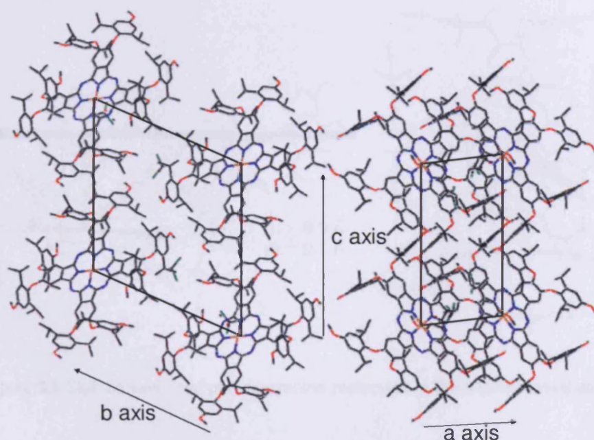
Figure 3.5. The triclinic packing of PcOMeCu
