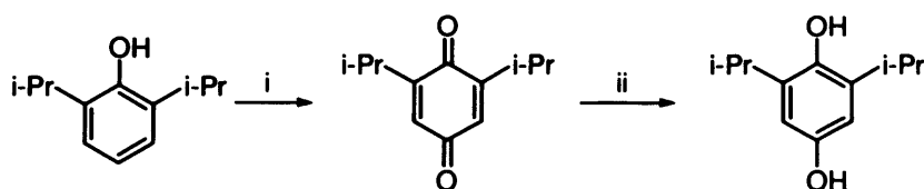
Scheme 3.7. Synthesis of 2,6-di- iso -propyl-p-quinone and of 2,6-di- iso -propyl-p-hydroquinone. Reagents and Conditions: i) HClO 4 (70%), PbO 2 , acetic acid; ii) NaBH 4 , MeOH, 0 °C
