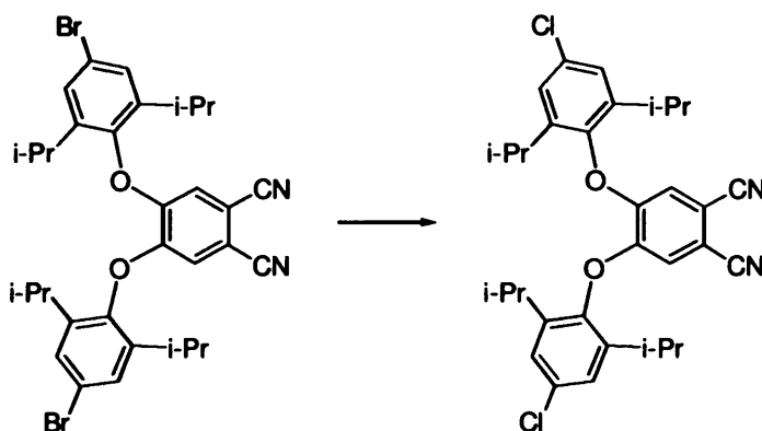
Scheme 3.5. Synthesis of Pn3 . Reagents and conditions: CuCl, anhydrous DMF, 150 °C
