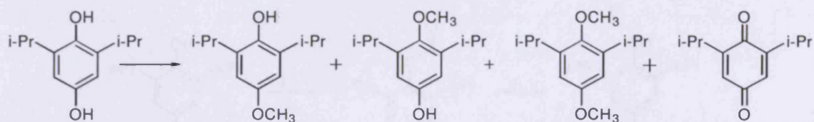
Scheme 3.8. Synthesis of 4-methoxy-2,6-di- iso -propylphenol. Reagents and Conditions: a) \text{CH}_3\text{I} , \text{K}_2\text{CO}_3 , 2-butanone; b) (\text{CH}_3)_2\text{SO}_4 , \text{K}_2\text{CO}_3 , acetone; c) p -toluene-methylsulfonate, \text{NaOH} (20%) or \text{K}_2\text{CO}_3 , acetone
