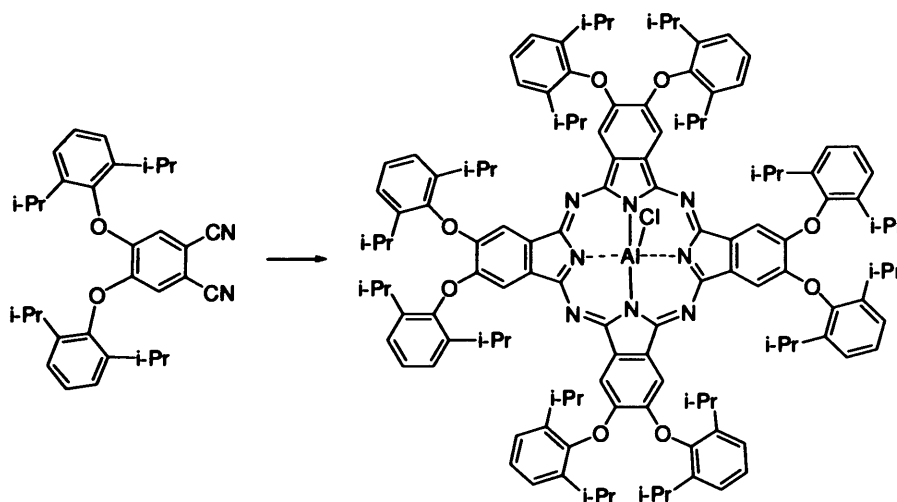
Scheme 2.15. Synthesis of Pc1AlCl . Reagents and conditions: Aluminum(III) chloride, quinoline, 160 °C.
