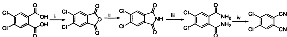
Scheme 2.1. Synthesis of 4,5-dichlorophthalonitrile. Reagents and conditions: i) acetic anhydride, reflux, 5h; ii) formamide, reflux, 3h; iii) ammonia solution, r.t., 48h, iv thionyl chloride, DMF, 0-5 °C, 5h, r.t. 24 h
