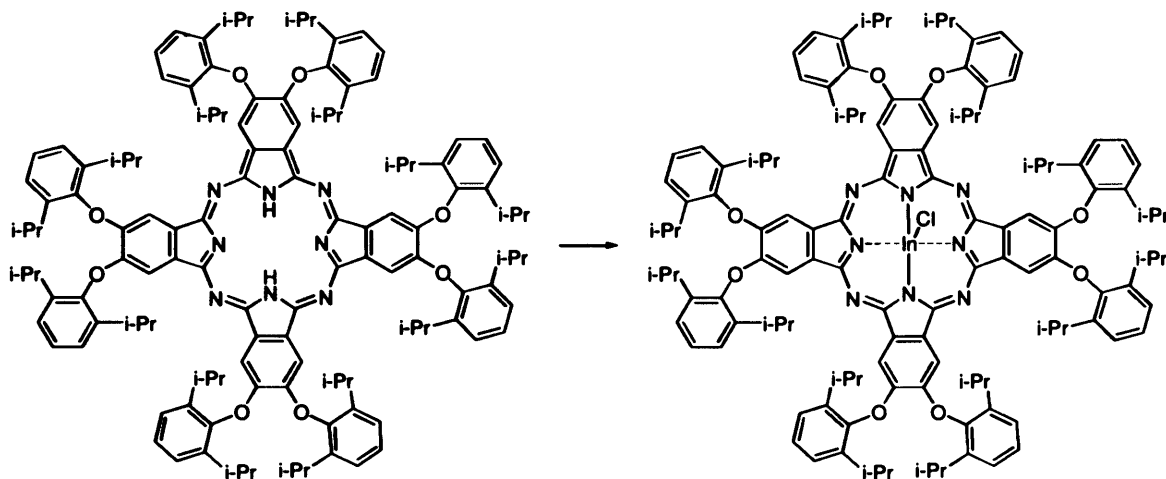
Scheme 2.14. Synthesis of Pc1InCl . Reagents and conditions: Indium(III)chloride, pentanol, reflux.
