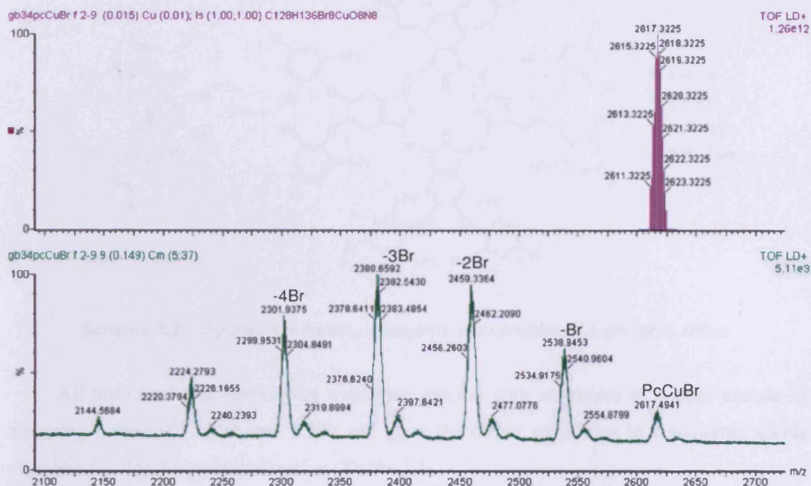
Figure 3.2 MALDI spectrum of a column chromatography fraction deriving from the attempted synthesis of PcBrCu using copper acetate.
