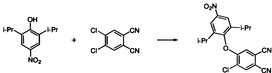
Scheme 3.19. Attempted Synthesis of PnNO 2 . Reagents and conditions: \text{K}_2\text{CO}_3 , DMF 70 °C
