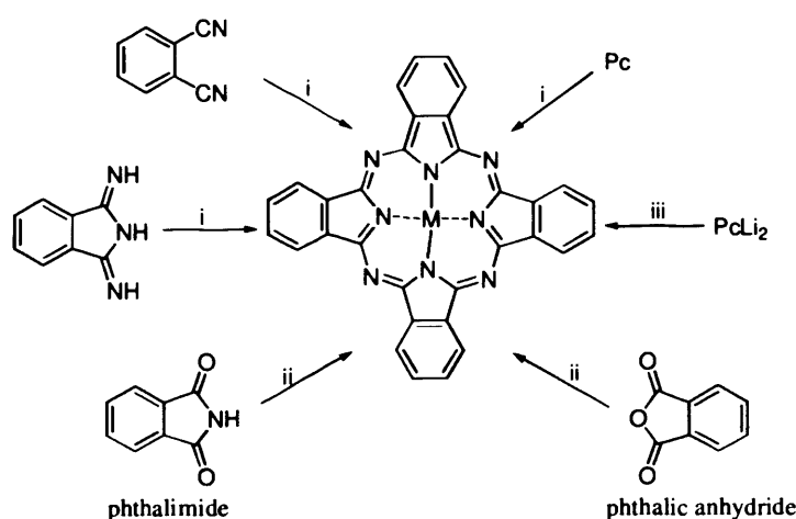
Scheme 1.2. Synthetic routes to MPc . Reagents and conditions: i) Heat in a high-boiling-point solvent (e.g. quinoline) with metal salt. ii) Heat in a high-boiling-point solvent with metal salt and urea. iii) Heat in ethanol with metal salt.
