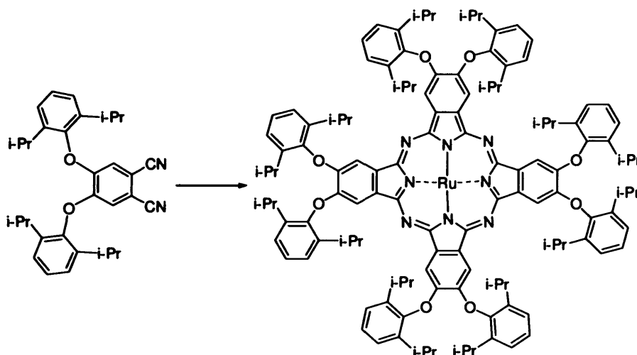
Scheme 2.11. Synthesis of Pc1Ru . Reagents and conditions: Ruthenium(III) chloride, DBU, 160 °C.
