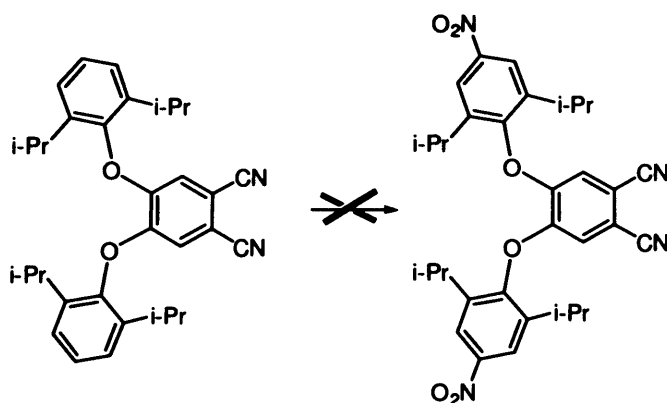
Scheme 3.16. Nitration of Pn1 . Reagents and conditions: a) HNO 3 /H 2 SO 4 ; b) HNO 3 /CH 3 COOH, DCM.
