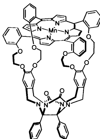
Figure 1.4 Diphenylglycoluril-based cavity Mn porphyrin.
