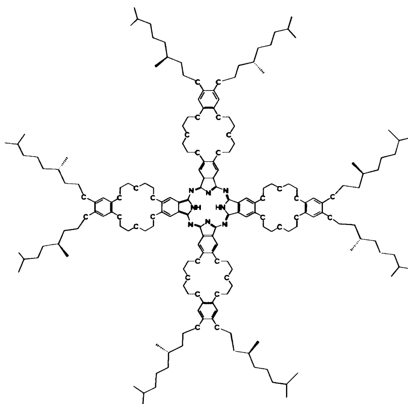
Figure 1.2 Chemical structures of crown ether phthalocyanine Pc-18-crown-6 .
