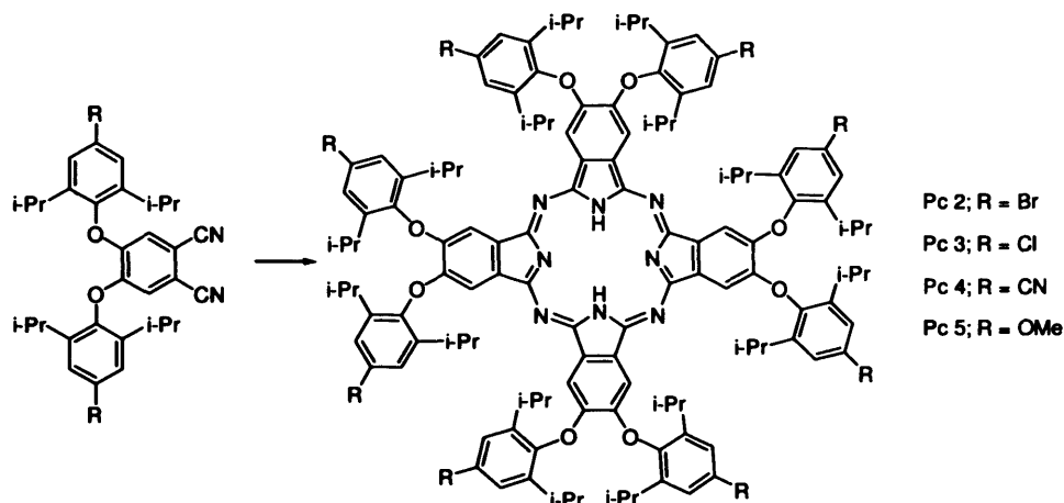
Scheme 3.21. Synthesis of PcRH_2 . Reagents and conditions: Li, pentanol, reflux.
