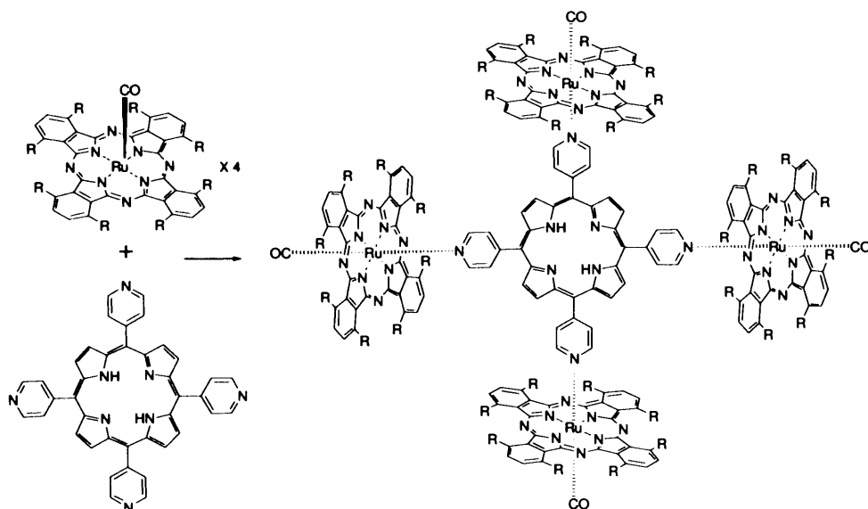
Scheme 1.3 Supramolecular assembly of porphyrins and phthalocyanine molecules through pyridine-ruthenium axial ligand coordination.
