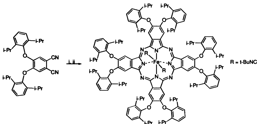
Scheme 2.10. Synthesis of Pc1Fe . Reagents and conditions: i) Lithium metal, iron(II) acetate, n -pentanol, reflux; ii) t -butylisocyanide 50 °C.
