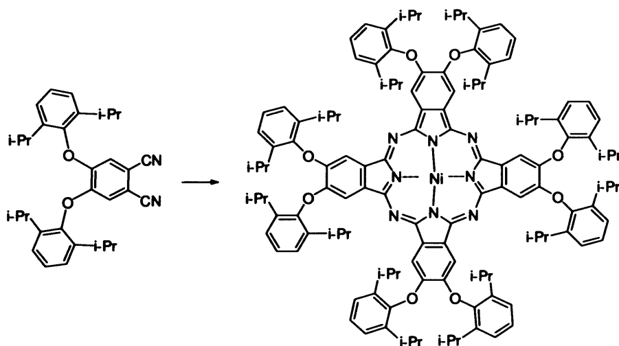
Scheme 2.6. Synthesis of Pc1Ni . Reagents and conditions: \text{NiCl}_2 , quinoline, 165 °C
