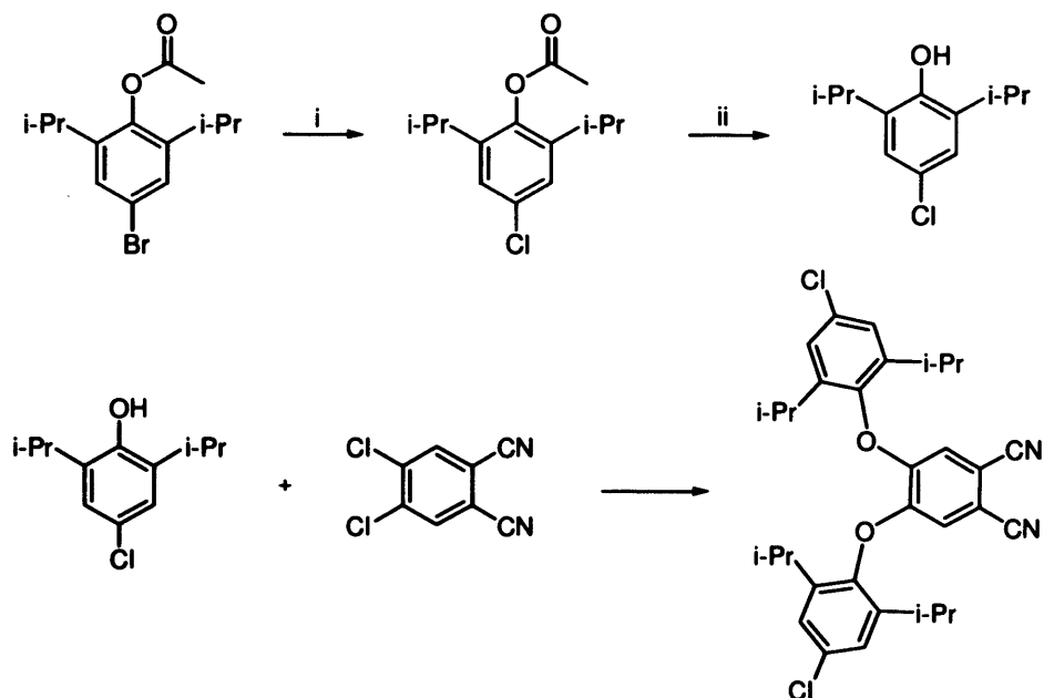
Scheme 3.13. Synthesis and hydrolysis of the 4-acetoxy-3,5-di-iso-propyl-chlorobenzene. Reagents and conditions: i) CuCl, DMF, 150°C. ii) NaOH (40%), MeOH and synthesis of PnCl . Reagents and conditions: K 2 CO 3 , anhydrous DMF, 70 °C.
