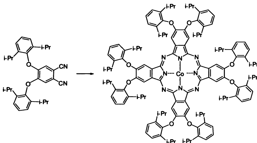
Scheme 2.3. Synthesis of Pc1Co . Reagents and conditions: CoAc 2 , NMP, 165 °C.
