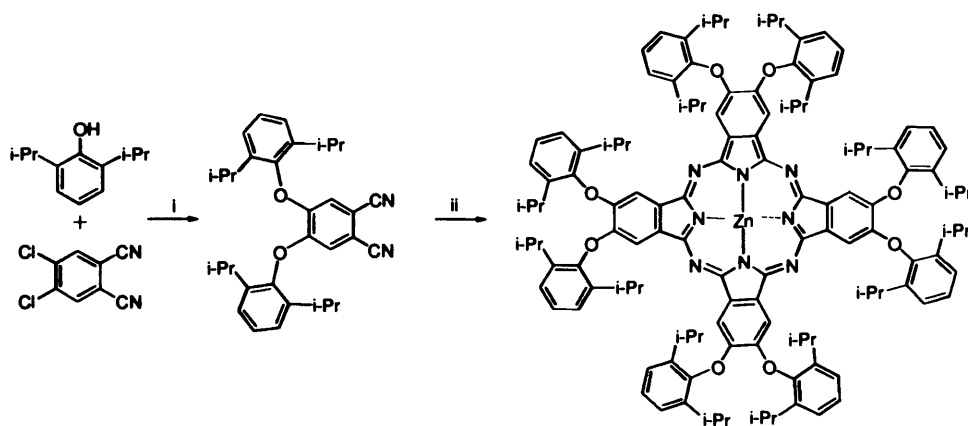
Scheme 1.5. The synthesis of Pc1Zn . Reagents and conditions: i) K_2CO_3 , DMF, 70 °C; ii) Zn(OAc)_2 , NMP, 150 °C.
