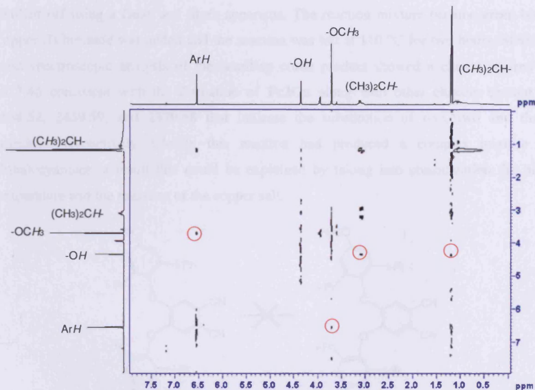
Figure 3.1. ^1\text{H} NOESY NMR of 4-methoxy-2,6-di- iso -propylphenol.
