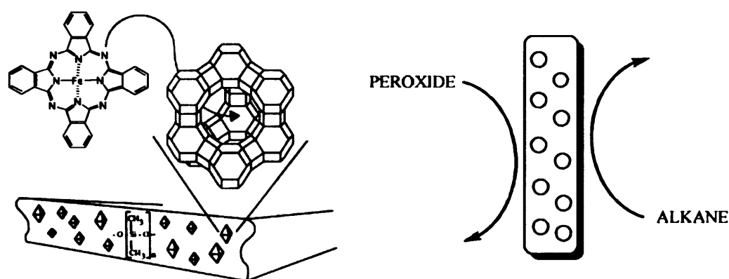
Figure 1.7. Schematic representation of the incorporation of PcFe complex in the supercages of zeolite Y and subsequent incorporation of these zeolite crystals in the PDMS-membrane.
