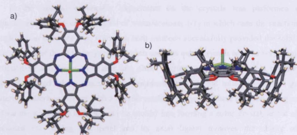
Figure 2.10 The molecular structure of Pc 1 Mg . a) Face-on and b) edge-on molecular view.
