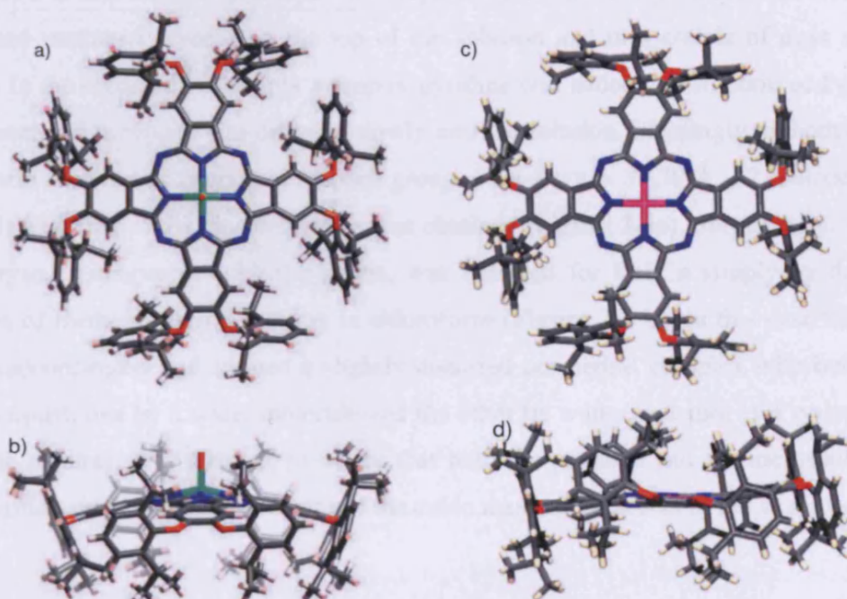
Figure 2.3 The molecular structure of Pc1Zn . a) Face-on and b) edge-on molecular views, and Pc1Co . c) Face-on and d) edge-on molecular views
