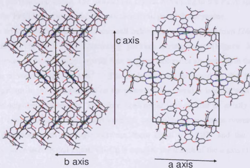
Figure 3.8 The monoclinic packing of PcBrZn crystals from DCM/MeOH.
