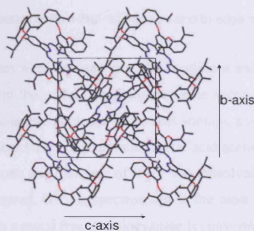
Figure 2.9 The monoclinic packing of Pc1, view along a .
