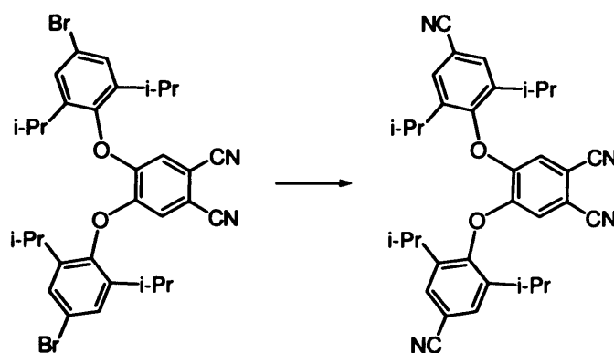
Scheme 3.6. Synthesis of Pn4 . Reagents and conditions: CuCN, anhydrous DMF, 150 °C
