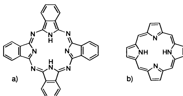
Figure 1.1. a) The structure of phthalocyanine. b) The structure of the simplest porphyrin; porphine.
