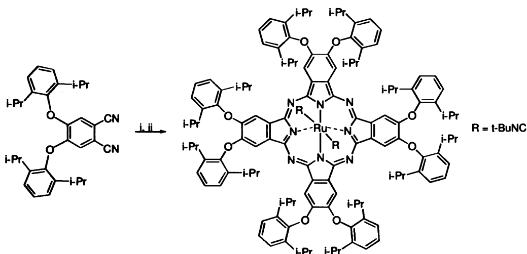
Scheme 2.12. Synthesis of \text{Pc1Ru}(t\text{-BuNC})_2 . Reagents and condition: i) Ruthenium(III) chloride, NMP, 170 °C; ii) t\text{-BuNC} , 50 °C.
