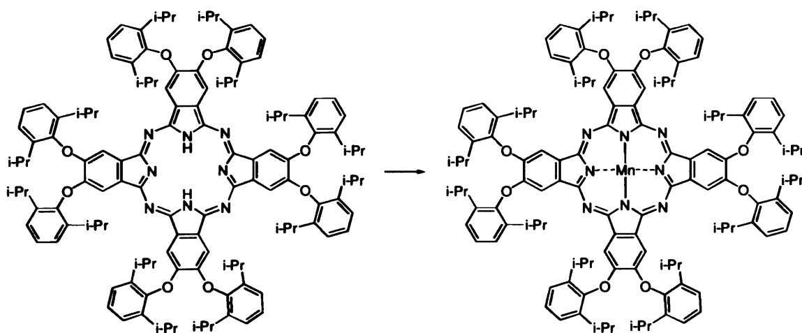
Scheme 2.8. Synthesis of Pc1Mn . Reagents and conditions: Manganese(II) acetate, DMF, reflux.
