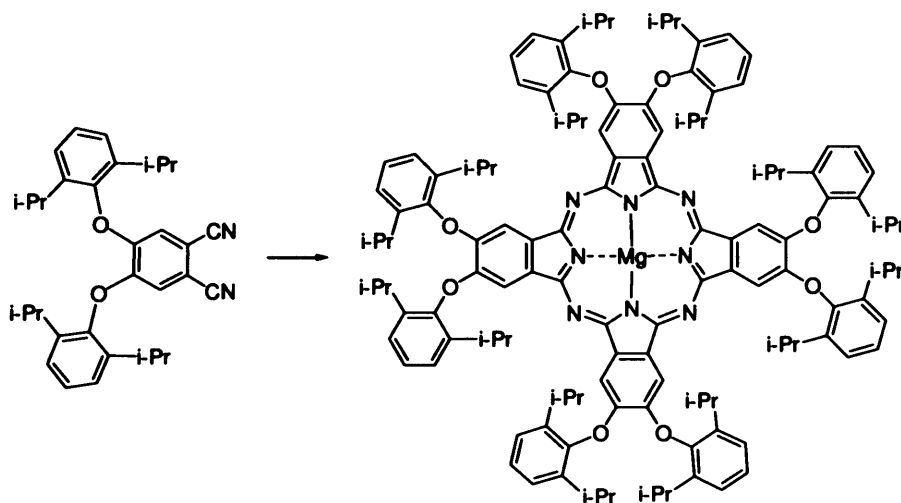
Scheme 2.7. Synthesis of Pc1Mg . Reagents and conditions: Magnesium, pentanol, iodine, reflux.
