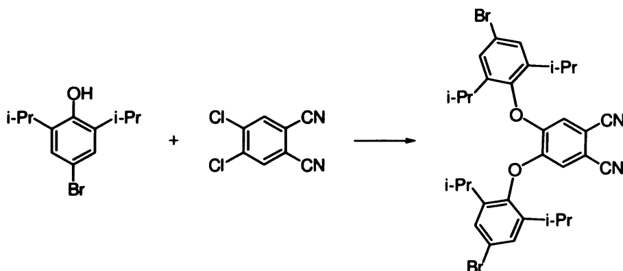
Scheme 3.4. Synthesis of PnBr . Reagents and conditions: K 2 CO 3 , anhydrous DMF 70 °C
