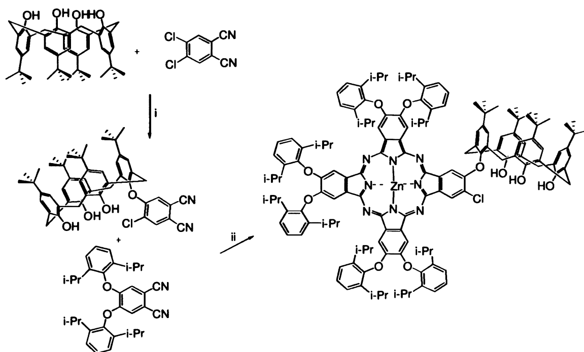
Scheme 3.27. Synthesis of Pncalix and Pc 13 PccalixZn . Reagents and conditions: i) K_2CO_3 , 70 °C, 72 h. Synthesis ii) Zn(II) acetate, NMP, 165 °C.
