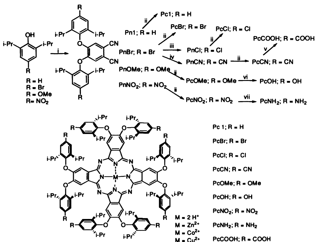
Scheme 3.1. The outline synthesis of PcR. Reagents and conditions: i) 4,5-Dichlorophthalonitrile, K 2 CO 3 , DMF 80 °C; ii) Metal acetate, NMP, 165 °C; iii) CuCl, DMF, 150 °C; iv) CuCN, DMF, 150 °C; v) KOH, EtOH, reflux; vi) BBr 3 , CH 2 Cl 2 , rt; vii) Sn, HCl
