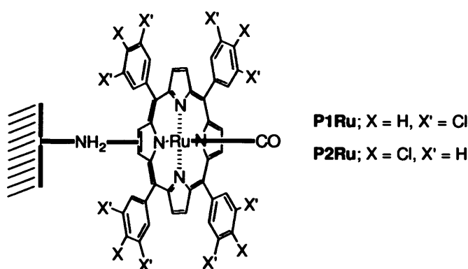
Figure 1.6. Schematic structures of Ruthenium porphyrins. a) coordinatively grafted onto the surface modified MCM-41 .
