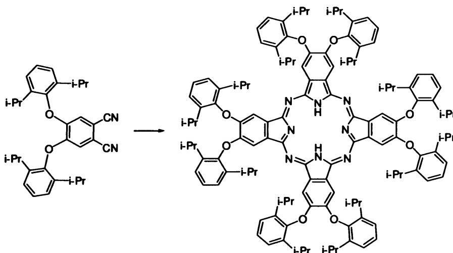
Scheme 2.4. Synthesis of Pc 1 . Reagents and conditions: i) Li, n -pentanol, reflux; ii) dilute CH 3 COOH.
