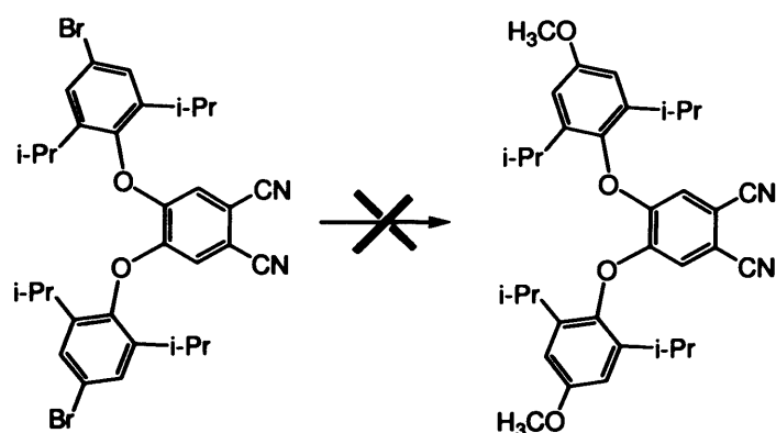
Scheme 3.9. Synthesis of PnOMe . Reagents and Conditions: NaOCH 3 /MeOH, DMF, CuBr, 110 °C
