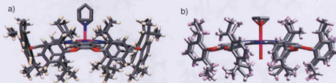
Figure 2.5 Edge-on molecular views of the molecular structure of a) Pc1CoPy , and b) Pc1Co recrystallized from \text{CHCl}_3 /MeOH.
