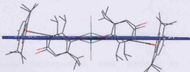
Figure 3.4 Distortion of phthalocyanine macrocycle in PcOHZn
