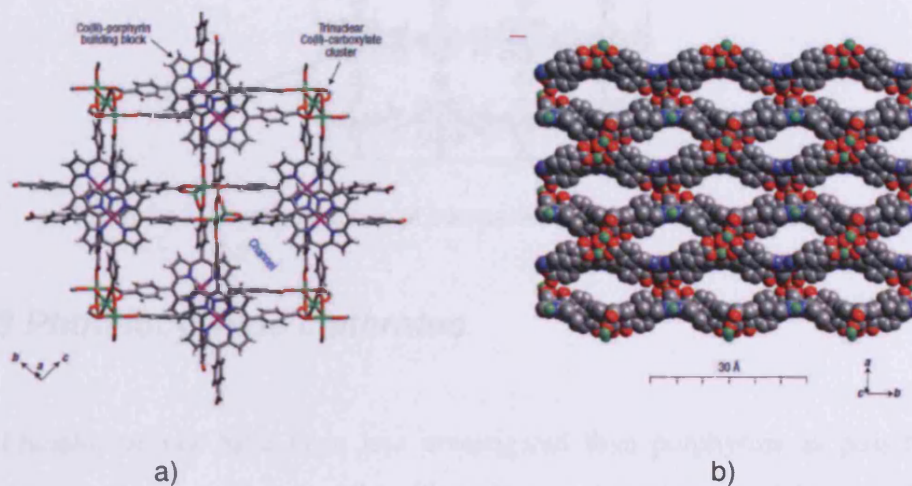
Figure 1.11. PIZA-1 network a) structure along the a axis. b) Space filling view along b or c axes.
