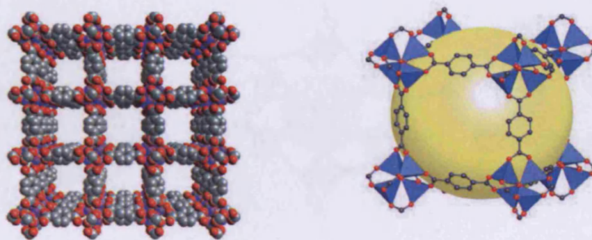
Figure 1.8. MOF-5 X-ray single crystal structure. The yellow sphere represents the size of the largest sphere that would occupy the cavity without contacting the interior van der Waals surface.
