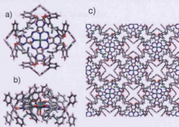
Figure 1.17. The molecular and crystal structure of AzaPc2-Zn . a) Face-on and b) side views of the molecule. c) A view of the tetragonal arrangement of the macrocycles looking down the z axis of the crystal.
