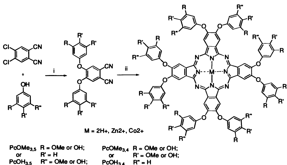
Scheme 3.25. Synthesis of dimethoxy- and dihydroxy-phenoxy substituted Pcs. Reagents and conditions: i) K 2 CO 3 , DMF 70 °C. ii) Li, pentanol, reflux or metal salt, NMP, 165 °C, followed by demethylation with BBr 3 to form the hydroxy derivatives.
