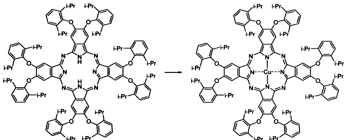
Scheme 2.5 Synthesis of Pc1Cu . Reagents and conditions: Copper(II) acetate, n-pentanol, reflux.
