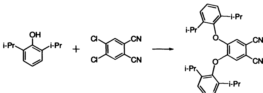
Scheme 2.2. Synthesis of Pn1. Reagents and conditions: K 2 CO 3 , DMF 80 °C.
