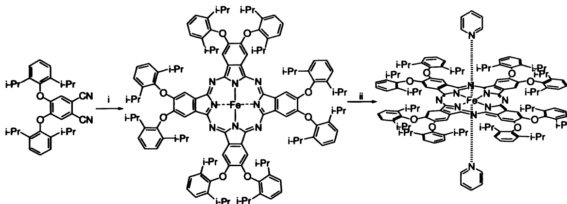
Scheme 2.9. Synthesis of Pc1Fe and Pc1Fe(py) 2 . Reagents and condition: i) \text{Fe}(\text{CO})_5 , Ethylene glycol, \mu\text{W} , 200 W, 235 °C, 240 psi. ii) pyridine.
