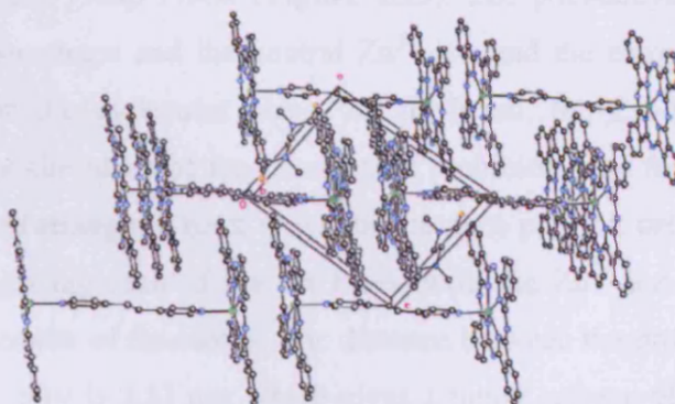
Figure 1.14. The crystal-packing of 1,2-di(4-pyridyl)ethylene PcZn complex along the b axis.
