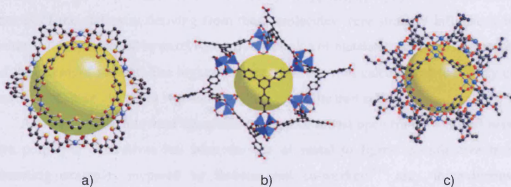
Figure 1.9. Ball and stick model of MOP-28 , MOF-177 and MOP-17 with yellow sphere showing the internal cavity.
