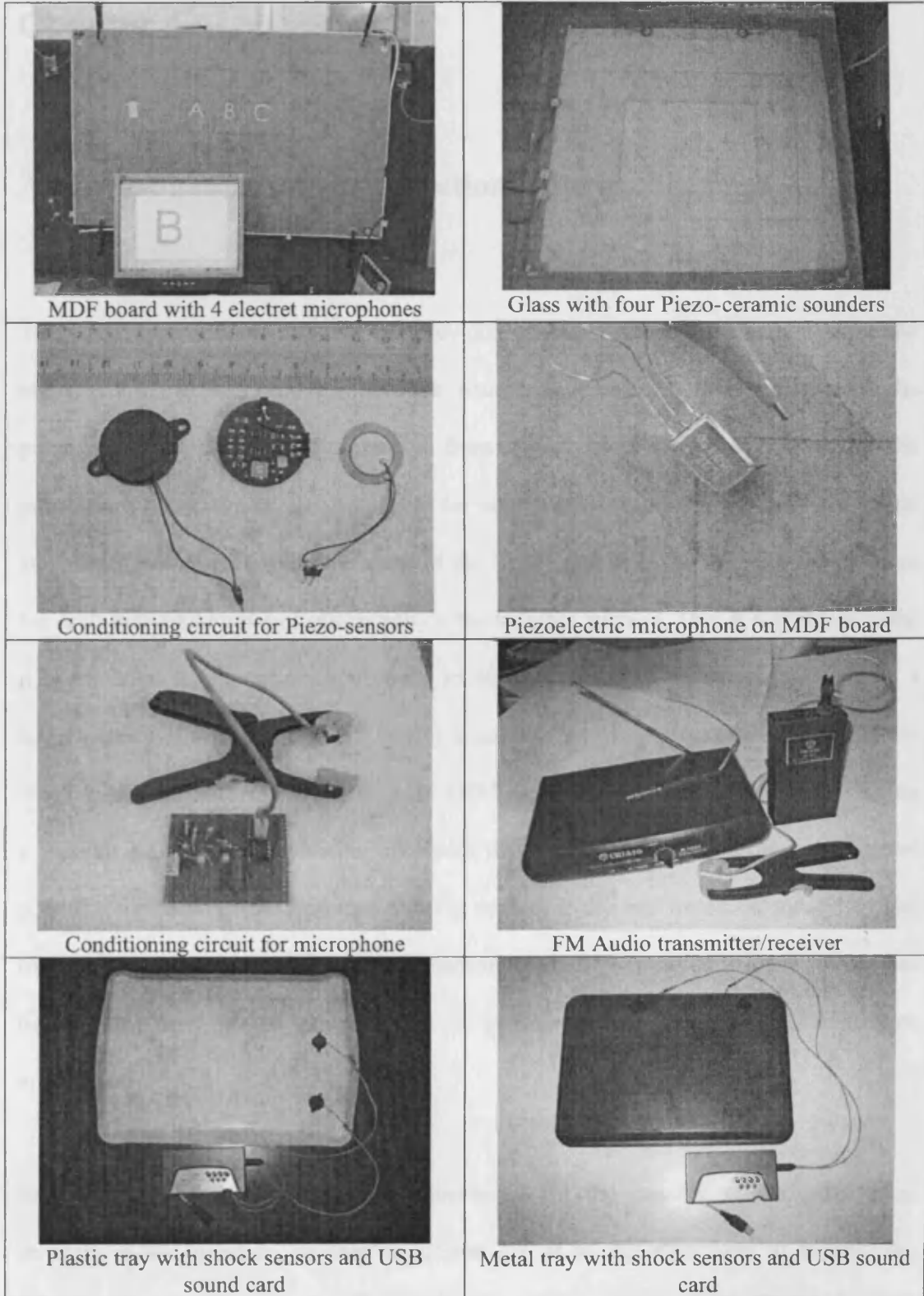
Figure 3.12. Various experimental equipment for LPM localisation.
