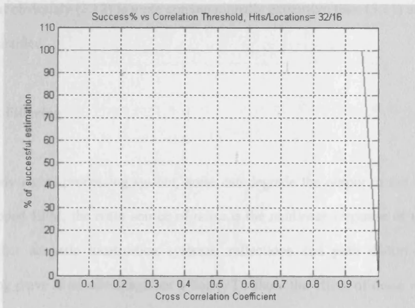
Figure 3.7. Threshold of cross correlation coefficient.
