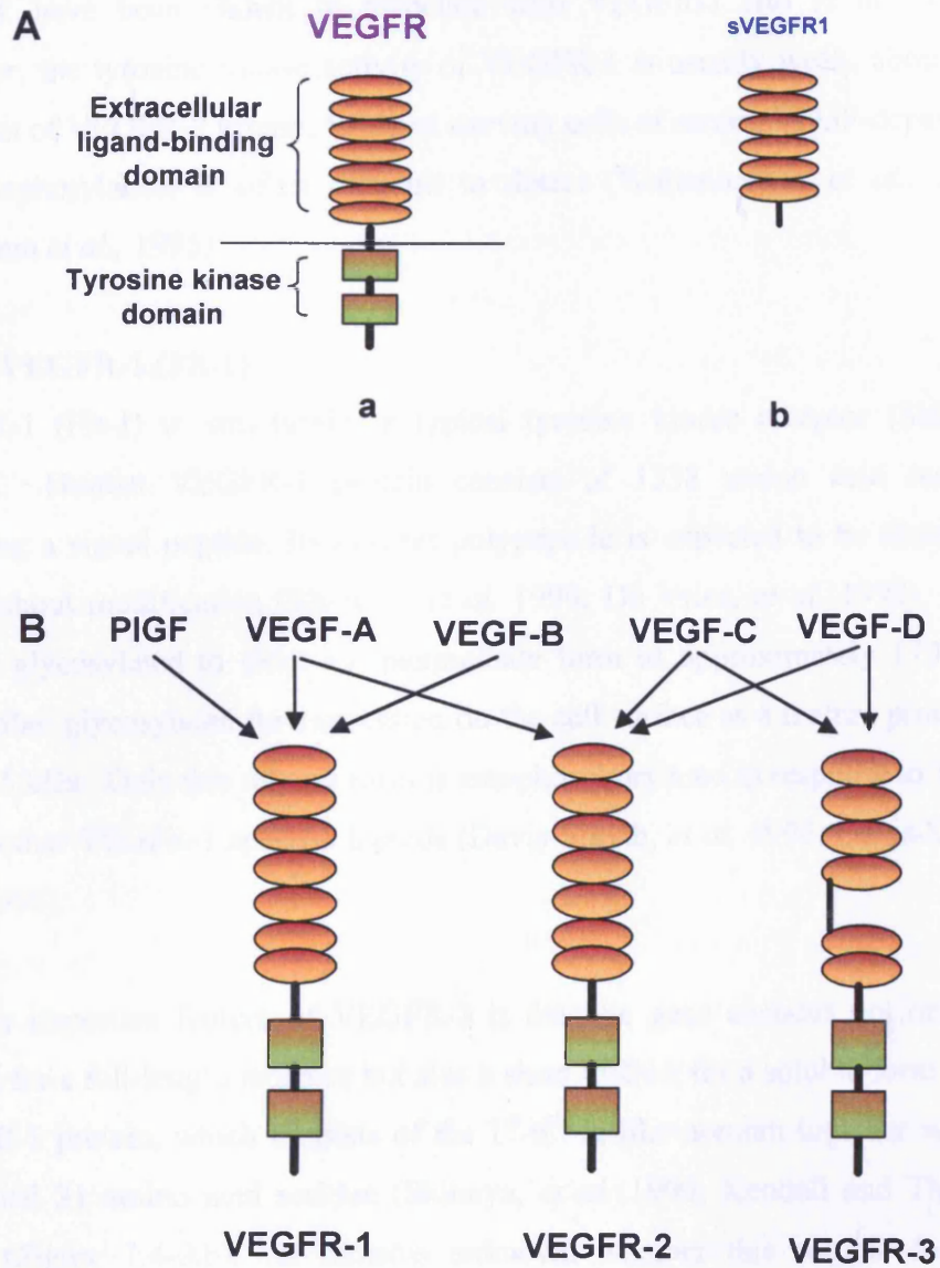
Fig 1.4 A schematic representation of the structure of VEGFRs. (A) the full-length of VEGFR-1(a) and soluble form of VEGFR-1(b); B) shows the interaction between VEGF family and their receptors (Modified from Yancopoulos et al. , 2000).
