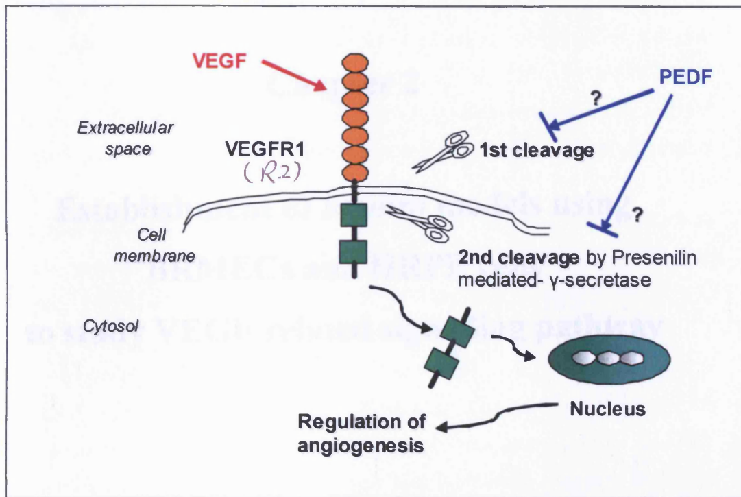
Fig 1.10b. A schematic representation of the hypothesis – the effect of VEGF/PEDF on VEGFR-1/VEGFR-2. PEDF inhibits VEGF induced angiogenesis by inhibiting the enzyme(s) activity of the first or second or both cleavages of VEGFR-1 in the RIP signalling pathway.
