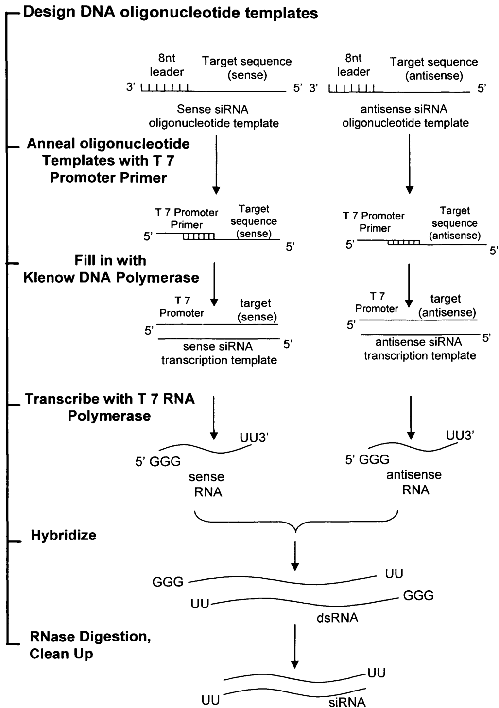
Fig 6.3 Silence siRNA Construction Kit Procedure (Adapted from the Silencer ® siRNA Construction Kit manual)
