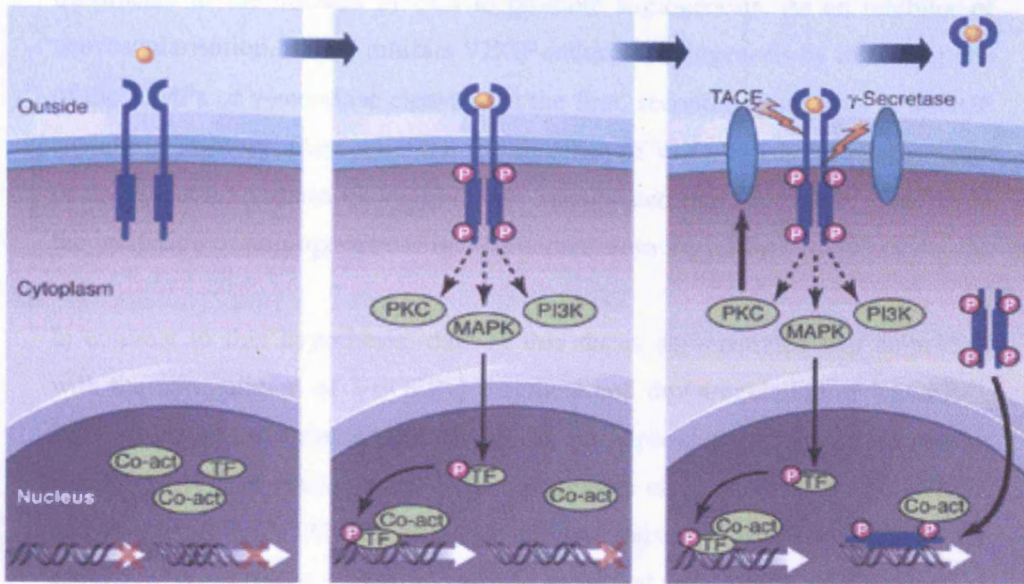
Fig 7.3 Regulated intramembrane proteolysis of a tyrosine kinase receptor. Binding of a ligand to its tyrosine kinase receptor induces activation and autophosphorylation of the receptor and the creation of docking sites for signaling proteins containing SH2 domains. In this way, different signaling pathways, such as that containing mitogen-activated protein (MAP) kinase, are activated. In a separate signaling pathway, PLC- \gamma activates PKC, which then activates the metalloprotease TACE. This enzyme cleaves off the ectodomain of the receptor and allows intramembrane cleavage of the remaining part by \gamma -secretase. The cleaved cytoplasmic region of the receptor then moves to the nucleus, where it may affect the transcription of target genes (Copied from Heldin and Ericsson, 2001).
