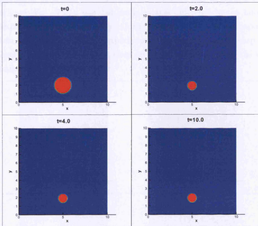
Figure 7.22: A plot of the colour function at different times, representing bubble collapse near a wall in a Newtonian fluid with \mu_s = 0.1 , h = 2.0 .
