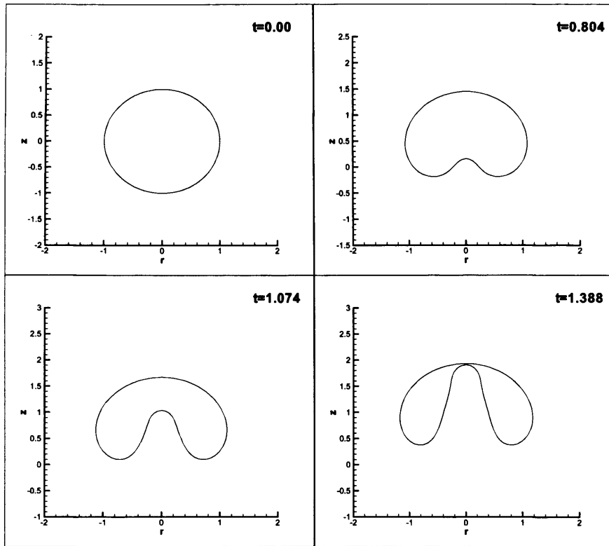
Figure 6.1: Bubble profiles at select times during ascent for Re = \infty and E\ddot{o} = 106 .
