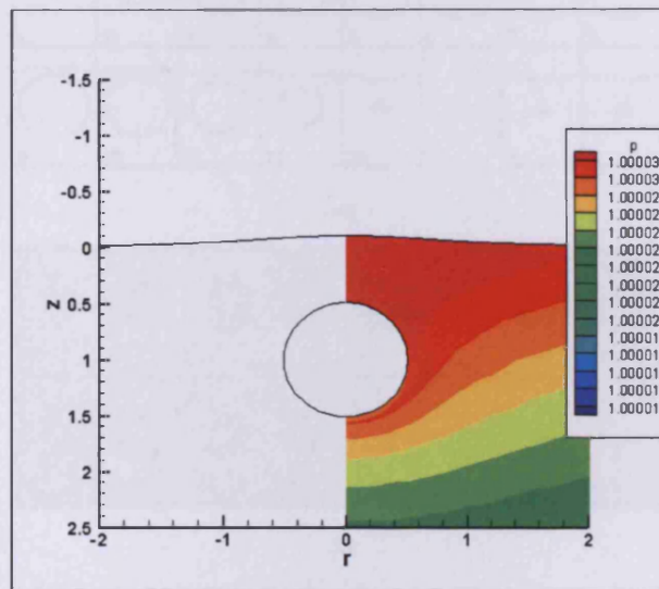
Figure 5.38: Pressure contours and velocity vectors at t = 17.6 with De = 0.5 , Re = 1.0 ( h = 1.0 ).
