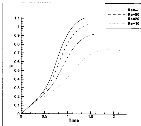
Figure 6.6: Evolution of the rise velocity for a selection of Reynolds numbers with E\ddot{o} = 106 .
