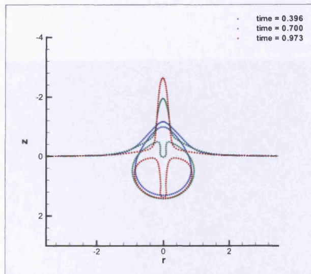
Figure 5.5: Bubble and free surface shapes for an inviscid fluid at h = 0.5 . Different colours indicate different instances in time.
