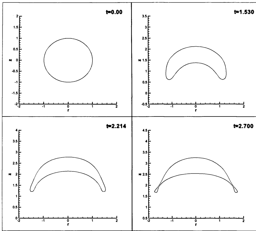
Figure 6.2: Bubble profiles at select times during ascent for Re = \infty and E\ddot{o} = 6.6 .
