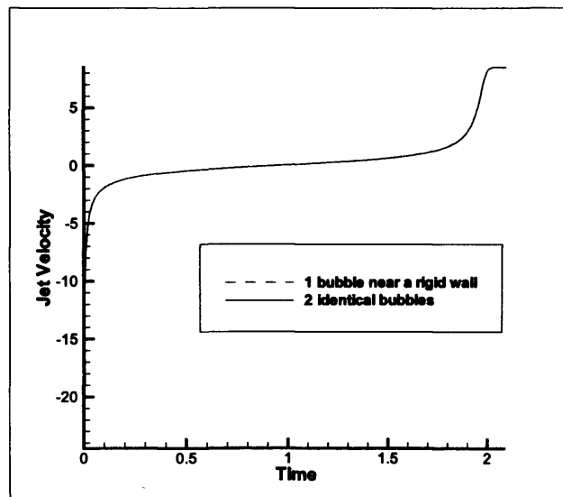
Figure 4.2: Jet velocities for a bubble near a rigid wall and one bubble near an identical bubble
