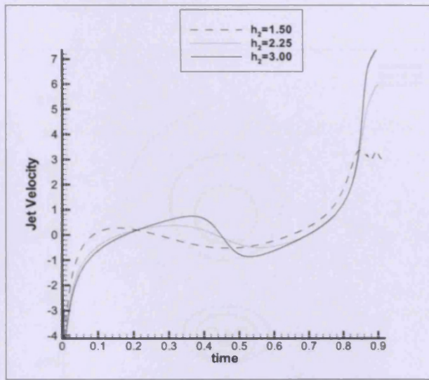
Figure 4.28: Jet velocities in B_1 at h_1 = 0.5 , for varying h_2 ( De = 1 , Re = 2 ).
