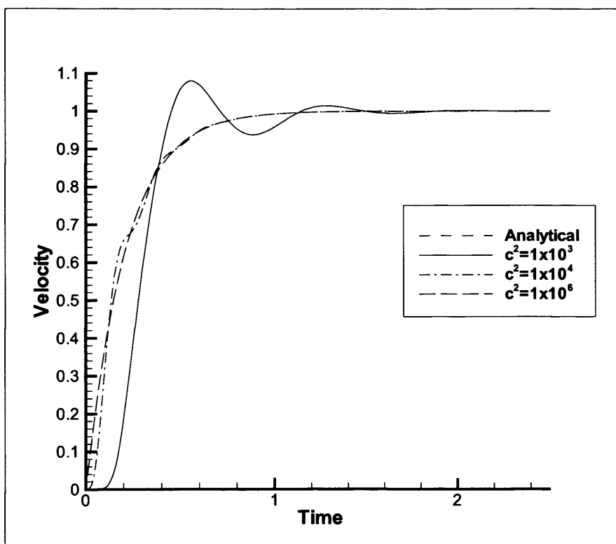
Figure 7.8: Incompressible analytical and compressible numerical solutions for velocity u for transient Poiseuille flow. By increasing the speed of sound the compressible solutions tend towards the incompressible solution. The channel length in this case is L = 10 .
