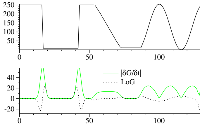
Fig. 9. A one dimensional signal (above), and responses of convolution by a LoG and \frac{\partial G}{\partial t} (below).
