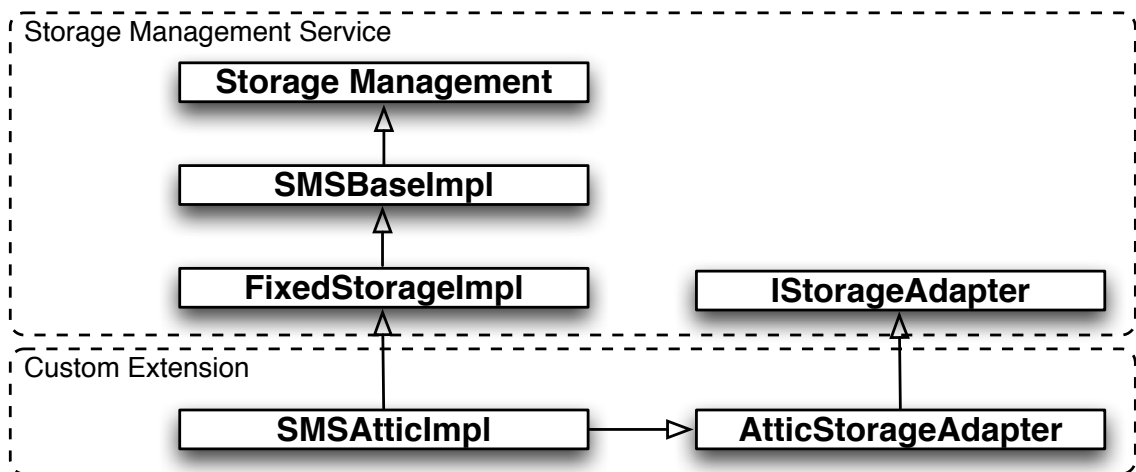
Figure 5.11: UNICORE Storage Adapter Implementation — shows a rough class diagram in which the two classes at the lower end contain the adapter functionality of a UNICORE Storage Service.
