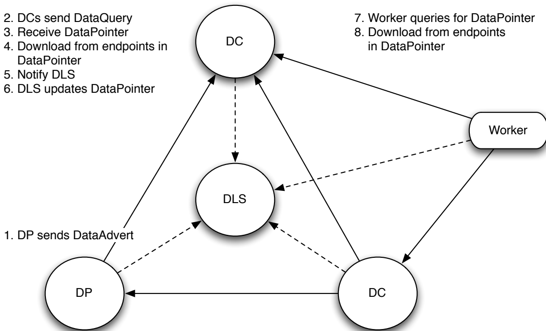
Figure 5.2: Attic Protocol Workflow.
