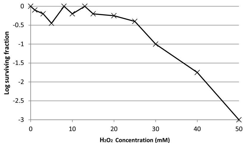
Figure 4.18: Log 10 surviving fraction of wild-type E. coli K12 culture after 15 min exposure to various hydrogen peroxide concentrations. . Adapted from Imlay & Linn (1986).
