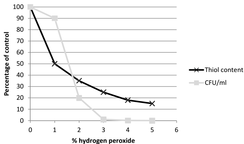
Figure 3.26: Expected relationship between hydrogen peroxide concentration and thiol content/ CFU/mL if thiol oxidation was major mechanism of bactericidal action of hydrogen peroxide.
