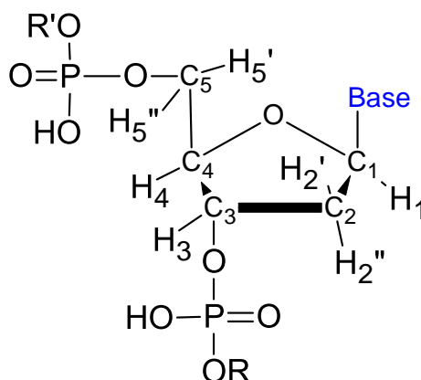
Figure 4.1: Diagram of the DNA sugar moiety enumerating the positions of the carbon and hydrogen atoms.
