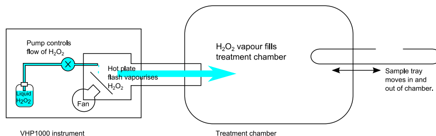
Figure 2.1: Schematic showing VHP1000 vapourised hydrogen peroxide treatment system.
