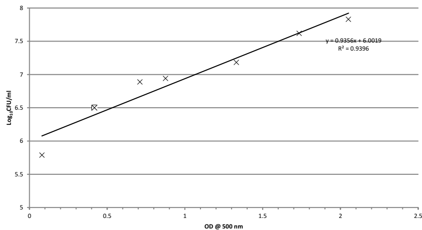
Figure 2.2: A500 (x axis) vs. \log_{10} CFU/mL showing linear trendline and equation.
