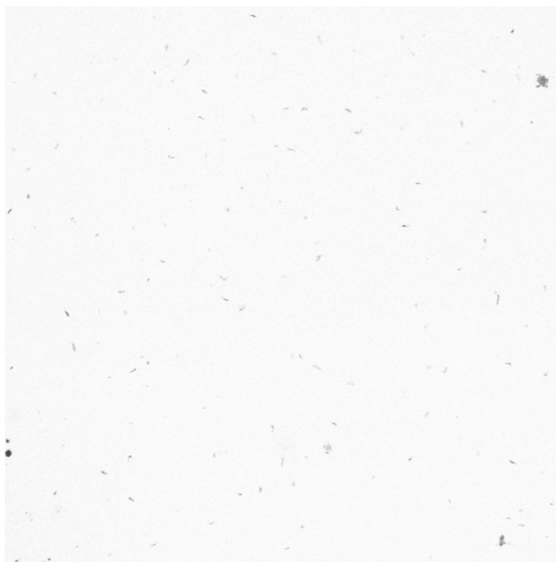
Figure 4.3: Acridine orange stained Comet assay image from control sample (original image converted to grey scale and inverted).
