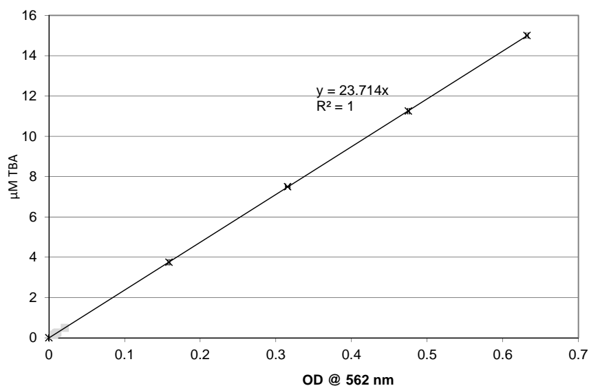
Figure 5.3: Standard curve for the aqueous phase of the two-phase TBARS assay. Test and control sample values are shown in grey.
