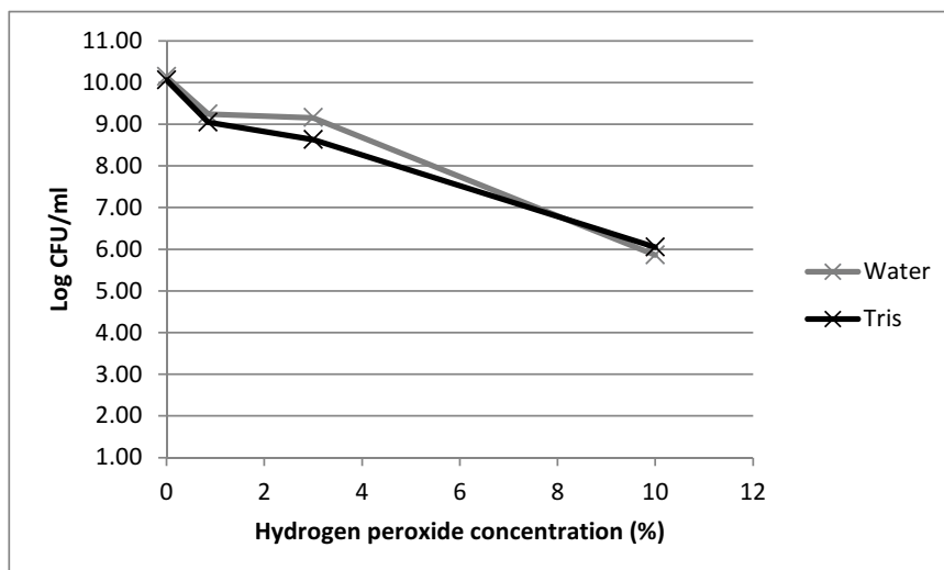
Figure 2.12: Reduction in \log_{10} CFU/mL E. coli in suspensions exposed to increasing concentrations of hydrogen peroxide in water or Tris buffer.
