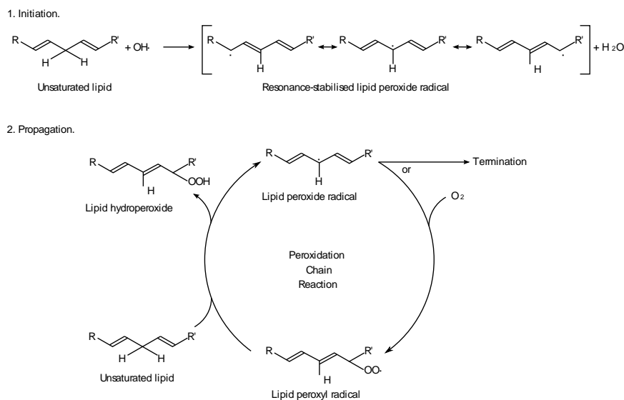
Figure 5.1: Summary of lipid peroxidation chain reaction.
