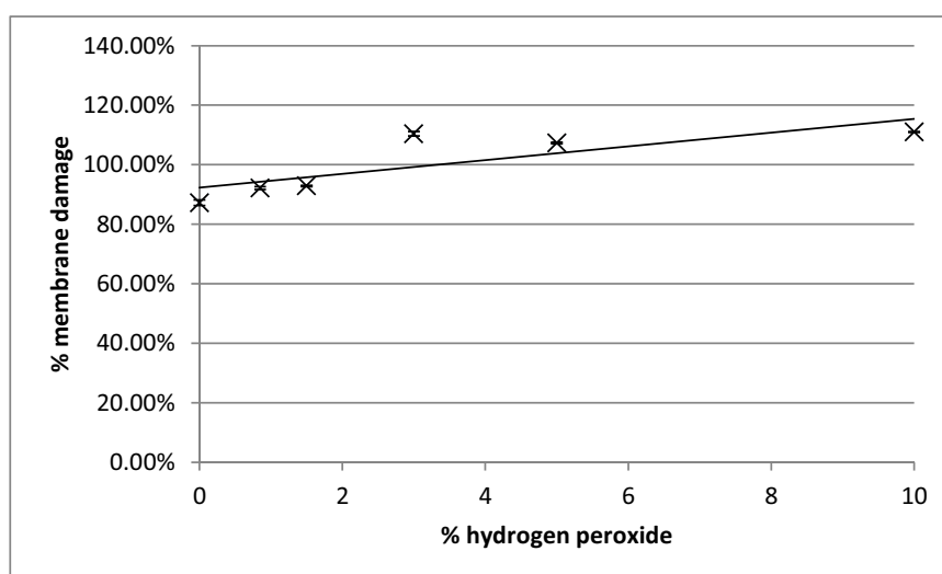
Figure 5.6: Mean percentage of membrane damaged cells from E. coli suspensions treated with increasing concentrations of liquid hydrogen peroxide as assayed using the Baclight LIVE/DEAD stain kit.
