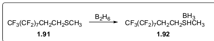
Scheme 1.32
