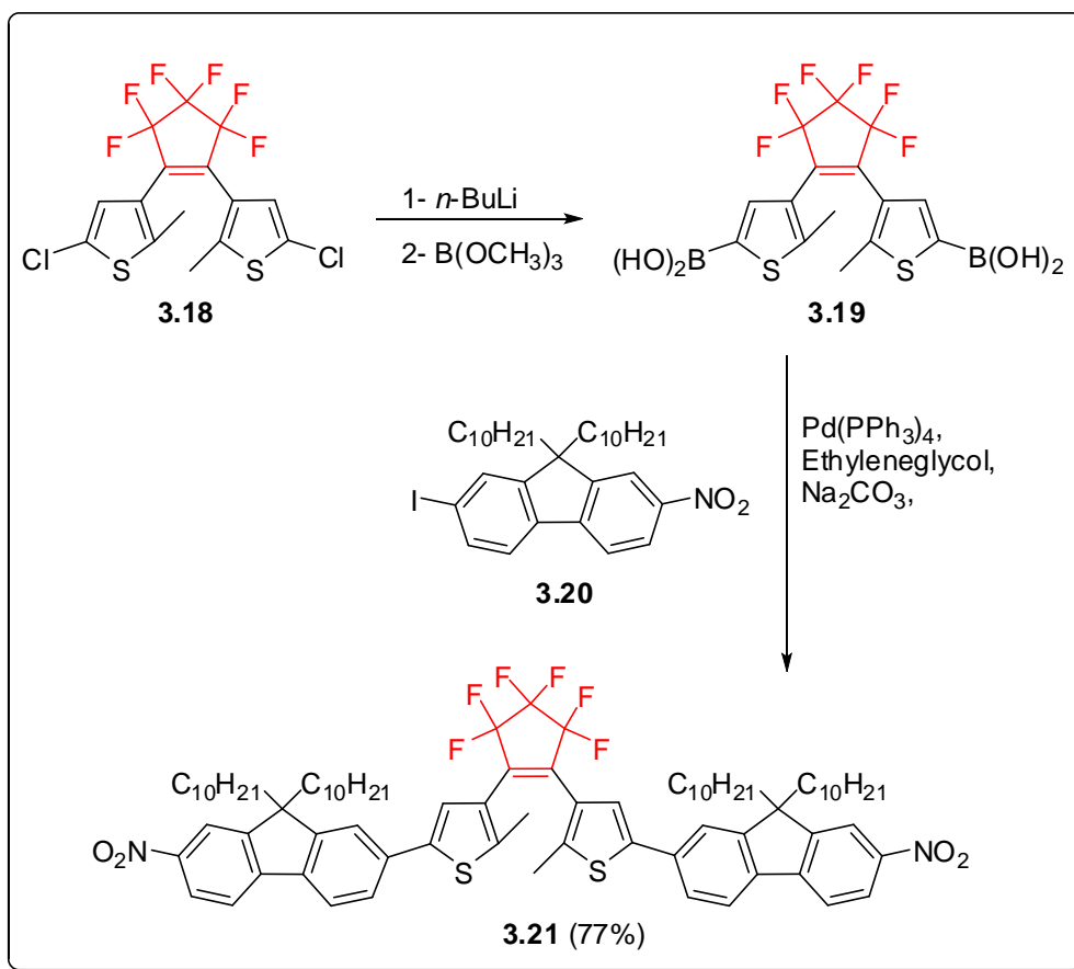
Scheme 3.7
