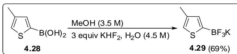
Scheme 4.11
