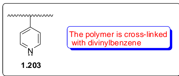
Figure 1.5: Cross-linked poly(4-vinylpyridine)
