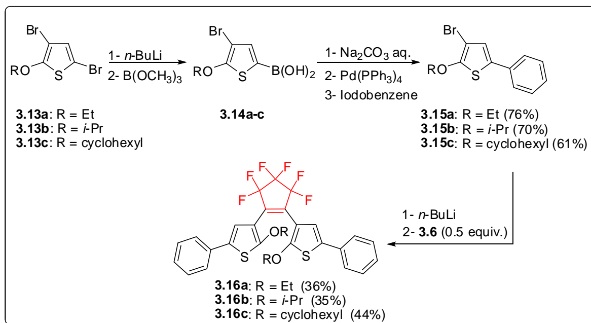
Scheme 3.5
