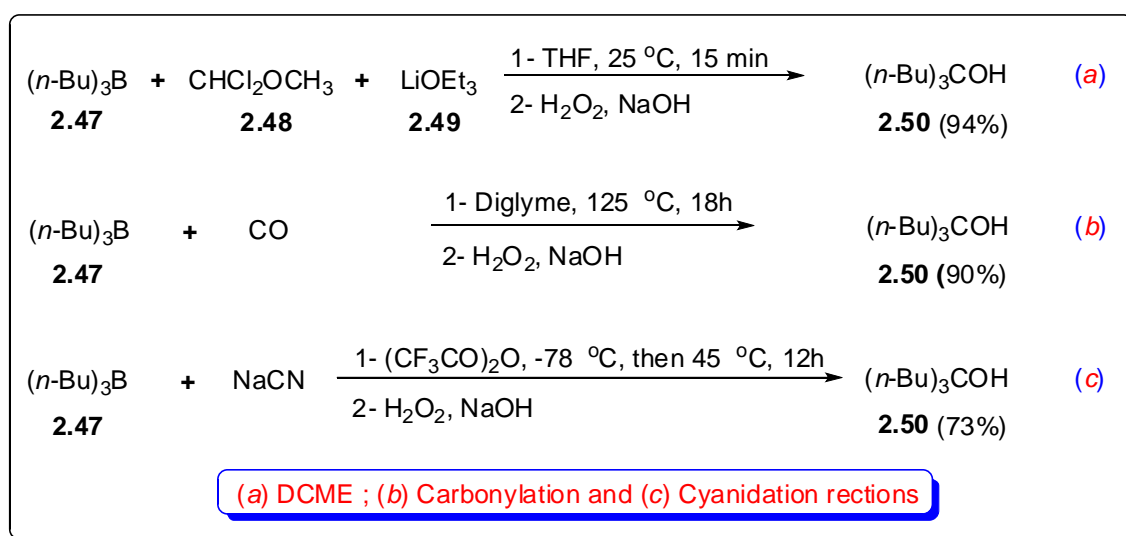
Scheme 2.19
