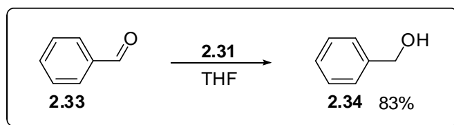
Scheme 2.15
