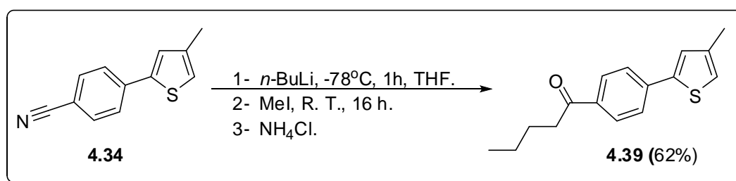
Scheme 4.17
