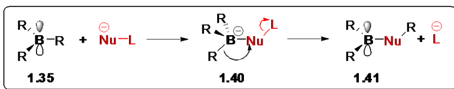
Scheme 1.16
