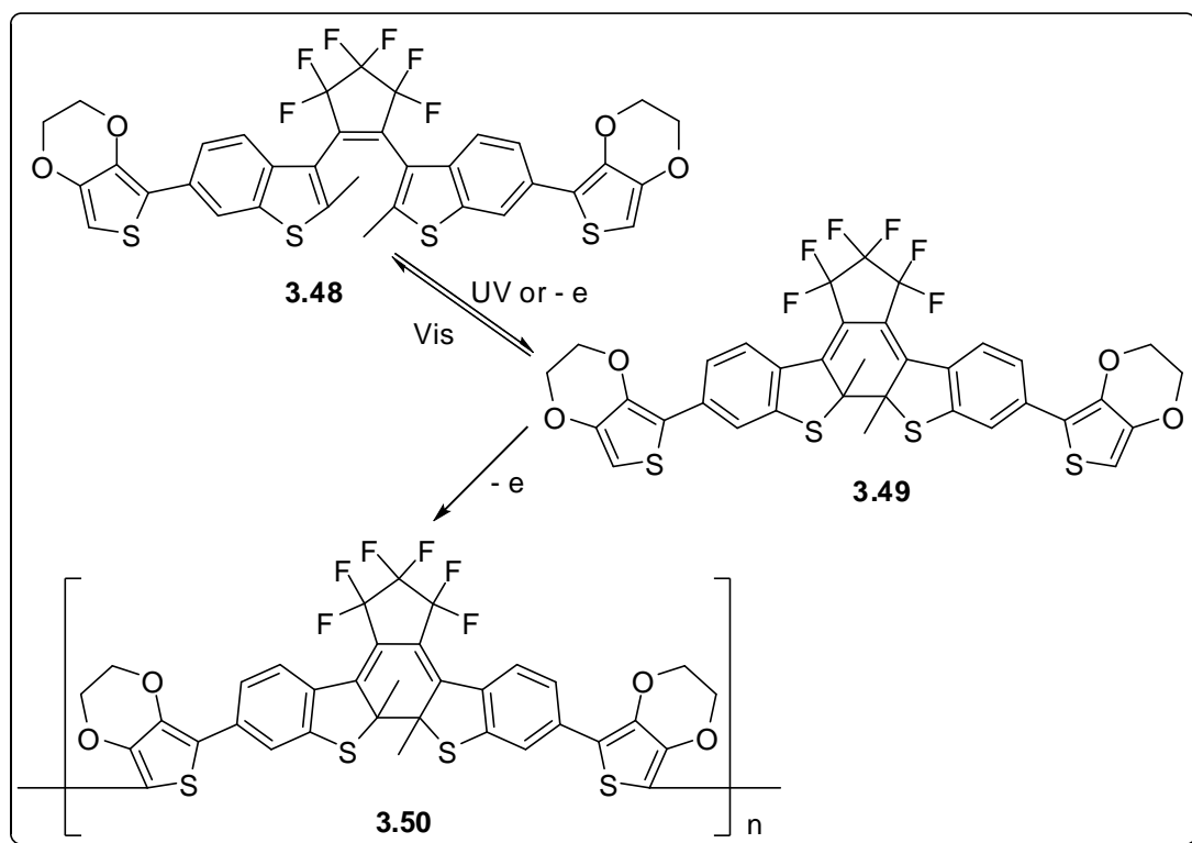
Scheme 3.16
