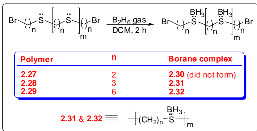
Scheme 2.13
