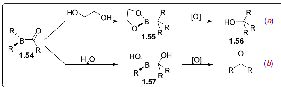
Scheme 1.22
