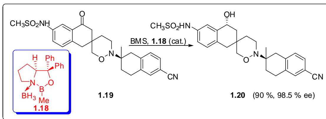
Scheme 1.8
