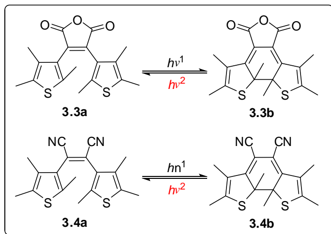
Scheme 3.2
