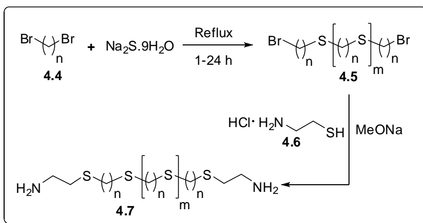
Scheme 4.2
