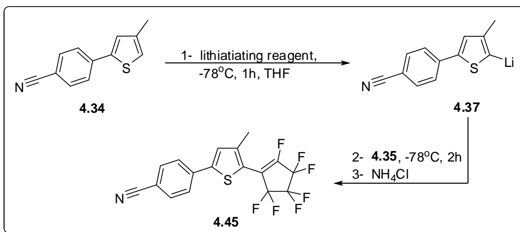
Scheme 4.15
