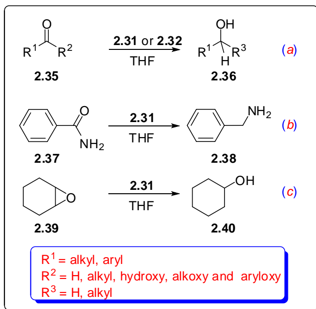
Scheme 2.16
