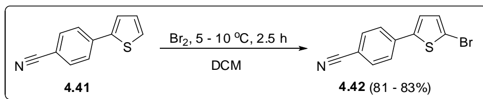
Scheme 4.19
