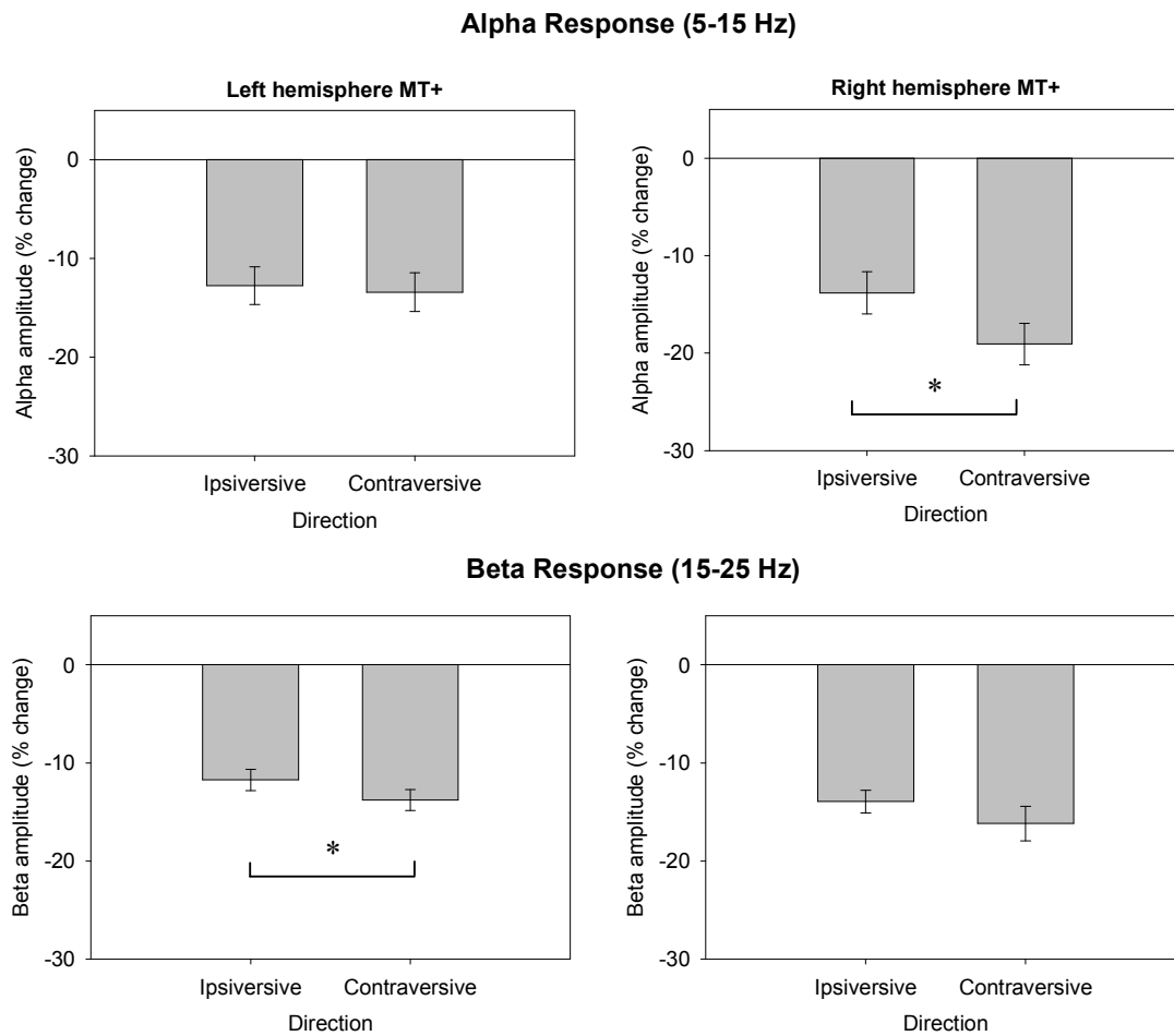
Figure 38. Mean alpha and beta suppression averaged across all velocities for ipsi- versus contraversive pursuit directions from left and right hemisphere MT+, with \pm 1 standard error bars.
