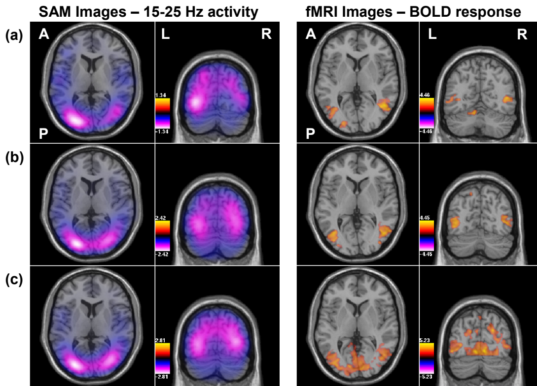
Figure 13. Group results from MEG and fMRI in all three conditions.
