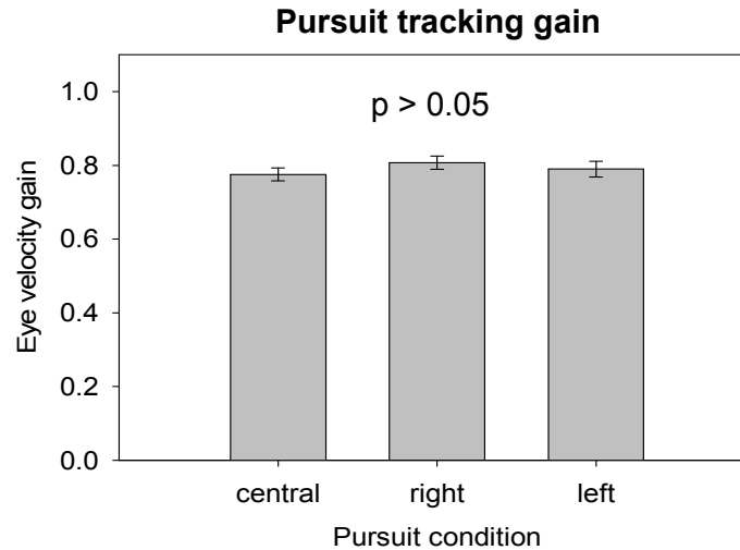
Figure 26. Eye movement velocity gain for the excursive pursuit experiment.
