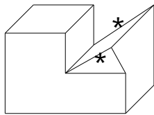
Figure 66. Edges Not Parallel in 3D
