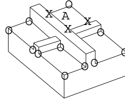
Figure 70. Coplanar Vertices
