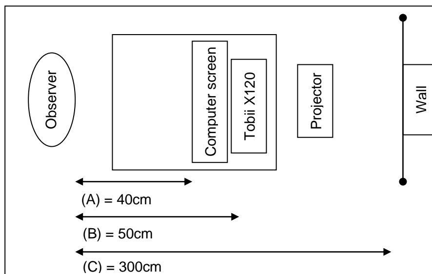
Figure 3.17 Schematic diagram of the set up for the Tobii X120, showing the distance from the observer to: the eye tracker (B), the stimulus on the computer screen (A) and the stimulus on the wall projection (C).
