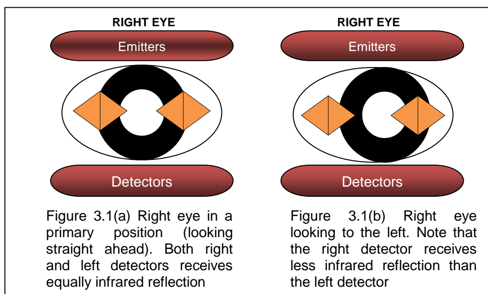
Figure 3.1 Graphical drawings illustrating the principle of eye movement detection using the infrared emitters and detectors of the Skalar IRIS.
