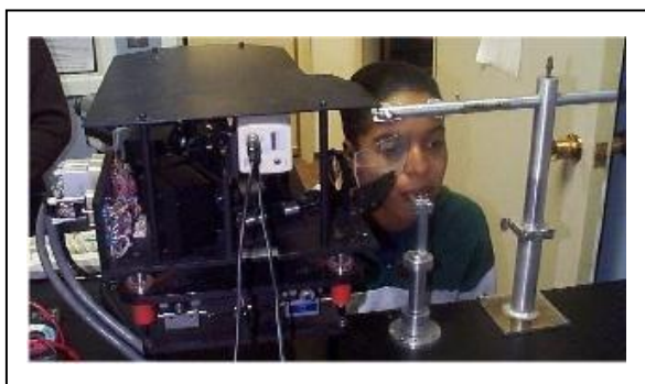
Figure 2.20 Dual Purkinje Image eye tracker (Fourward Technologies, Inc. 2001).
