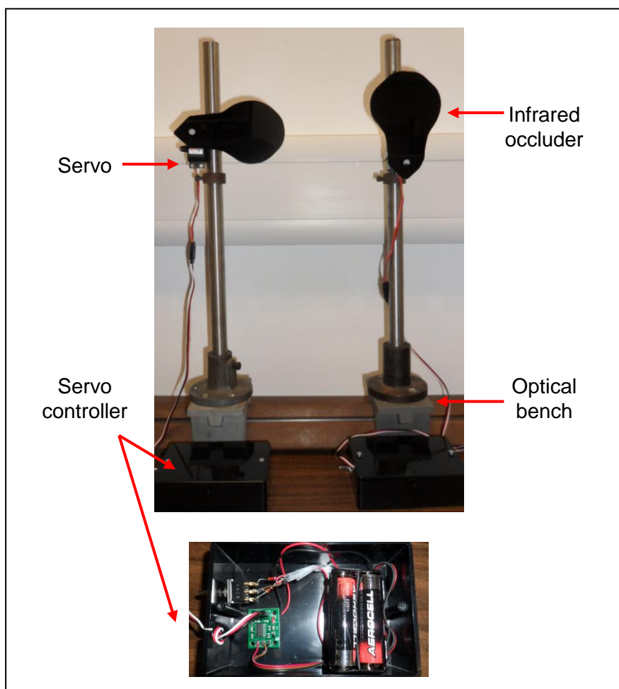
Figure 3.15 Semi-automated occluder unit.
