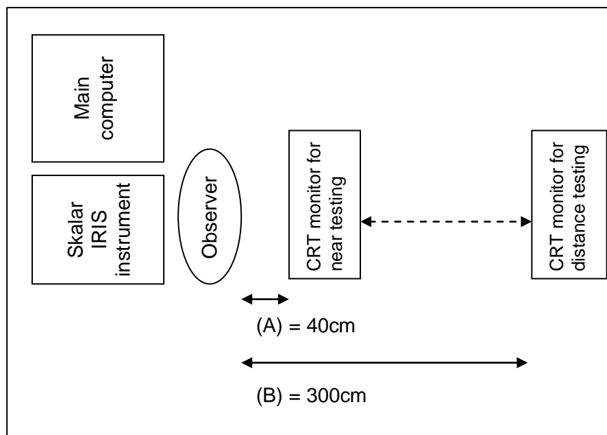
Figure 3.16 Schematic diagram of the set up for the Skalar IRIS eye tracker, showing the distance from the observer to the monitor screen for experiment at near (A) and at far (B).
