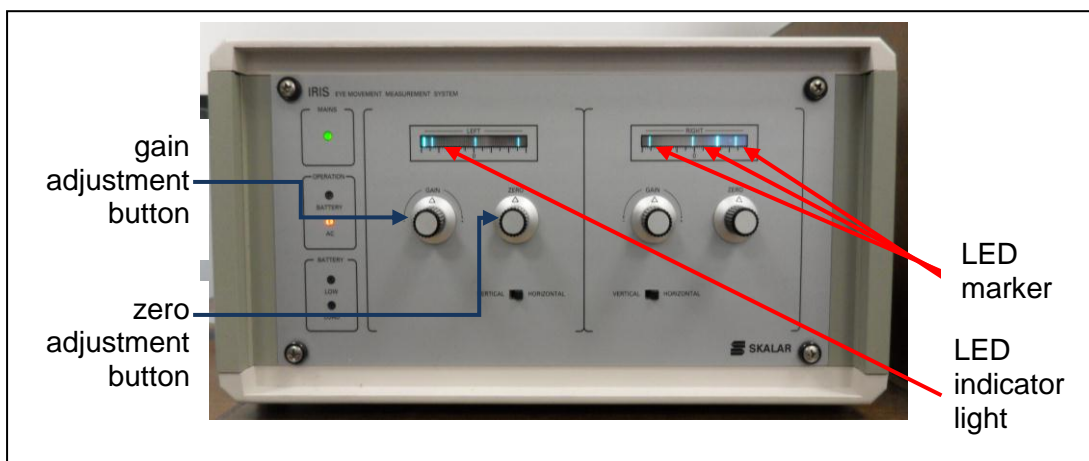
Figure 3.5 Close up control module showing the LED indicator lights, LED marker, gain and zero adjustment button.
