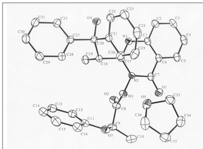
Figure 1 X-ray crystal structure of 13a with numbered crystallographic atoms
