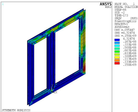
(c) Von Mises equivalent stress
