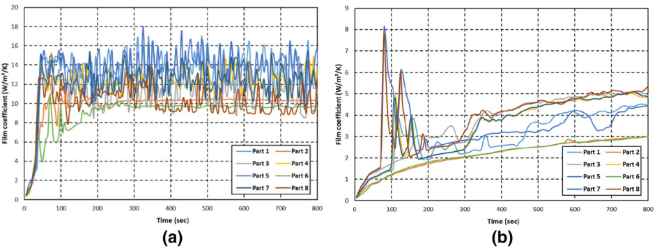
Figure 8. Evolution of the convective coefficient applied to the exposed (a) and un-exposed (b) faces for all sections of the window frame.
