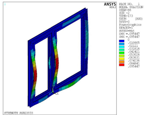
(b) Window deformation
