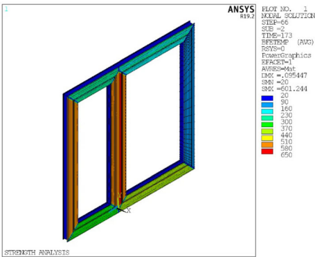
(a) Window temperature
