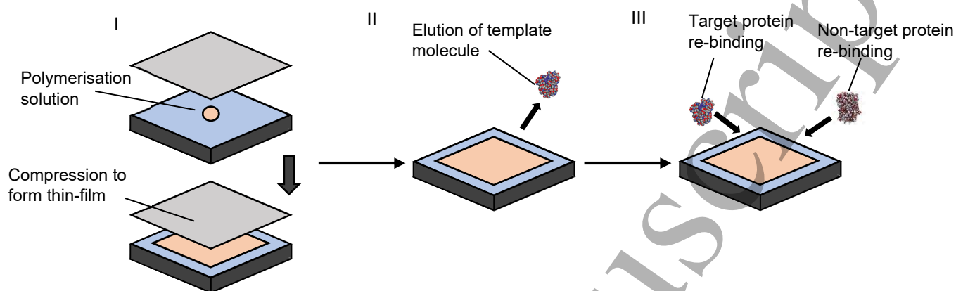
Figure 3. Schematic representation of the synthesis of the thin-sheet (2D) MIP: (I) Template contained polymerising solution placed on to Parafilm®, followed by compression using bronze weights, then polymerisation, to form thin-sheets. (II) Elution of templates molecule with 10% (w/v):10% (v/v) SDS:AcOH eluent, for two hours, followed by five water washes. (III) The reloading of target molecule and/or non-specific target to the MIPs.
