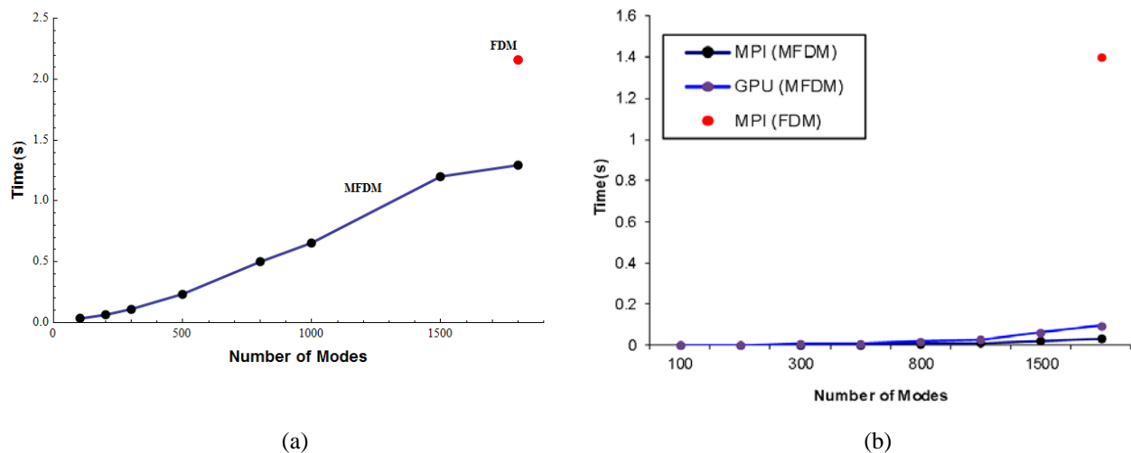
Fig. 11. (a) Serial MFDM ( M2 ) performance versus the number of used modes and serial FDM ( M1 ) performance (red point); (b) Parallel MPI- and CUDA- based MFDMs ( M4 and M5 ) performance vs. the number of used modes and MPI-based FDM performance ( M3 ) (red point)
