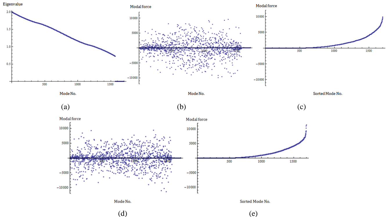
Fig. 3. (a) Eigenvalues, (b) modal force (explosive source) , (c) sorted modal force (explosive source), (d) modal force (for double couple) and (e) sorted modal force (for double couple) in the homogeneous case
