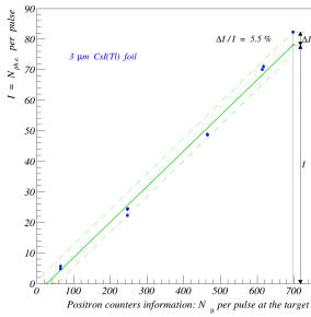
Figure 3. Linearity of the 3 \mu\text{m} foil.
