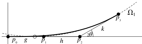
Figure 5. A J-shaped transition curve in normalized form.
