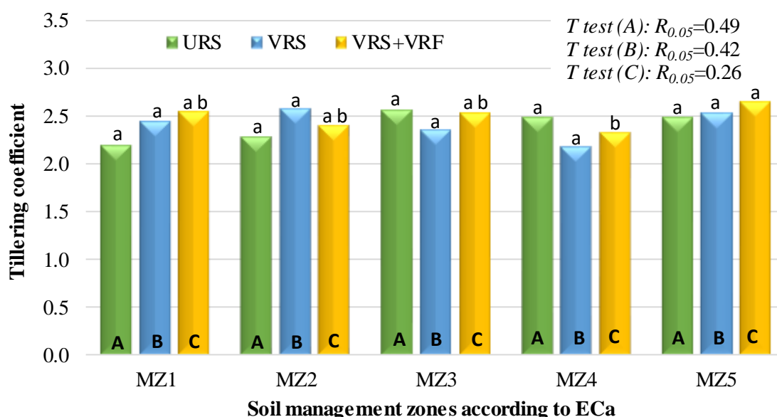
Fig. 5. Effect of precision seeding on winter wheat tillingering coefficient in different soil management zones
