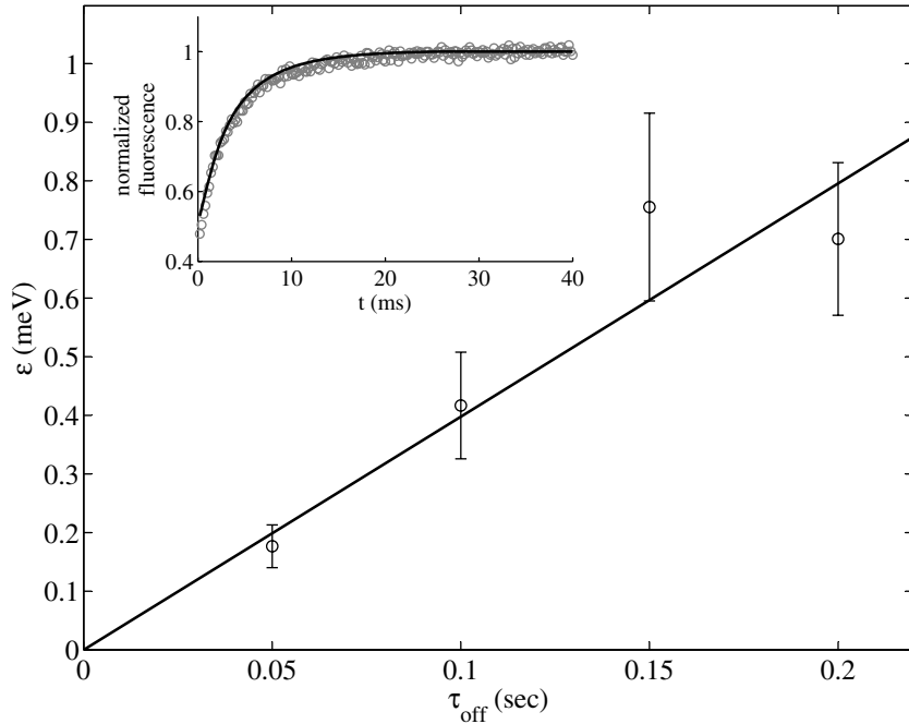
Figure 2. Scaled energy \epsilon as a function of ion heating time \tau_{\text{off}} in Doppler recooling experiments. As expected, the energy of the ion scales linearly with heating time and a linear fit constrained through the origin is used to derive the rate of change d\epsilon/dt , in this case 4.0 \pm 0.3 \text{ meV s}^{-1} . Uncertainties in the ion energy are determined by uncertainty in the exact value of the detuning used for the measurement. Inset: a typical Doppler recooling curve for one value of \tau_{\text{off}} with fluorescence as a function of time, and fitted (solid line) according to the procedure described in [41]. Time zero in the inset corresponds to the onset of recooling, i.e. turning on the repump laser at 866 nm.
