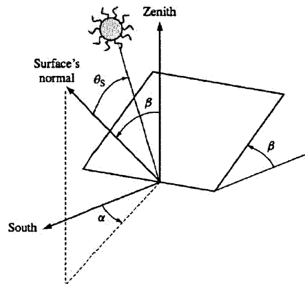
Figure II.2 Receiver position (slope \beta and azimuth \alpha ) and sun's rays incidence angle \theta_s
