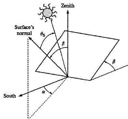
Figure II.1 Receiver position (slope \beta and azimuth \alpha ) and sun's rays incidence angle \theta_s Source: Luque and Hegedus 2003
