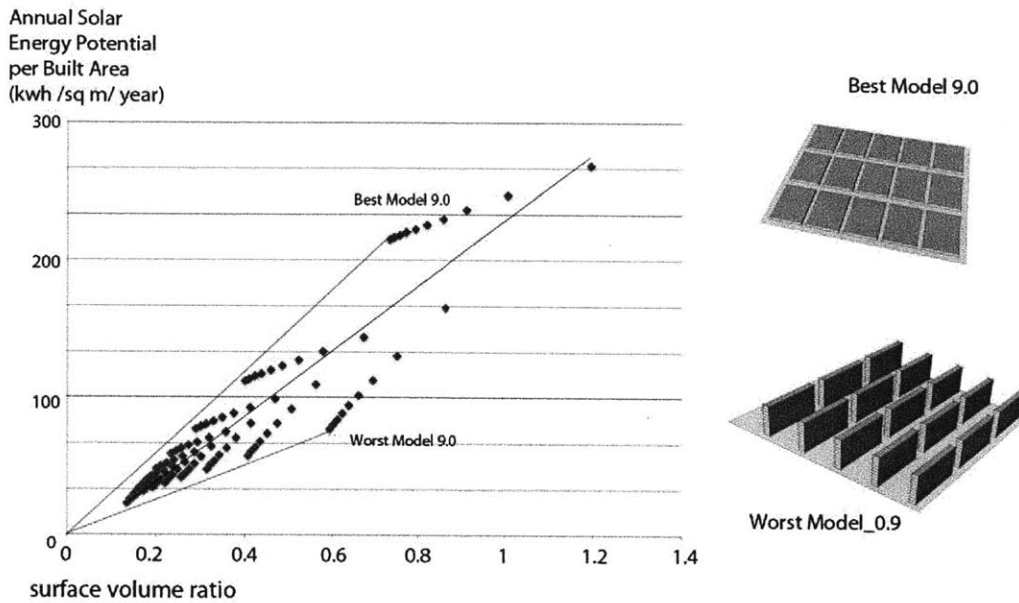
Figure 3.8 The relationship between energy yield and the surface area to volume ratio
