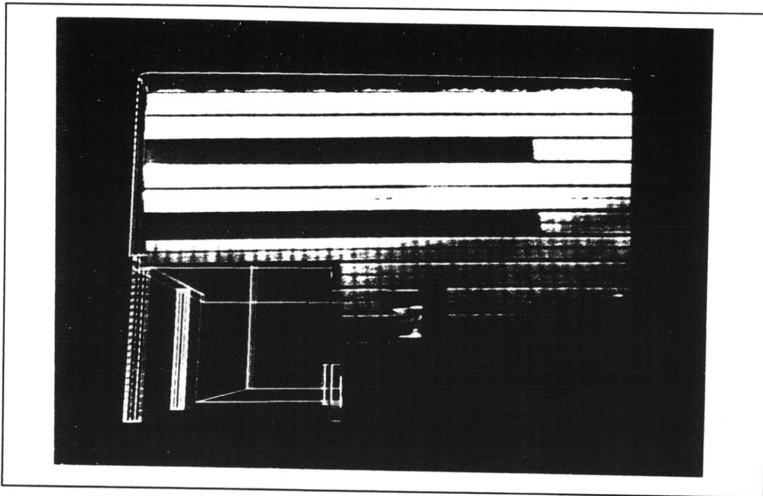
Figure 8: Registration error.
