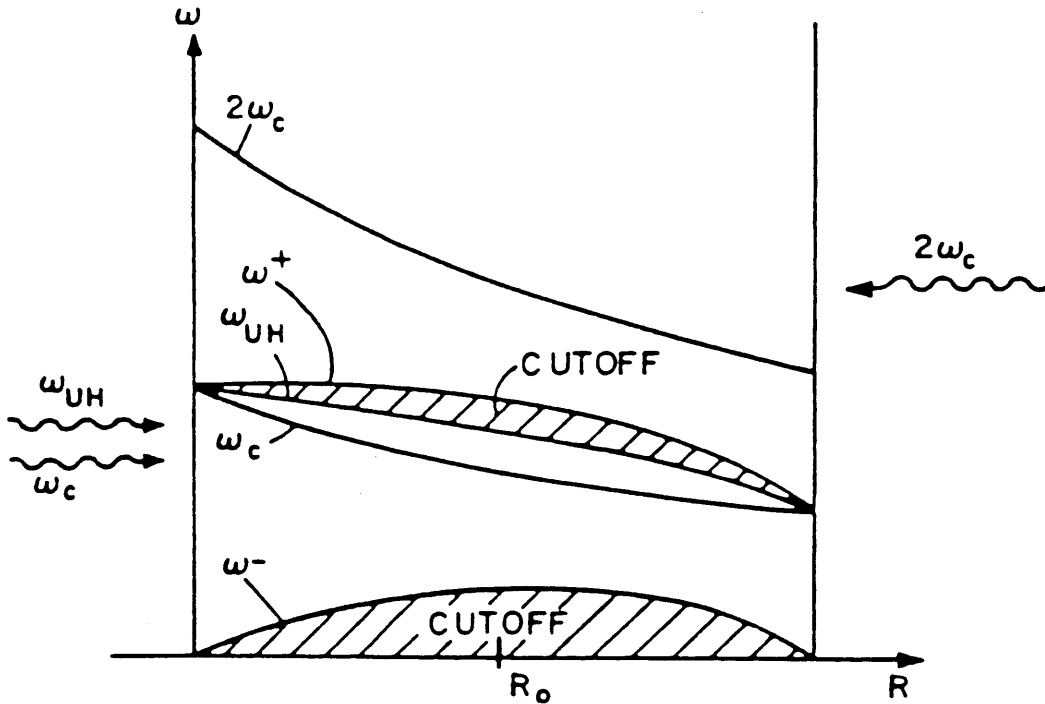
a) EXTRAORDINARY WAVE
