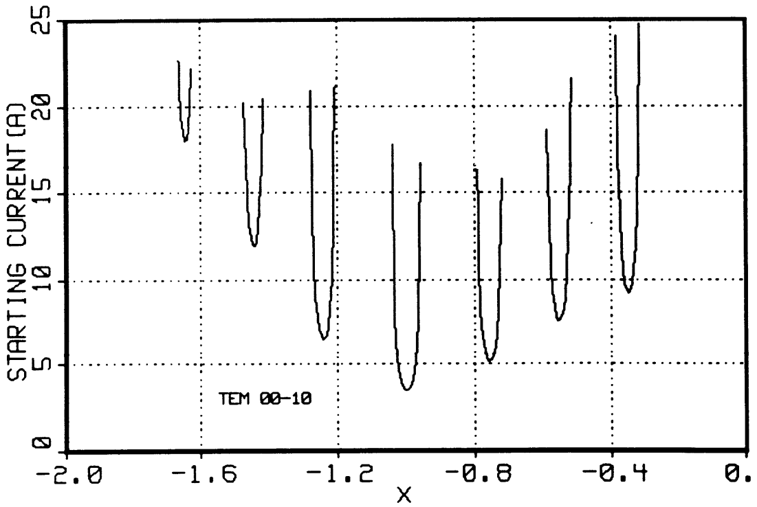
Figure 4.3(b): Characteristic Gain Curves for w/u = 2.5 and q = 10 .
