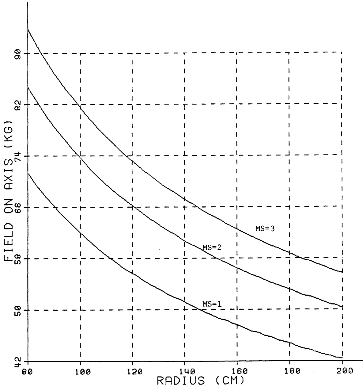
Figure 2.3 Minimum field as a function of the margin of safety. Temperature has been optimized according to Eq.(2.9)
