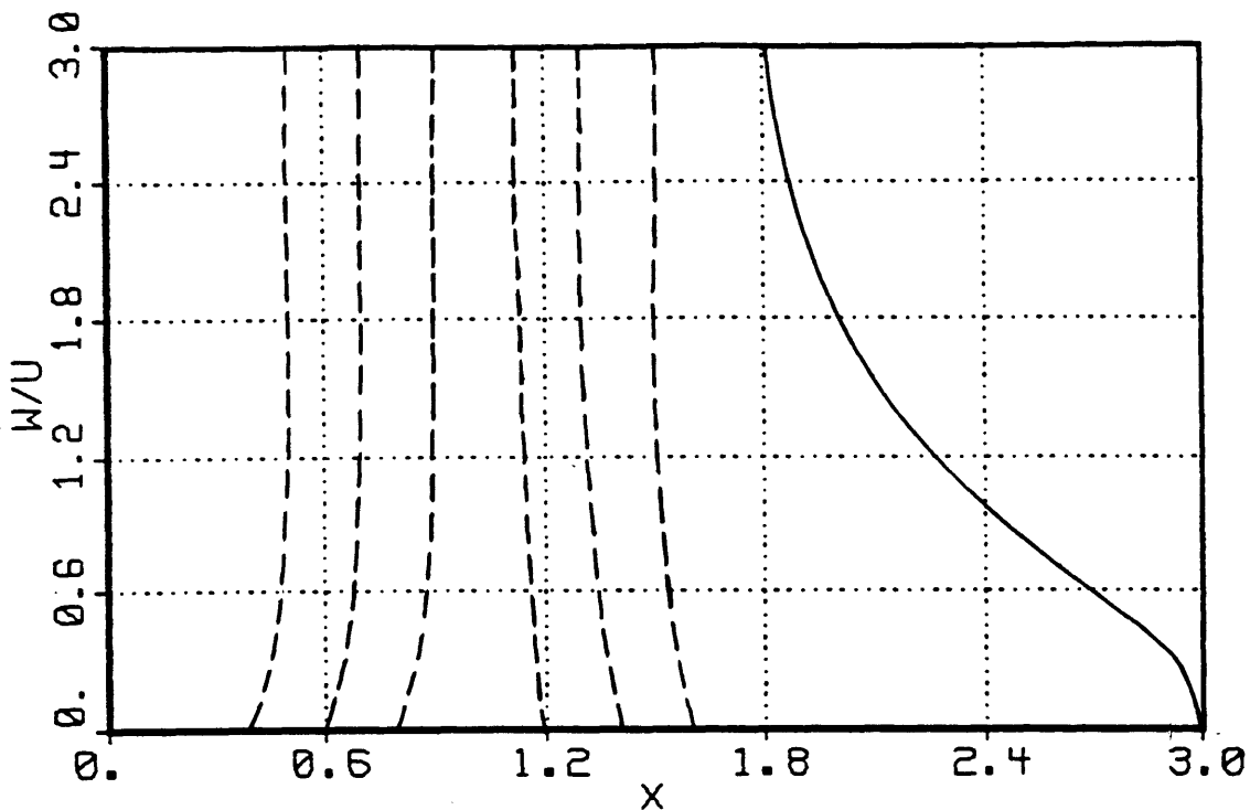
Figure 4.4(a): Minimum w/u for q = 1 (Solid) and q = 10 (Dash). \beta_{||} = 0.2 .
