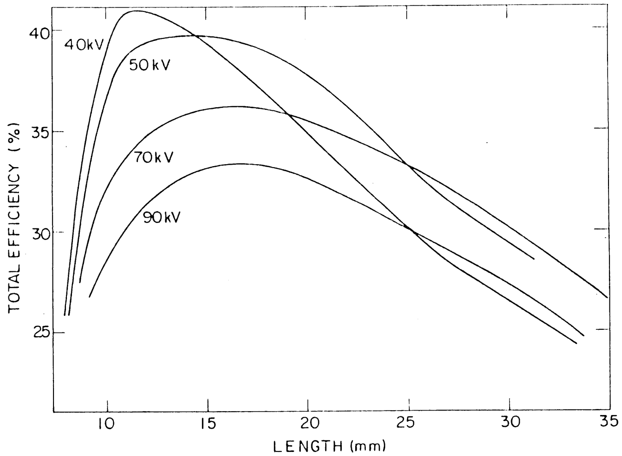
Fig. 5.3 Total Gyrotron Efficiency vs. Beam Voltage and Cavity Length.
