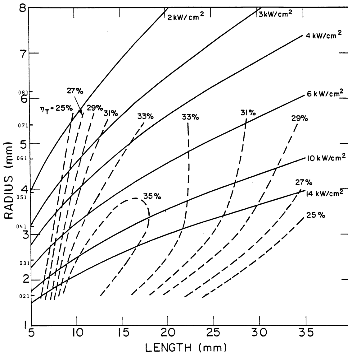
Fig. 5.8 Optimum Total Efficiency of 200 GHz, 100 kW Gyrotron with \beta_{\perp}/\beta_{\parallel} = 1.8 .
