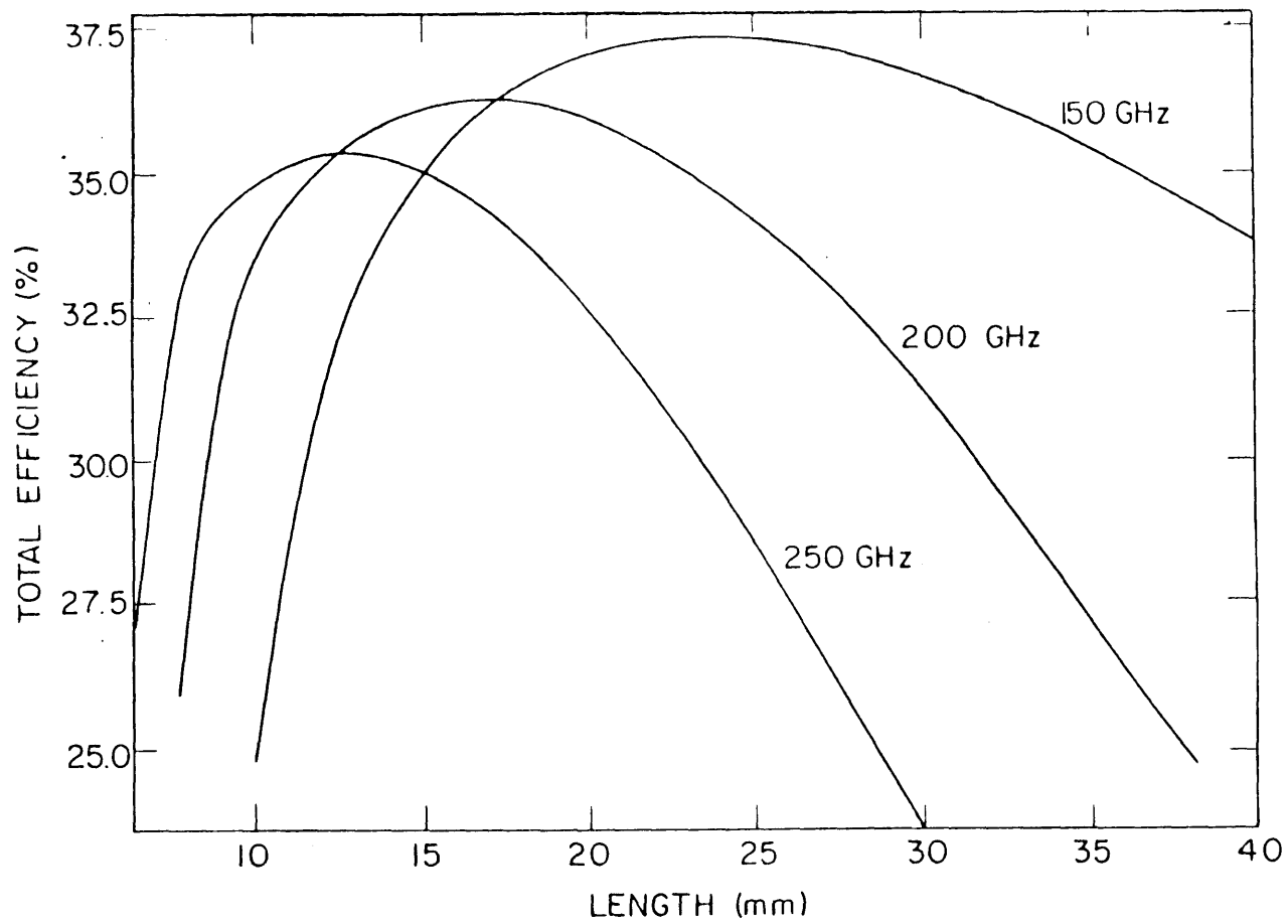
Fig. 5.2 Total Gyrotron Efficiency vs. Frequency and Cavity Length.
