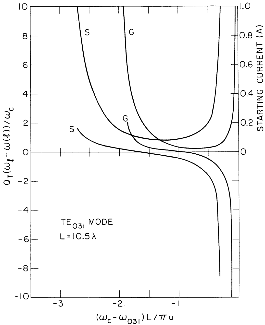
Figure 3.1 Comparison of the linear characteristics of an ECM with a sinusoidal (S) longitudinal RF field distribution with one having a Gaussian (G) profile. Upper curves represent the starting currents, while lower curves give the frequency detuning.
