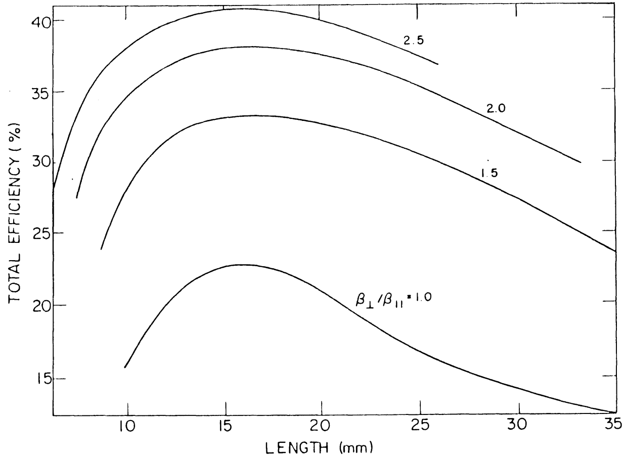
Fig. 5.4 Total Gyrotron Efficiency vs. Velocity Ratio and Cavity Length.
