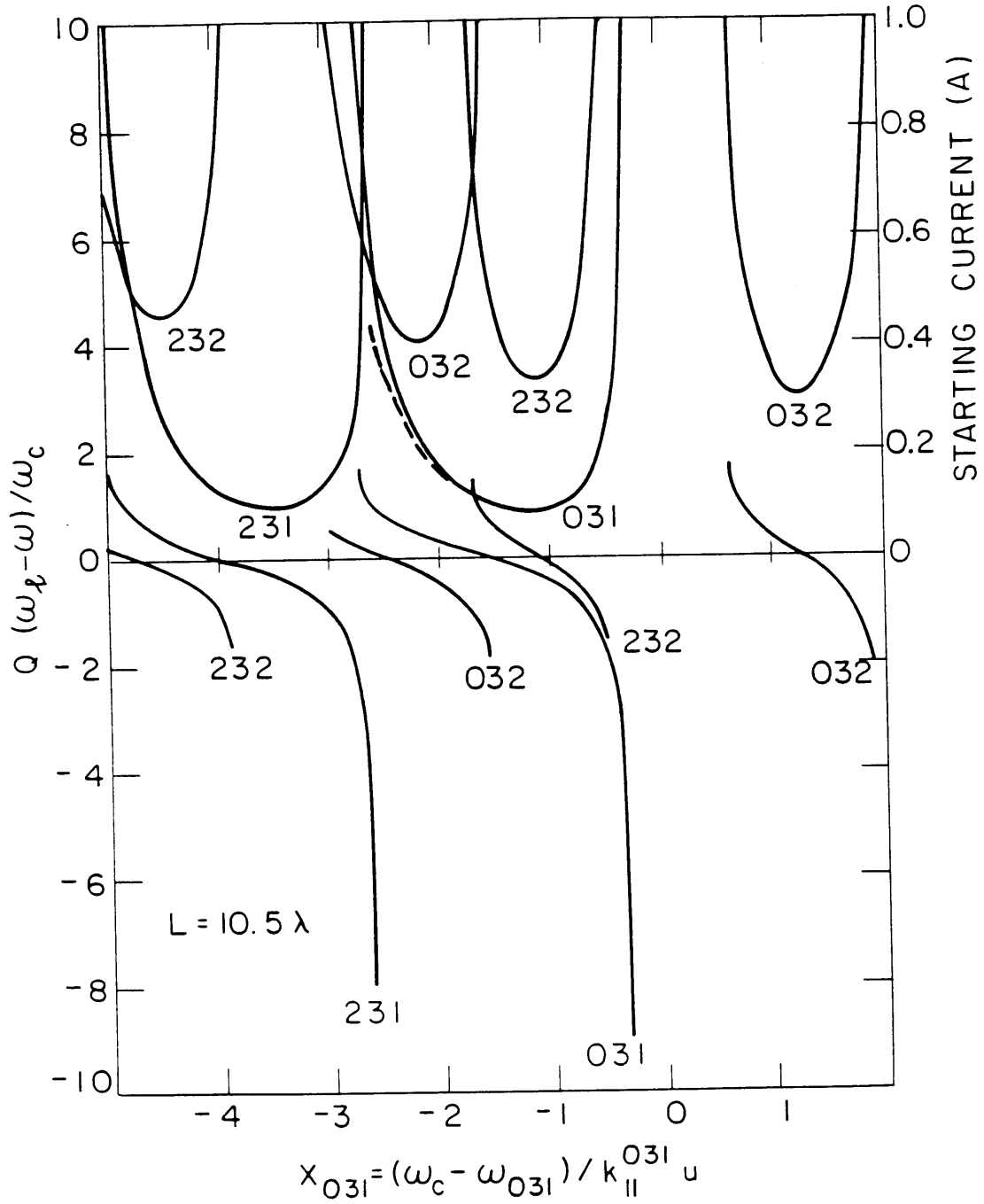
Figure 3.7 Starting current (upper curves) and detuning (lower curves) for the TE 03q and TE 23q modes. Dotted line is starting current if TE 031 and TE 032 oscillate simultaneously.
