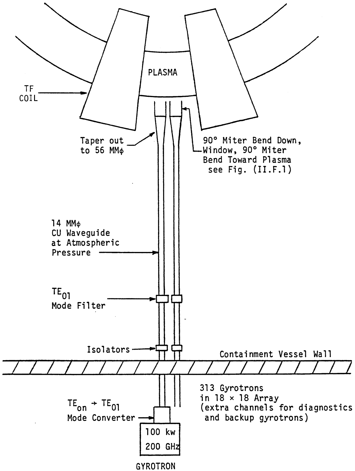
Fig. 5.11 ECRH POWER TRANSMISSION
