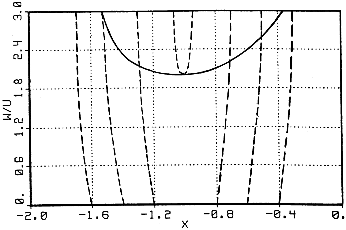
Figure 4.3(a): Minimum w/u for q=1 (Solid) and q=10 (Dash). \beta_{||} = 0.2 .
