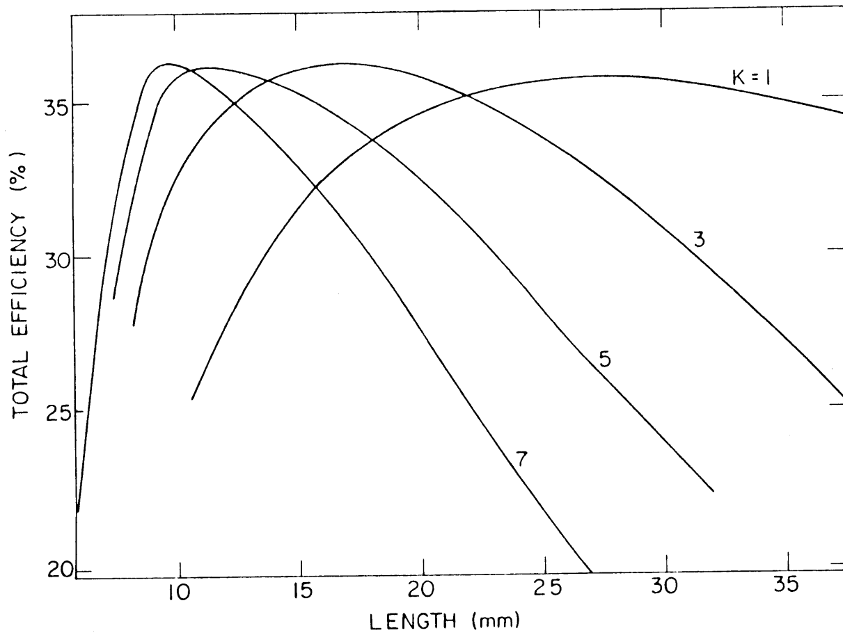
Fig. 5.5 Total Gyrotron Efficiency vs. the Coupling Factor K and Cavity Length.
