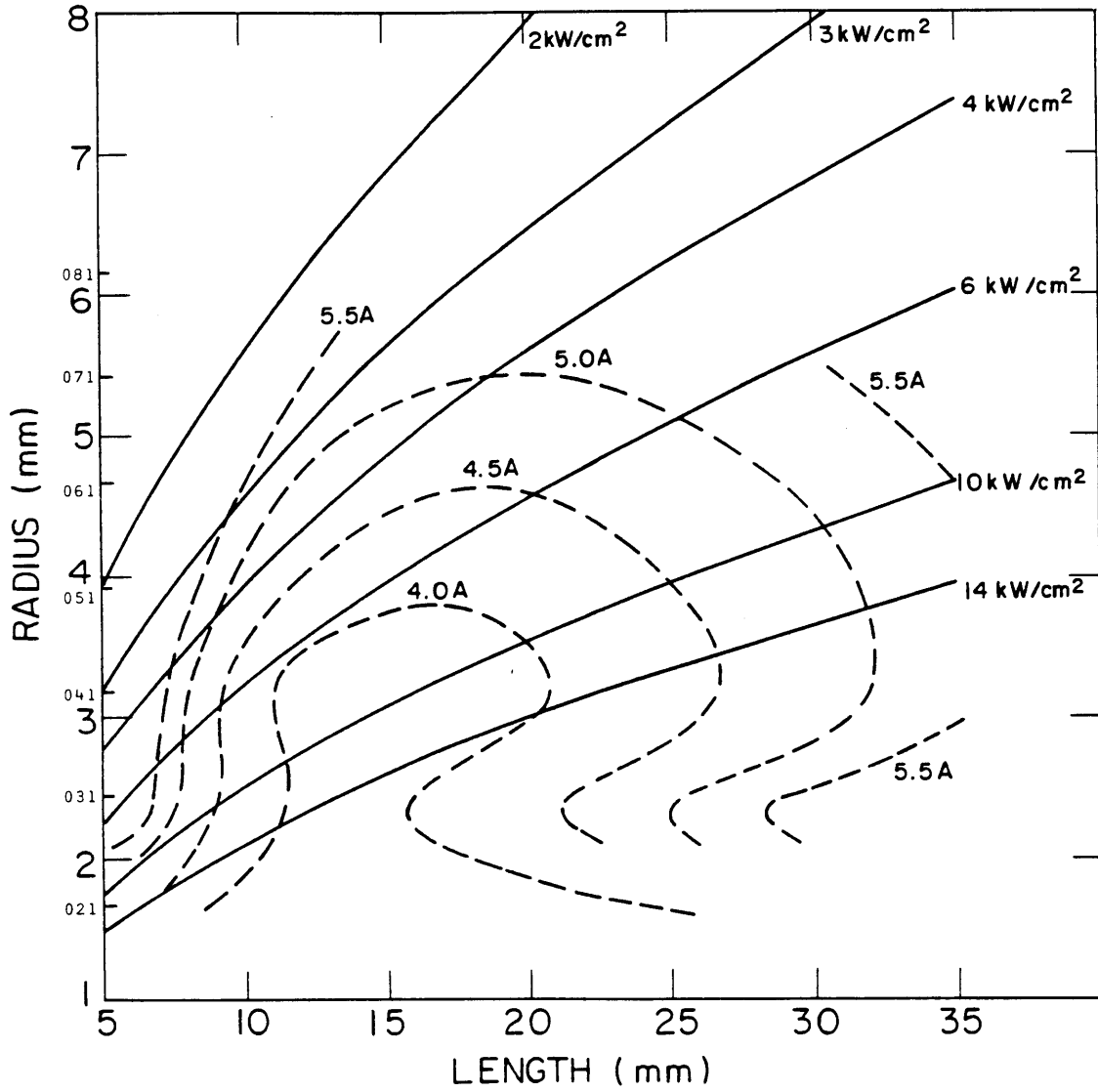
Fig. 5.9 Beam Currents Associated with Operating Conditions Shown in Fig. 5.8
