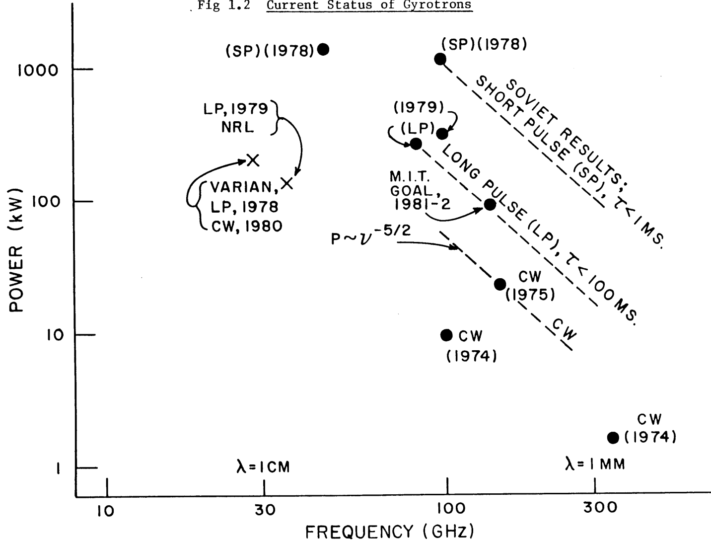
Fig 1.2 Current Status of Gyrotrons
