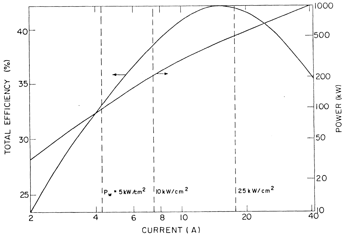
Fig. 5.10 Total Efficiency and Output Power vs. Beam Current. Also shown are Limits Imposed by Wall Heat Flux.
