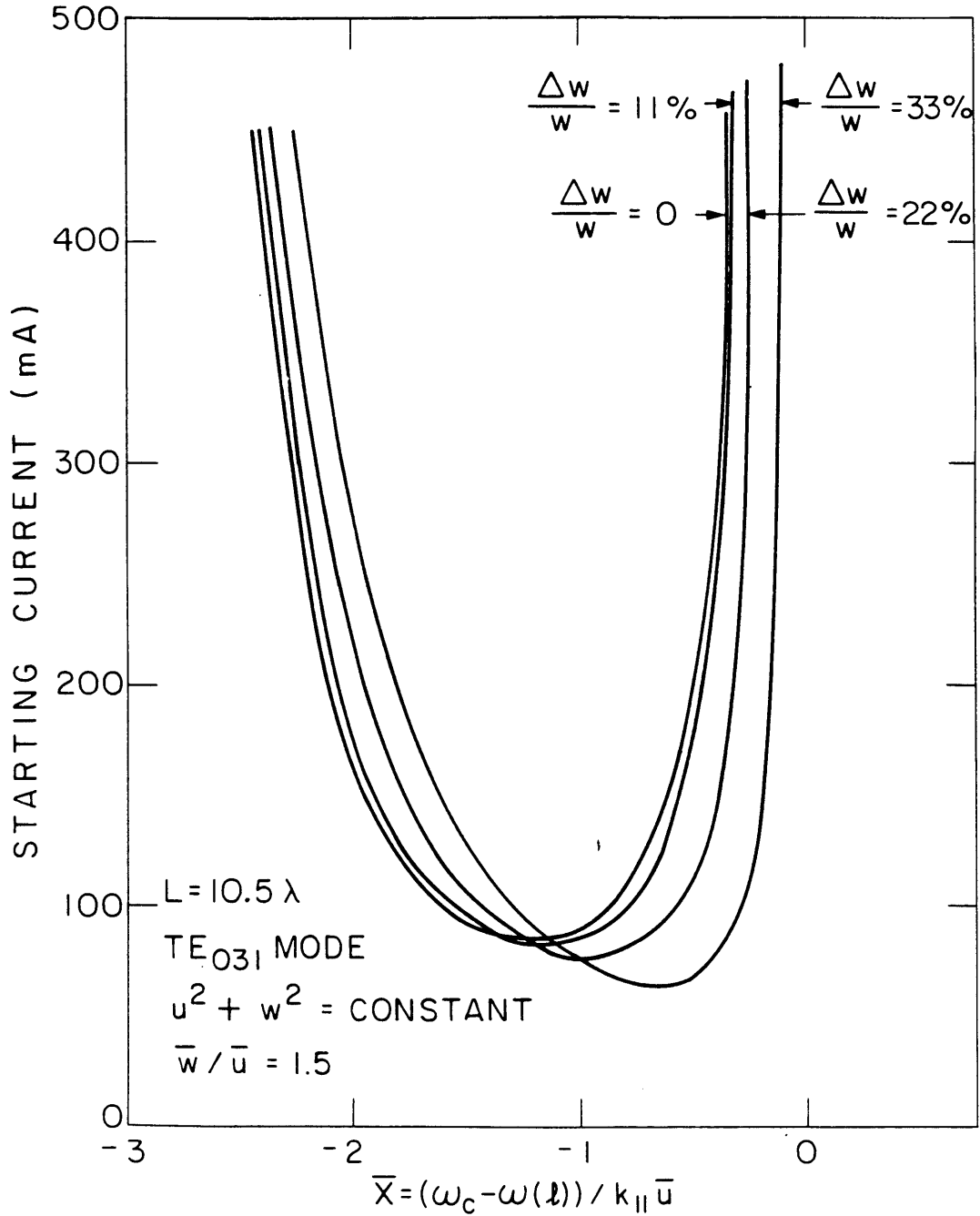
Figure 3.2 Dependence of the starting current on the velocity spread of the electron beam, \Delta w/w , for the TE_{031} mode. ECM has RF field with sinusoidal longitudinal profile, and same operating parameters as those given for Fig. 3.1
