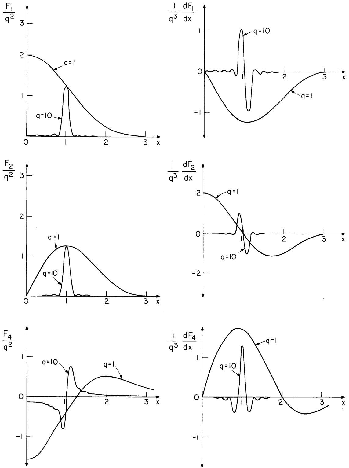
Figure 4.2 Gain Functions and Their Derivatives
