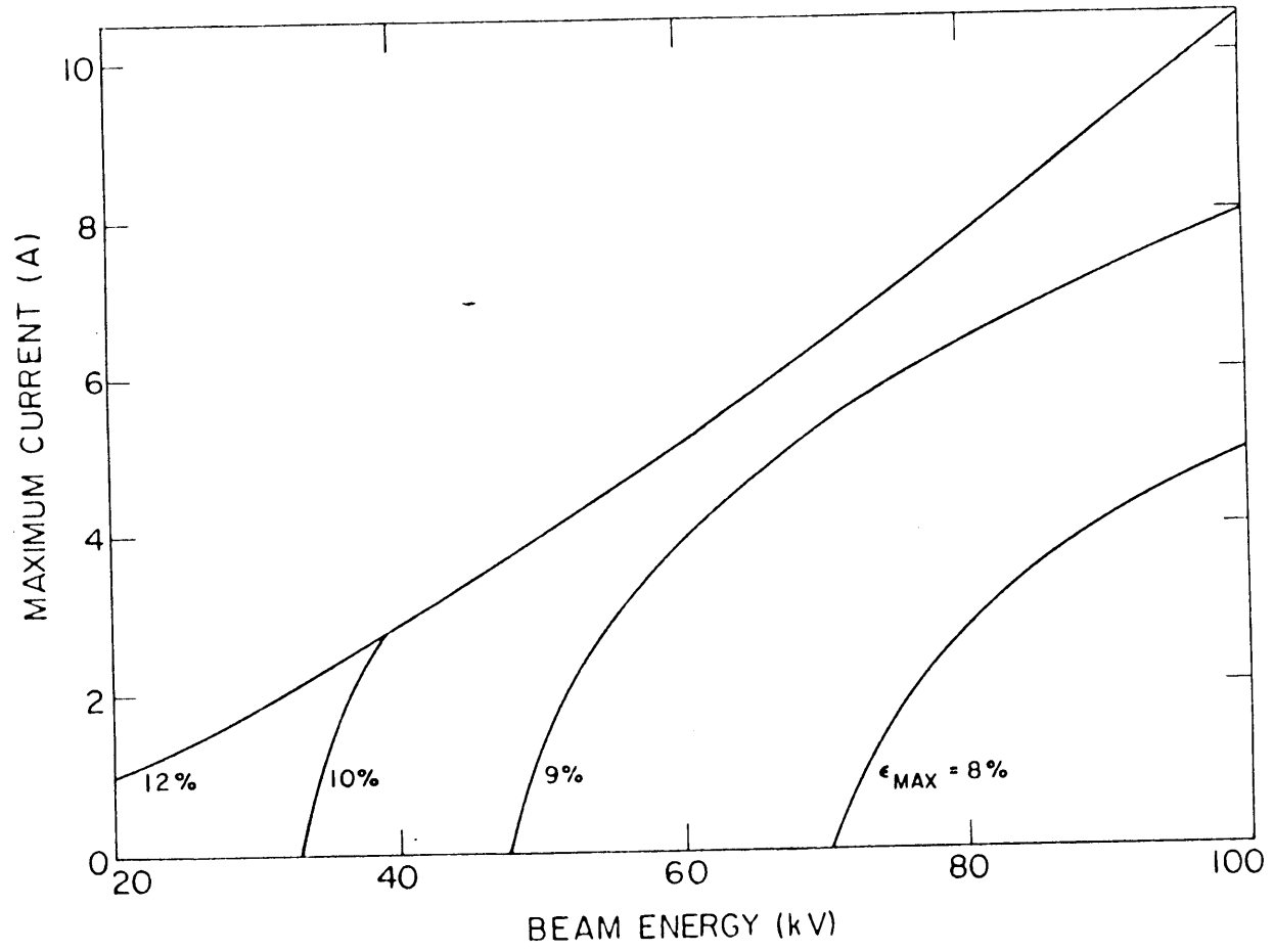
Fig. 5.6 Maximum Current Based on Gun Constraints vs. Beam Energy and Maximum Transverse Velocity Spread.
