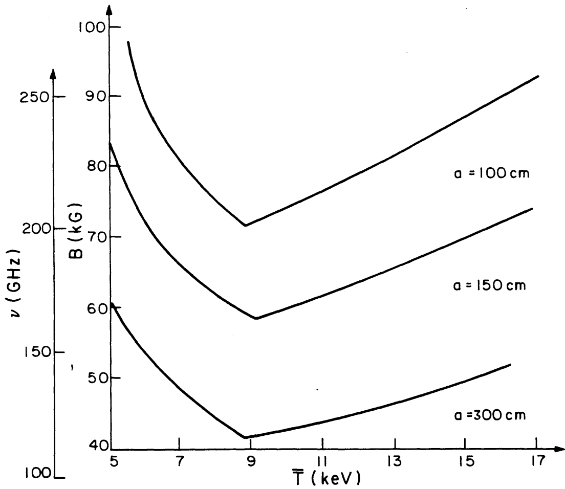
Figure 2.2 Minimum toroidal magnetic field and gyrotron frequency for a plasma with q=3 and an aspect ratio of 5. MS=2 and \beta_c=4\% .
