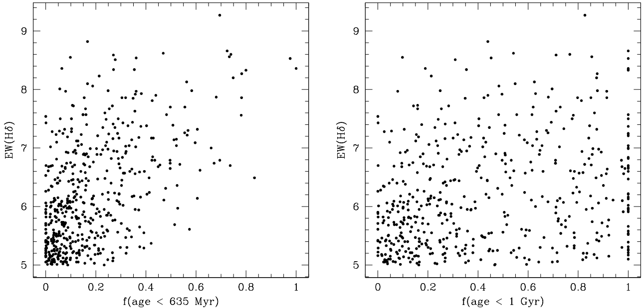
Figure 4. Rest-frame equivalent width of the H\delta absorption line from Goto (2007) with respect to the recent star formation fraction. The equivalent width is weakly correlated with the fraction of stellar mass younger than 635 Myr ( left ). But we do not find a correlation with the fraction of stellar mass younger than 1 Gyr ( right ) (e.g. Kauffmann et al. 2003; Martin et al. 2007; Falkenberg, Kotulla, & Fritze 2009a). The typical error of EW(H\delta) is about 1\text{\AA} .
