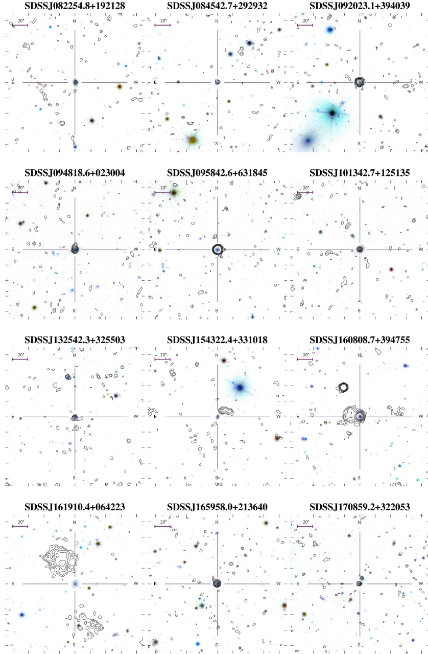
Figure 1. Radio-emitting post-starburst galaxies. Except for SDSSJ154322.4+331018, all galaxies are well matched to the coordinates of radio sources. SDSSJ160808.7+394755 and SDSSJ161910.4+064223 are suspected to have double radio lobes. Colour images are the SDSS gri cutout images of size 3'' \times 3'' , while the contour lines are from the FIRST images.
