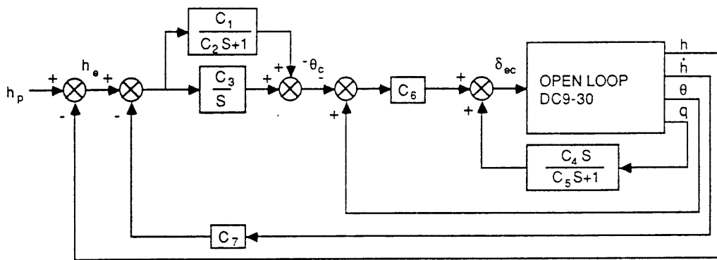
Figure 2-5 Block diagram of autopilot for McDonald Douglas DC9-30.
