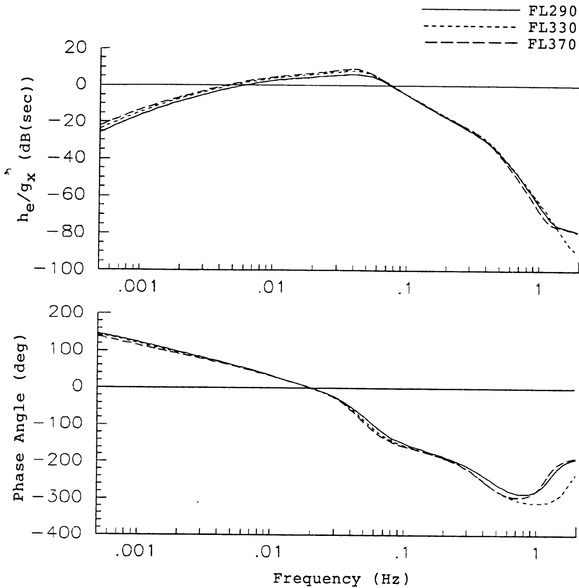
Figure 3-24 Altitude error sensitivity of 737-100 to horizontal gusts.
