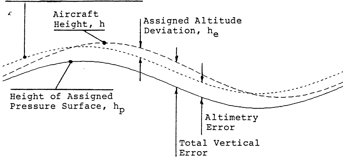
Figure 1-1 Altitude error components.
