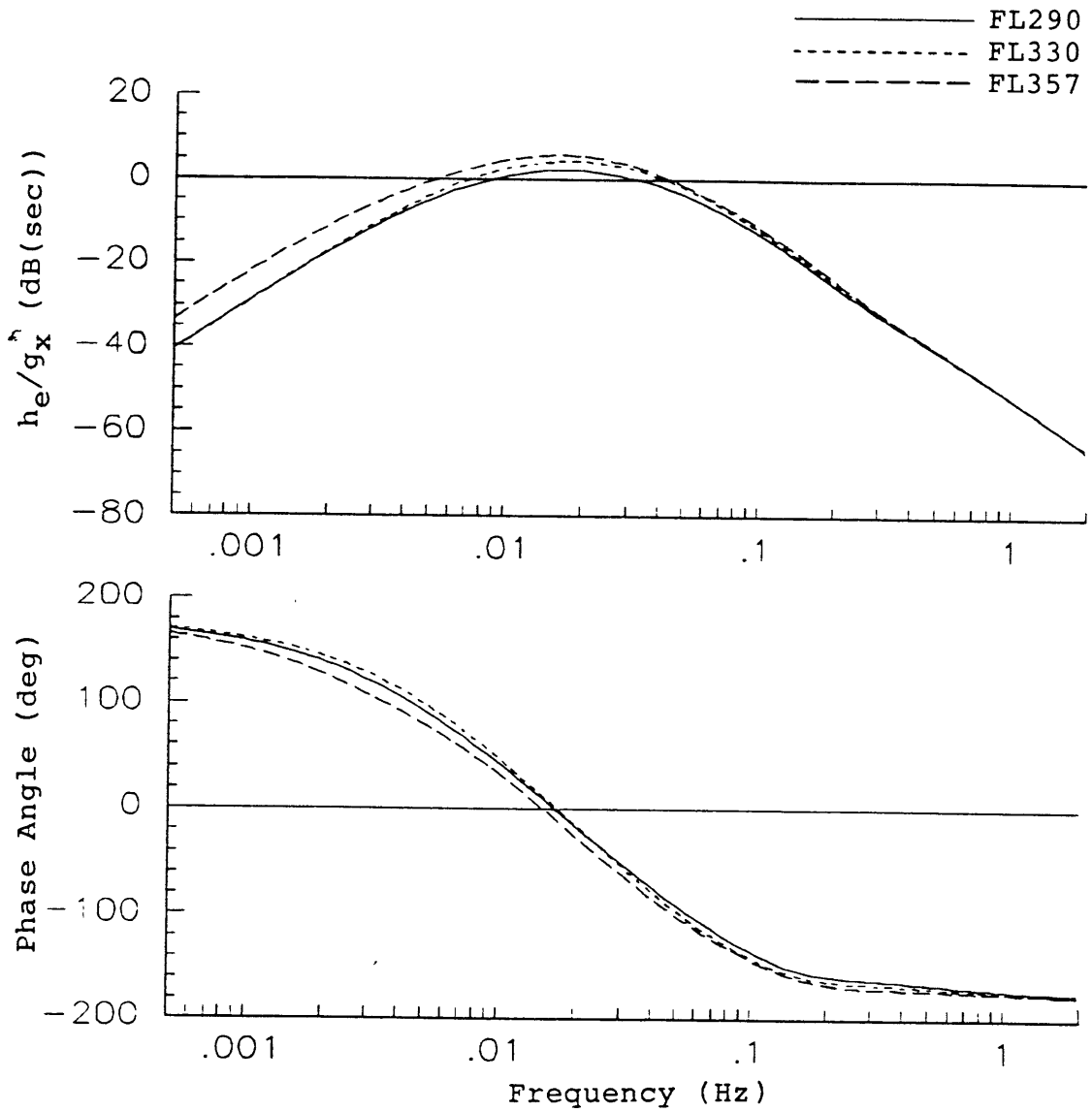
Figure 3-25 Altitude error sensitivity of DC9-30 to horizontal gusts.
