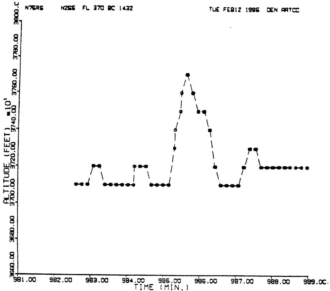
Figure 1-2 Mode C data showing an assigned altitude deviation of 700 feet.
