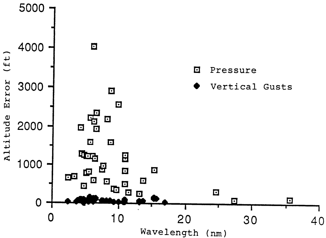
Figure 4-4 Predicted DC9 altitude errors resulting from observed pressure surface fluctuations and vertical gusts.
