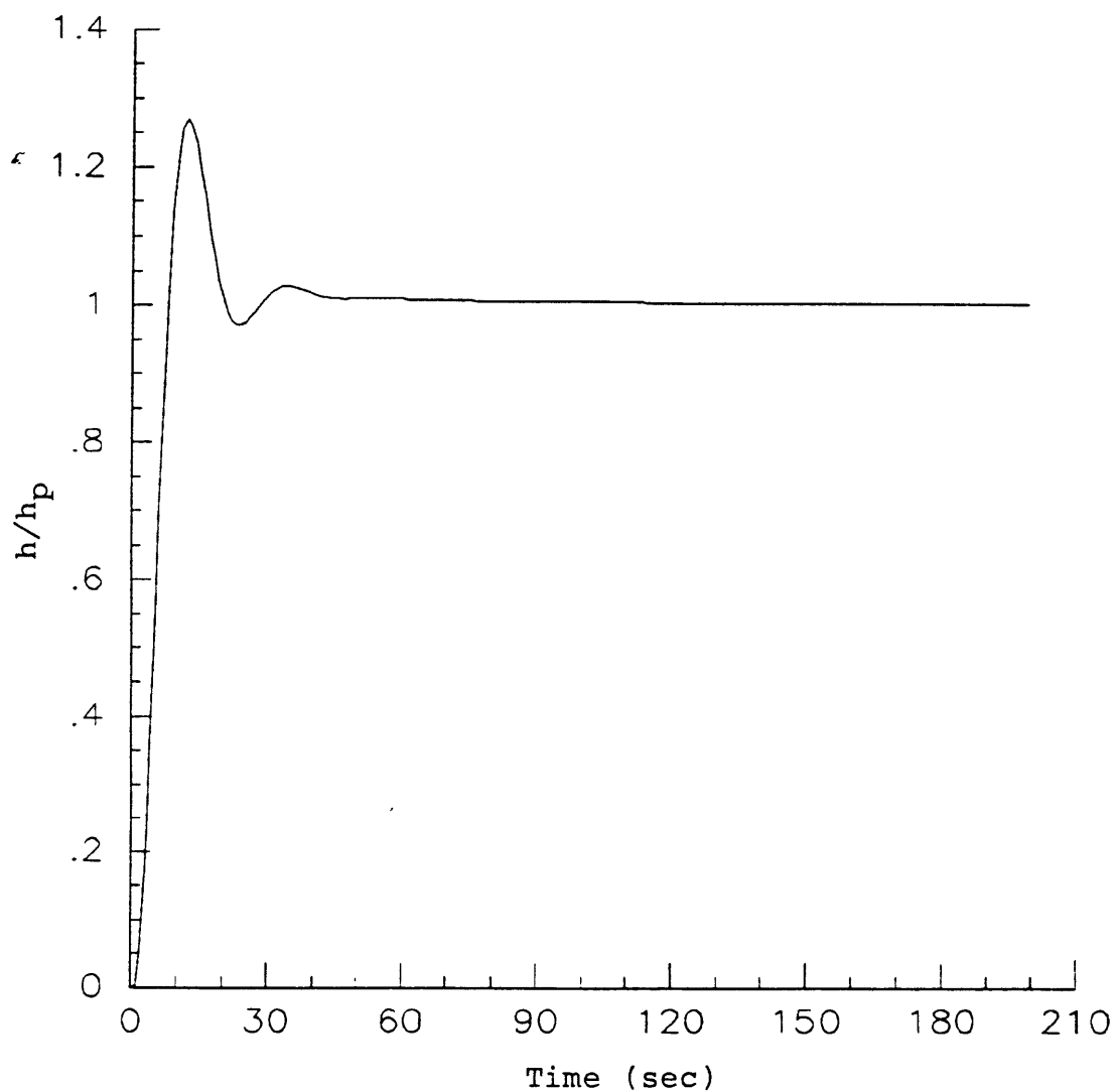
Figure 2-8 Typical response of aircraft height to step change in the height of the assigned pressure surface.
