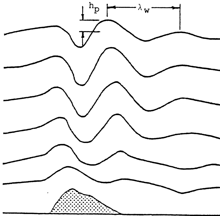
Figure 4-1 Mountain lee wave isobaric surfaces.
