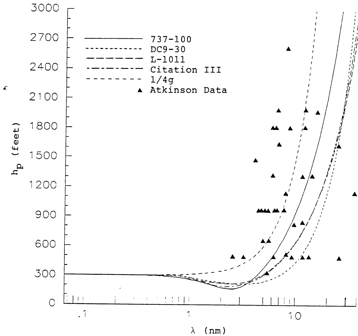
Figure 4-7 Tolerable pressure surface fluctuations for a specified altitude error limit of 300 feet.
