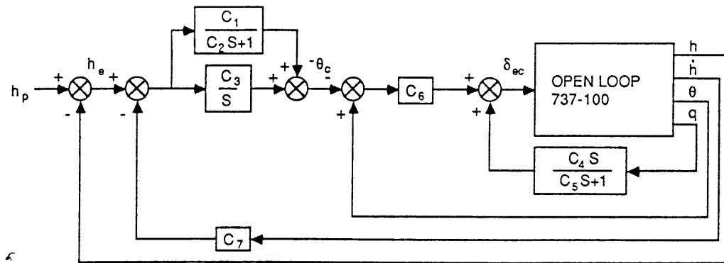
Figure 2-4 Block diagram of autopilot for Boeing 737-100.
