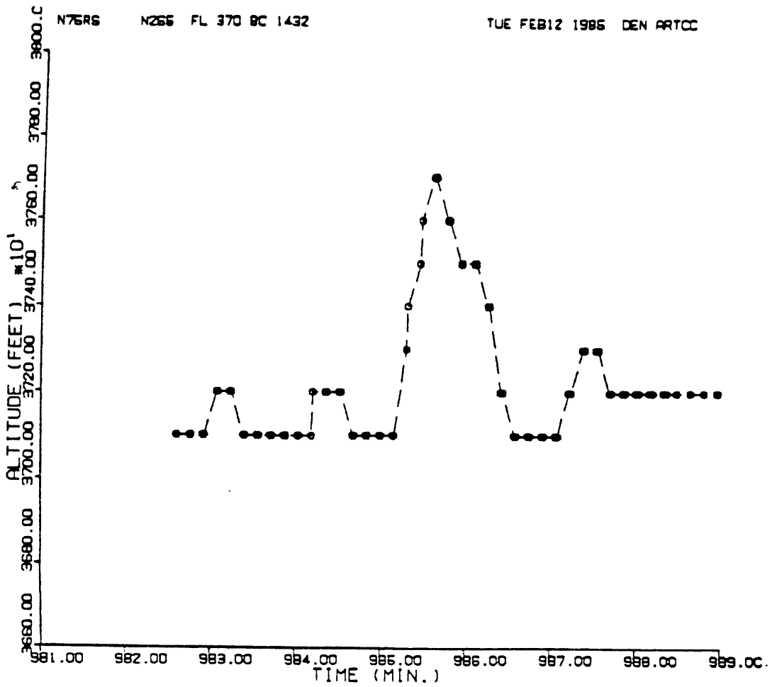
Figure 4-5 Mode C data from a Sabreliner flying in mountain waves.
