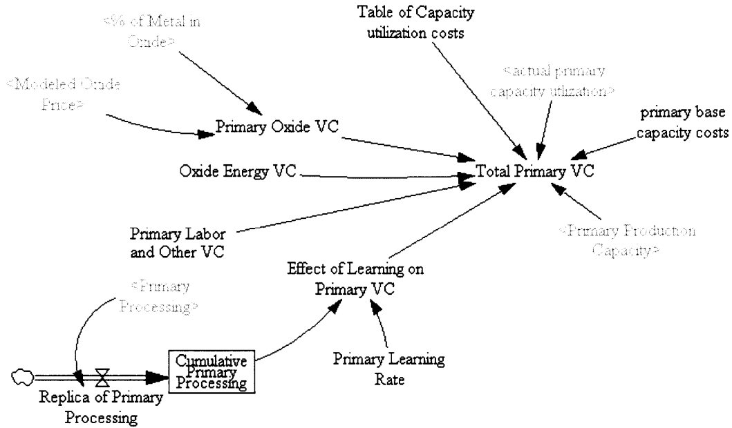
Figure 2-4: Model Structure for Costs
