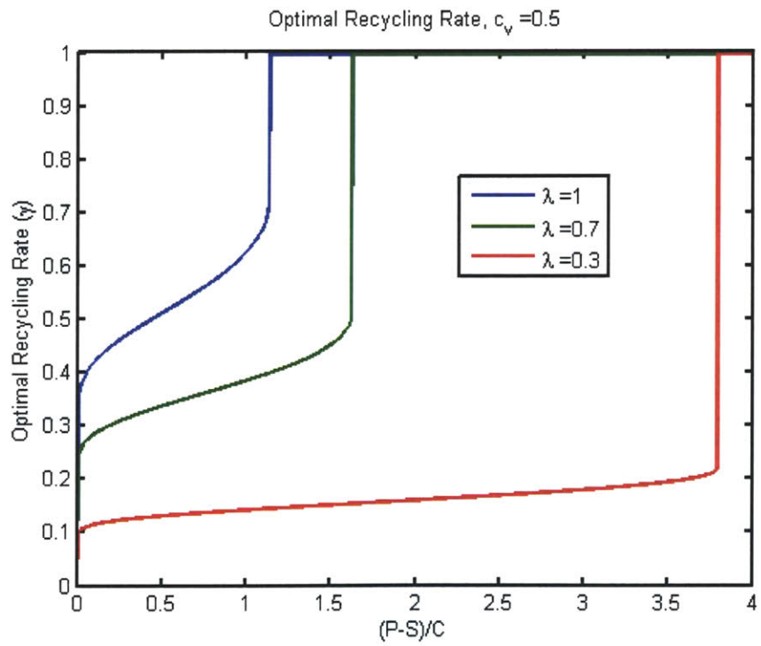
Figure 3-8: Optimal secondary use rate as a function of prices and costs. The y-axis variable \gamma is the optimal secondary use rate at a given primary price (P), secondary price (S), and cost of batch error (C).
