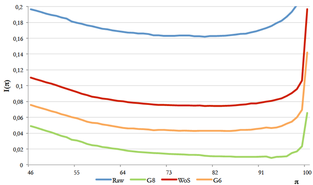
Figure 1. I(\pi) terms for percentiles in the interval [46, 100] before and after normalization using the G8 classification system for evaluation purposes
