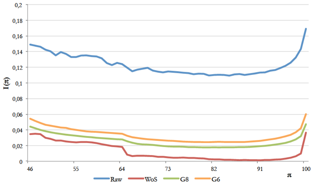
Figure 3. I(\pi) terms for percentiles in the interval [46, 100] before and after normalization using the WoS classification system for evaluation purposes
